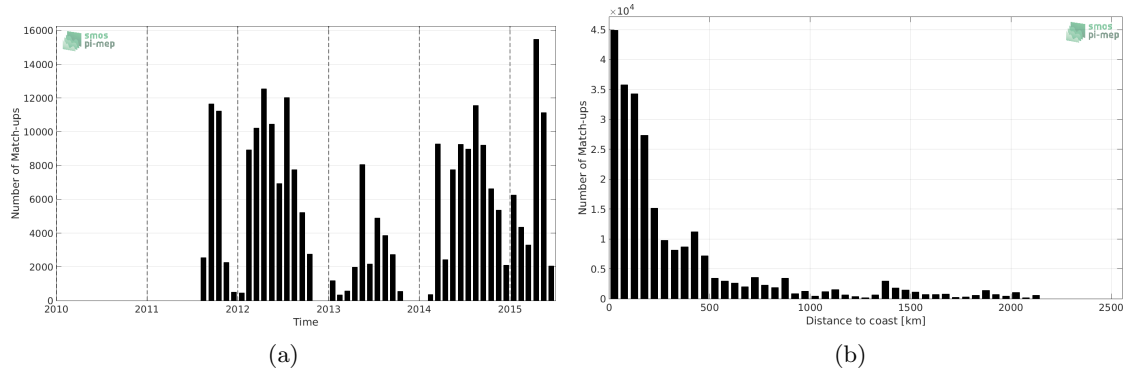
Figure 1: Number of match-ups between TSG-SAMOS and Aquarius-L2-JPL-V5 SSS as a function of time (a) and as function of the distance to coast (b) over the Pacific Ocean Pi-MEP region and for the full satellite product period.
