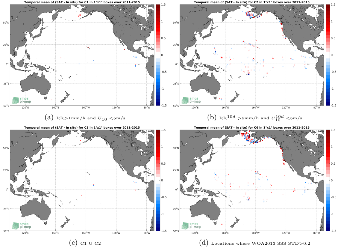
Figure 12: Temporal mean gridded over spatial boxes of size 1^\circ \times 1^\circ of \Delta SSS (Aquarius-L2-JPL-V5 - TSG-SAMOS) for 4 different subdatasets corresponding to: RR > 1\text{mm/h} and U_{10} < 5\text{m/s} (a), RR^{10d} > 5\text{mm/h} and U_{10}^{10d} < 5\text{m/s} (b), C1 U C2 (c), Locations where WOA2013 SSS STD > 0.2 (d).
