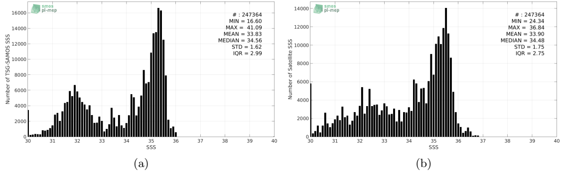
Figure 2: Histograms of SSS from TSG-SAMOS (a) and Aquarius-L2-JPL-V5 (b) considering all match-up pairs per bins of 0.1 over the Pacific Ocean Pi-MEP region and for the full satellite product period.
