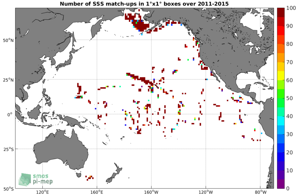
Figure 4: Number of SSS match-ups between TSG-SAMOS SSS and the Aquarius-L2-JPL-V5 SSS product for the Pacific Ocean Pi-MEP region over 1^\circ \times 1^\circ boxes and for the full satellite product period.
