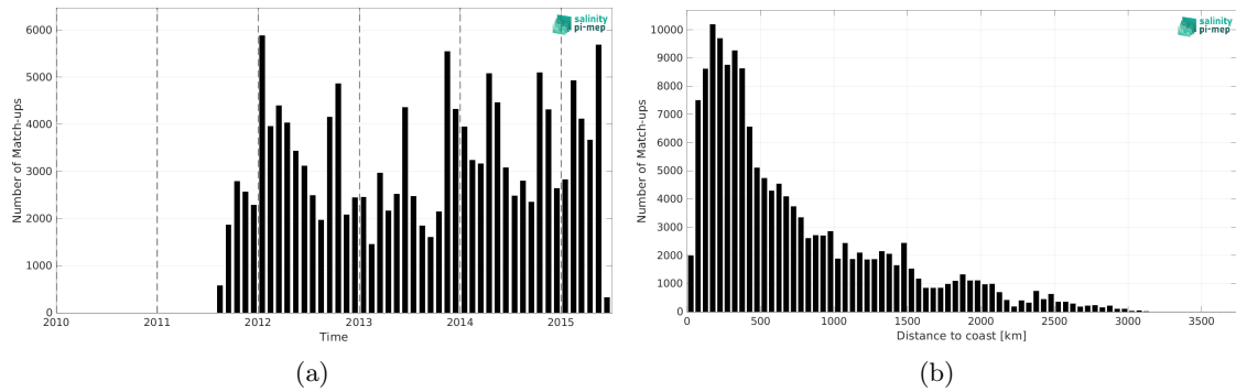
Figure 2: Number of match-ups between TSG (LEGOS-DM) and Aquarius SSS L2 CAP v5 (JPL) SSS as a function of time (a) and as function of the distance to coast (b) over the Pacific Ocean Pi-MEP region and for the full satellite product period.
