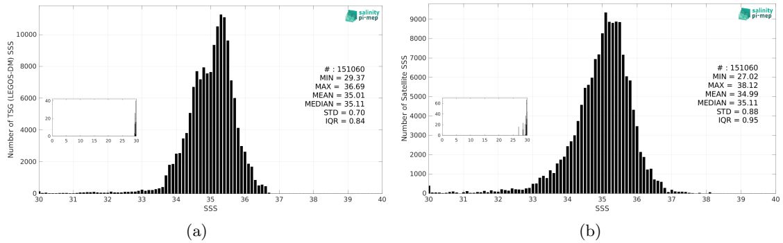
Figure 3: Histograms of SSS from TSG (LEGOS-DM) (a) and Aquarius SSS L2 CAP v5 (JPL) (b) considering all match-up pairs per bins of 0.1 over the Pacific Ocean Pi-MEP region and for the full satellite product period.
