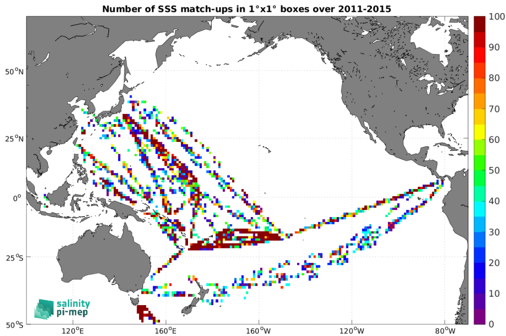
Figure 5: Number of SSS match-ups between TSG (LEGOS-DM) SSS and the Aquarius SSS L2 CAP v5 (JPL) SSS product for the Pacific Ocean Pi-MEP region over 1^\circ \times 1^\circ boxes and for the full satellite product period.
