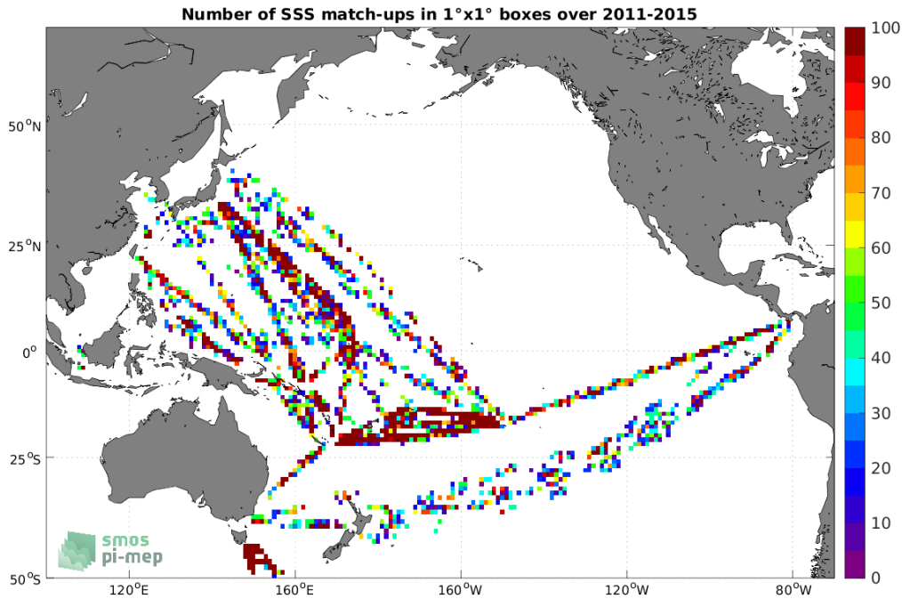
Figure 4: Number of SSS match-ups between TSG (LEGOS-DM) SSS and the Aquarius SSS L2 CAP v5 (JPL) SSS product for the Pacific Ocean Pi-MEP region over 1^\circ \times 1^\circ boxes and for the full satellite product period.
