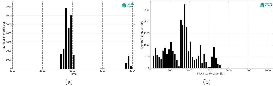
Figure 2: Number of match-ups between TSG (GOSUD-Sailing-ship) and Aquarius SSS L2 CAP v5 (JPL) SSS as a function of time (a) and as function of the distance to coast (b) over the Pacific Ocean Pi-MEP region and for the full satellite product period.
