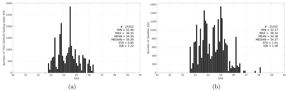
Figure 3: Histograms of SSS from TSG (GOSUD-Sailing-ship) (a) and Aquarius SSS L2 CAP v5 (JPL) (b) considering all match-up pairs per bins of 0.1 over the Pacific Ocean Pi-MEP region and for the full satellite product period.
