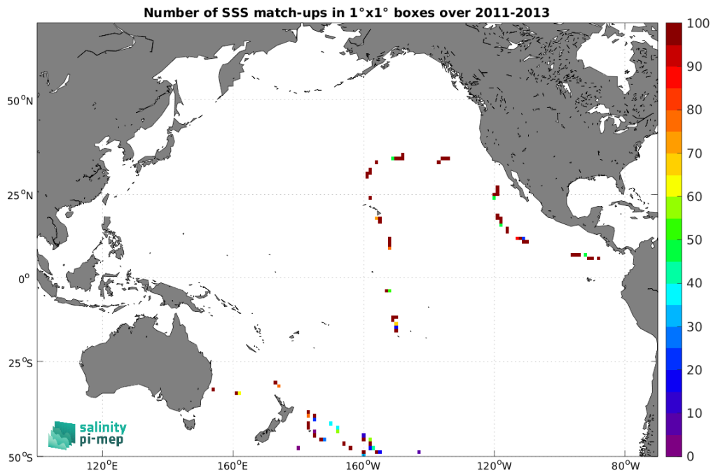
Figure 5: Number of SSS match-ups between TSG (GOSUD-Sailing-ship) SSS and the Aquarius SSS L2 CAP v5 (JPL) SSS product for the Pacific Ocean Pi-MEP region over 1^\circ \times 1^\circ boxes and for the full satellite product period.
