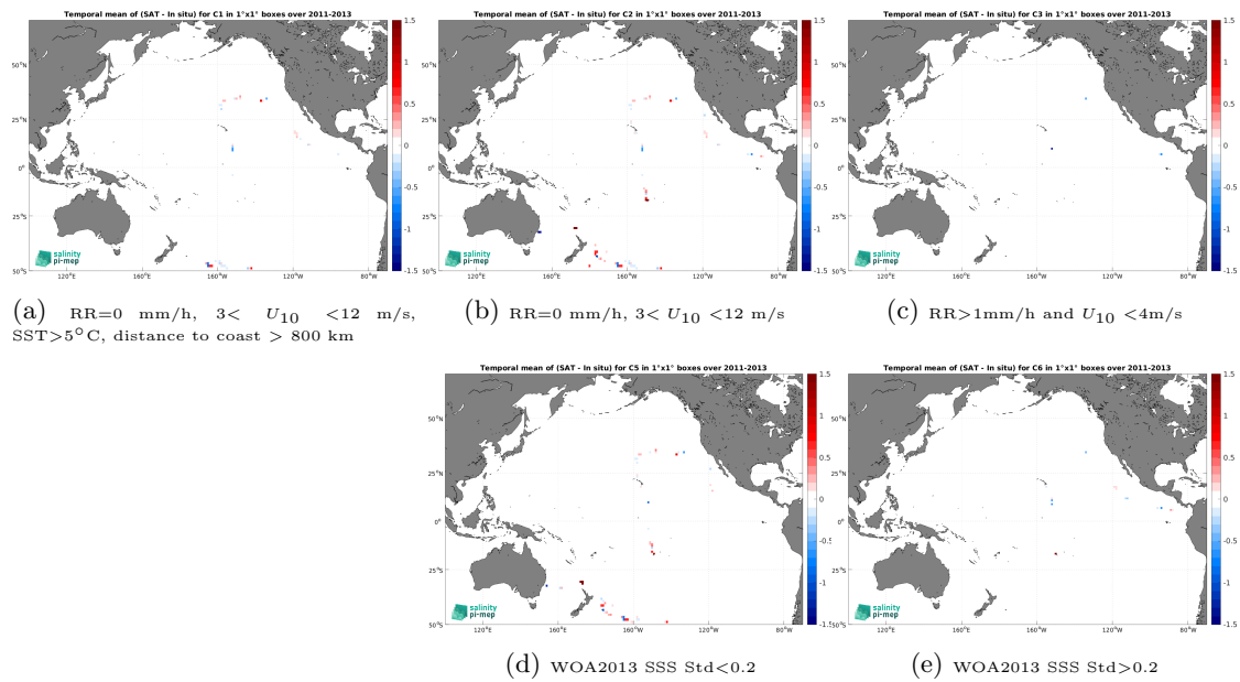
Figure 14: Temporal mean gridded over spatial boxes of size 1^\circ \times 1^\circ of \Delta SSS (Aquarius SSS L2 CAP v5 (JPL) - TSG (GOSUD-Sailing-ship)) for 5 different subdatasets corresponding to:RR=0 mm/h, 3 < U_{10} < 12 m/s, SST > 5^\circ\text{C} , distance to coast > 800 km (a), RR=0 mm/h, 3 < U_{10} < 12 m/s (b), RR > 1 mm/h and U_{10} < 4 m/s (c), WOA2013 SSS Std < 0.2 (d), WOA2013 SSS Std > 0.2 (e).
