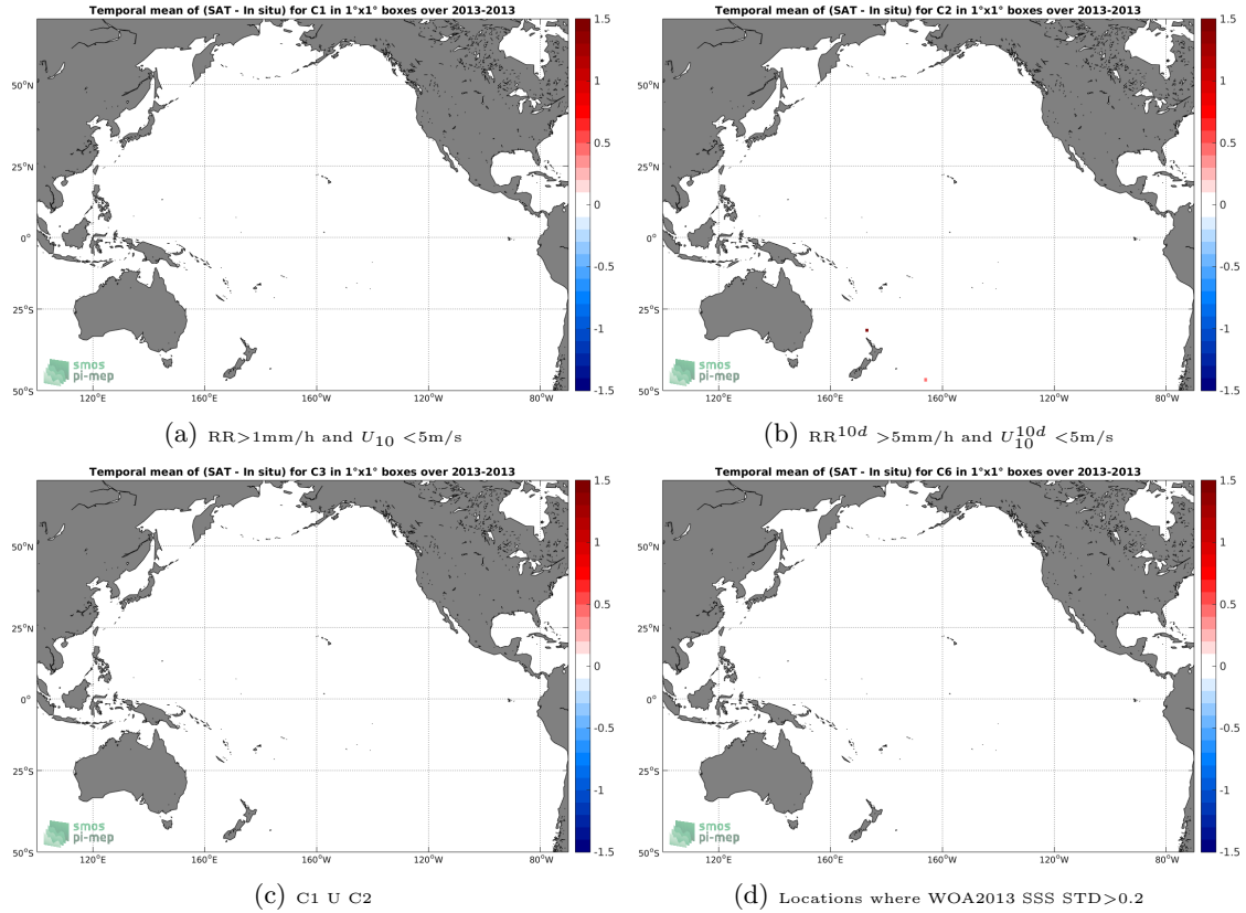
Figure 12: Temporal mean gridded over spatial boxes of size 1^\circ \times 1^\circ of \Delta SSS (Aquarius-L2-JPL-V5 - TSG-GOSUD-Sailing-ship) for 4 different subdatasets corresponding to: RR > 1\text{mm/h} and U_{10} < 5\text{m/s} (a), RR^{10d} > 5\text{mm/h} and U_{10}^{10d} < 5\text{m/s} (b), C1 U C2 (c), Locations where WOA2013 SSS STD > 0.2 (d).
