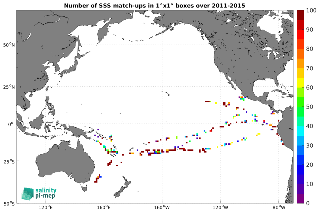
Figure 5: Number of SSS match-ups between TSG (GOSUD-Research-vessel) SSS and the Aquarius SSS L2 CAP v5 (JPL) SSS product for the Pacific Ocean Pi-MEP region over 1^\circ \times 1^\circ boxes and for the full satellite product period.
