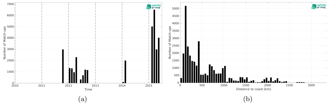
Figure 2: Number of match-ups between TSG (GOSUD-Research-vessel) and Aquarius SSS L2 CAP v5 (JPL) SSS as a function of time (a) and as function of the distance to coast (b) over the Pacific Ocean Pi-MEP region and for the full satellite product period.
