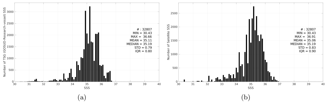
Figure 3: Histograms of SSS from TSG (GOSUD-Research-vessel) (a) and Aquarius SSS L2 CAP v5 (JPL) (b) considering all match-up pairs per bins of 0.1 over the Pacific Ocean Pi-MEP region and for the full satellite product period.
