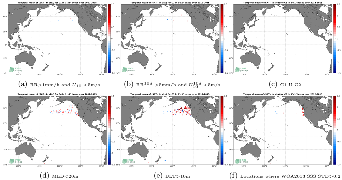
Figure 12: Temporal mean gridded over spatial boxes of size 1^\circ \times 1^\circ of \Delta\text{SSS} (Aquarius-L2-JPL-V5 - Sea mammals) for 6 different subdatasets corresponding to: RR > 1\text{mm/h} and U_{10} < 5\text{m/s} (a), RR^{10d} > 5\text{mm/h} and U_{10}^{10d} < 5\text{m/s} (b), C1 U C2 (c), MLD < 20\text{m} (d), BLT > 10\text{m} (e), Locations where WOA2013 SSS STD > 0.2 (f).
