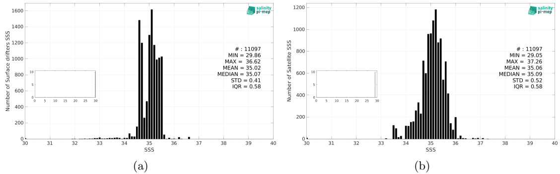
Figure 3: Histograms of SSS from Surface drifters (a) and Aquarius SSS L2 CAP v5 (JPL) (b) considering all match-up pairs per bins of 0.1 over the Pacific Ocean Pi-MEP region and for the full satellite product period.
