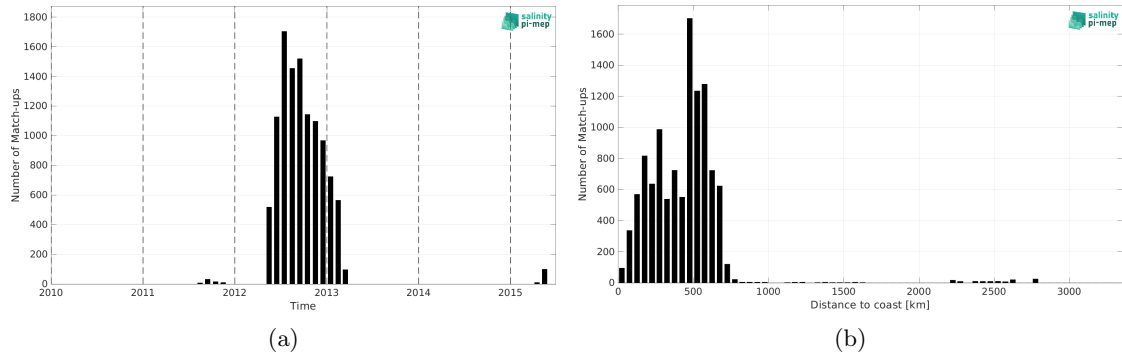
Figure 2: Number of match-ups between Surface drifters and Aquarius SSS L2 CAP v5 (JPL) SSS as a function of time (a) and as function of the distance to coast (b) over the Pacific Ocean Pi-MEP region and for the full satellite product period.
