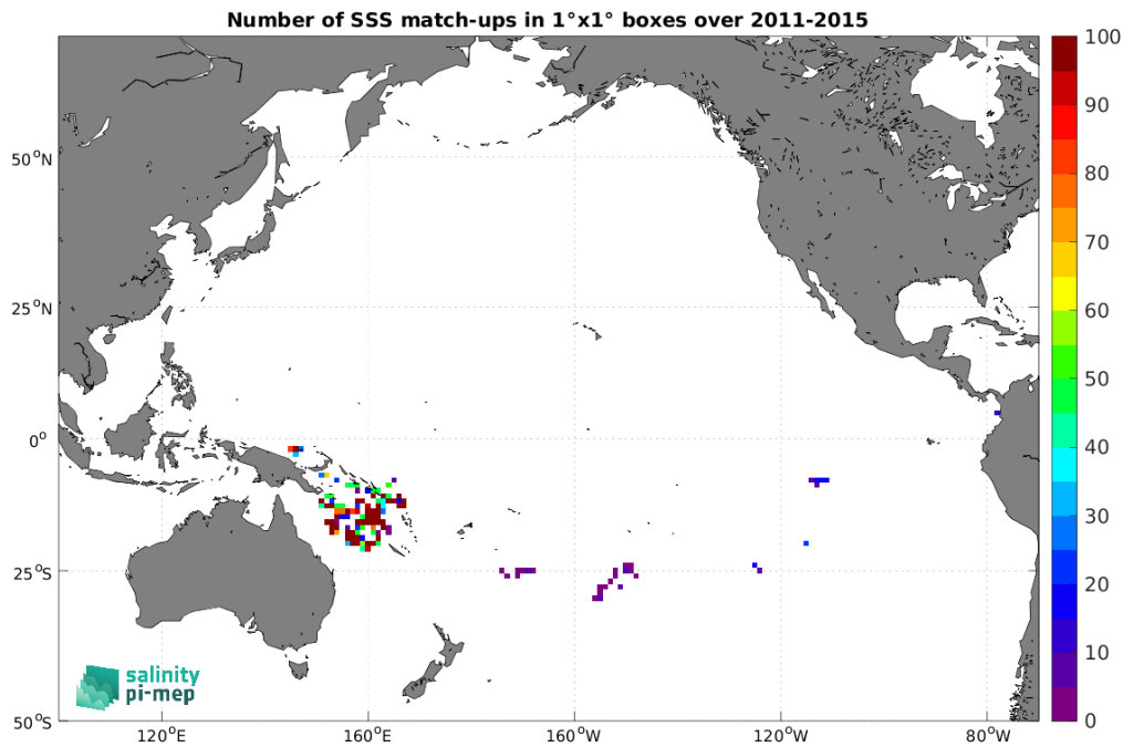
Figure 4: Number of SSS match-ups between Surface drifters SSS and the Aquarius SSS L2 CAP v5 (JPL) SSS product for the Pacific Ocean Pi-MEP region over 1^\circ \times 1^\circ boxes and for the full satellite product period.
