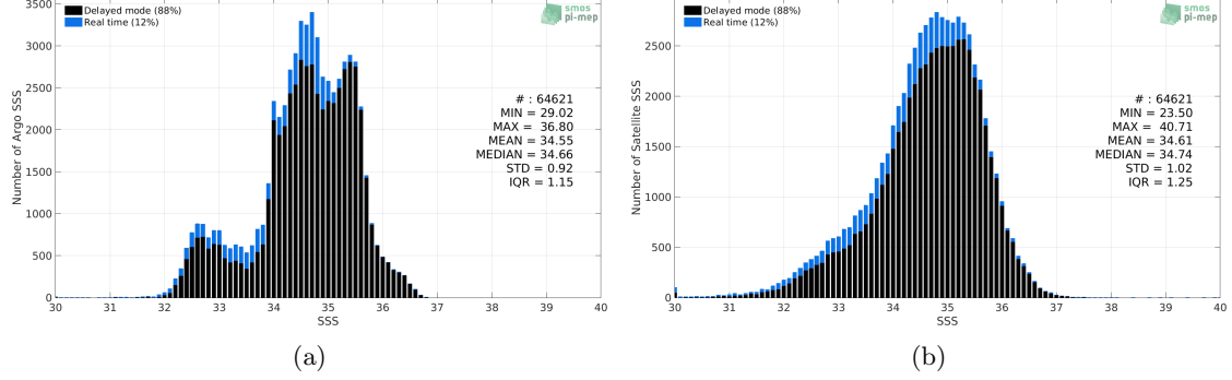
Figure 2: Histograms of SSS from Argo (a) and Aquarius SSS L2 CAP v5 (JPL) (b) considering all match-up pairs per bins of 0.1 over the Pacific Ocean Pi-MEP region and for the full satellite product period.
