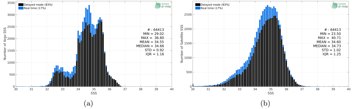
Figure 2: Histograms of SSS from Argo (a) and Aquarius-L2-JPL-V5 (b) considering all match-up pairs per bins of 0.1 over the Pacific Ocean Pi-MEP region and for the full satellite product period.
