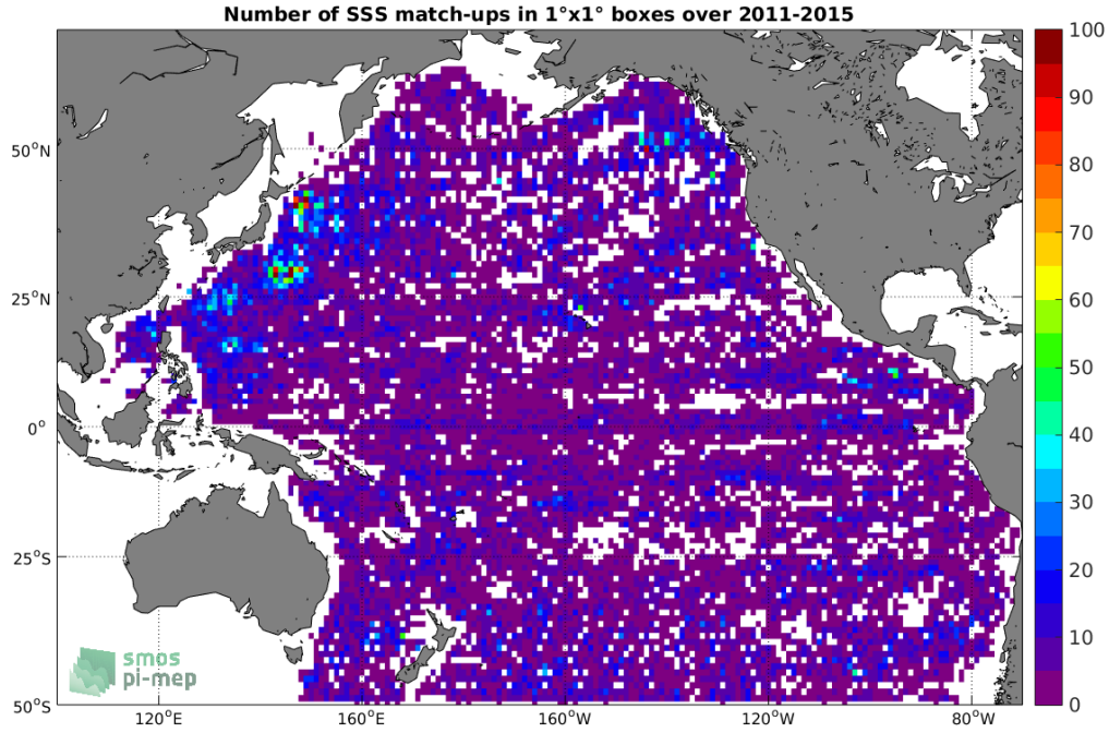
Figure 4: Number of SSS match-ups between Argo SSS and the Aquarius-L2-JPL-V5 SSS product for the Pacific Ocean Pi-MEP region over 1^\circ \times 1^\circ boxes and for the full satellite product period.
