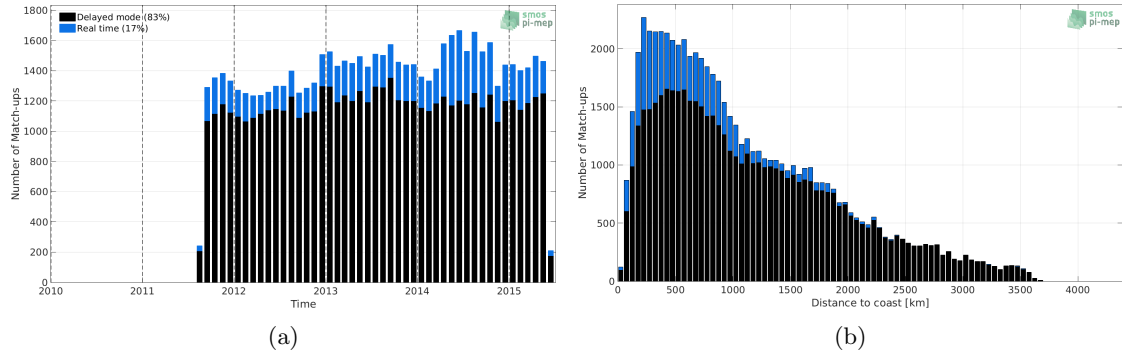
Figure 1: Number of match-ups between Argo and Aquarius-L2-JPL-V5 SSS as a function of time (a) and as function of the distance to coast (b) over the Pacific Ocean Pi-MEP region and for the full satellite product period.
