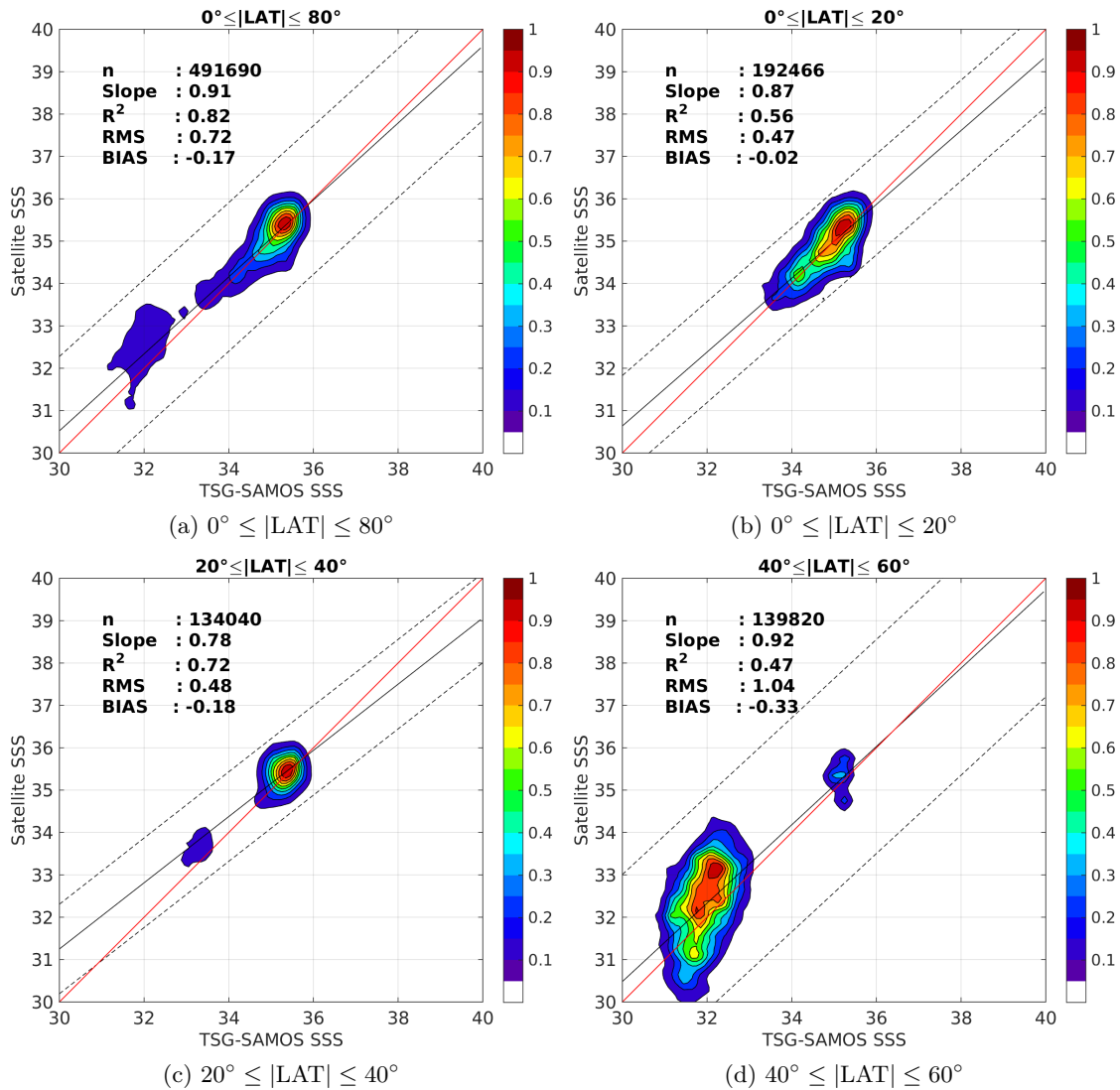
Figure 9: Contour maps of the concentration of AQUARIUS-L2-JPL-V4 SSS (y-axis) versus TSG-SAMOS SSS (x-axis) at match-up pairs for different latitude bands. For each plot, the red line shows x=y . The black thin and dashed lines indicate a linear fit through the data cloud and the \pm 95\% confidence levels, respectively. The number match-up pairs n , the slope and R^2 coefficient of the linear fit, the root mean square (RMS) and the mean bias between satellite and in situ data are indicated for each latitude band in each plots.
