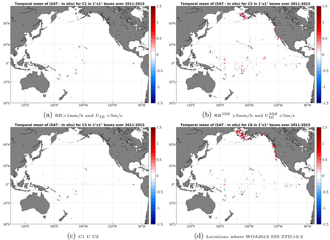
Figure 12: Temporal mean gridded over spatial boxes of size 1^\circ \times 1^\circ of \Delta SSS (AQUARIUS-L2-JPL-V4 - TSG-SAMOS) for 4 different subdatasets corresponding to: RR > 1\text{mm/h} and U_{10} < 5\text{m/s} (a), RR^{10d} > 5\text{mm/h} and U_{10}^{10d} < 5\text{m/s} (b), C1 U C2 (c), Locations where WOA2013 SSS STD > 0.2 (d).
