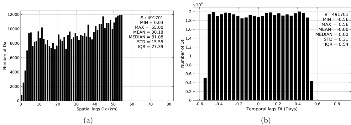
Figure 5: Histograms of the spatial (a) and temporal (b) lags between the time of the TSG-SAMOS measurements and the date of the corresponding AQUARIUS-L2-JPL-V4 SSS product.
