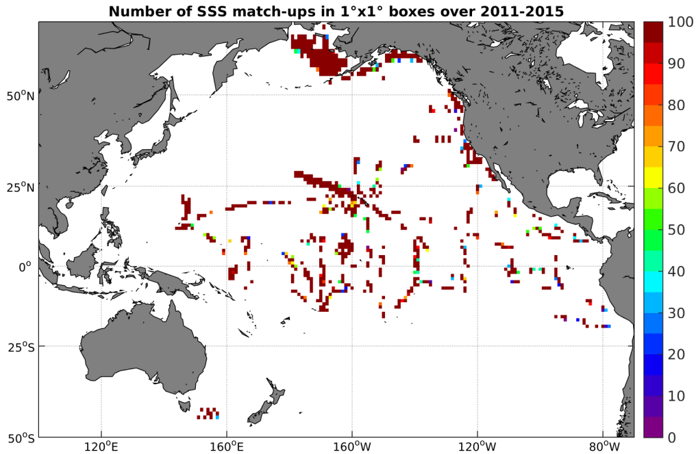
Figure 4: Number of SSS match-ups between TSG-SAMOS SSS and the AQUARIUS-L2-JPL-V4 SSS product for the Pacific Ocean Pi-MEP region over 1°x1° boxes and for the full satellite product period.
