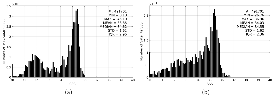
Figure 2: Histograms of SSS from TSG-SAMOS (a) and AQUARIUS-L2-JPL-V4 (b) considering all match-up pairs per bins of 0.1 over the Pacific Ocean Pi-MEP region and for the full satellite product period.
