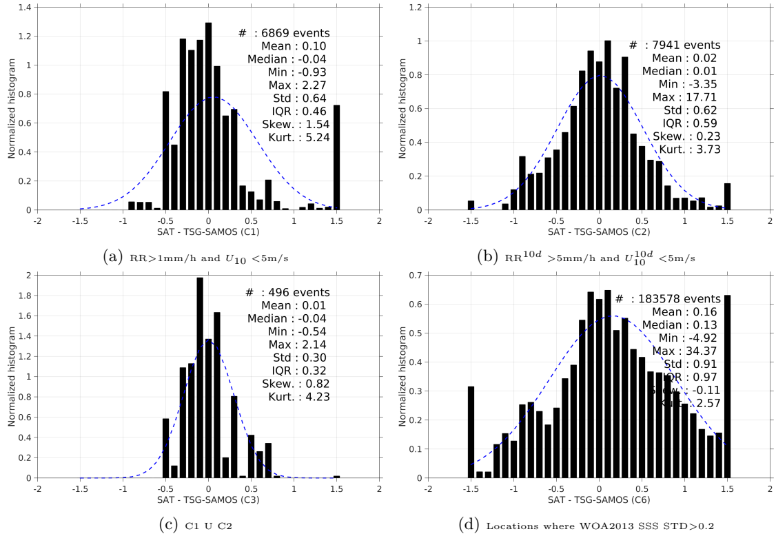
Figure 13: Normalized histogram of \Delta\text{SSS} (AQUARIUS-L2-JPL-V4 - TSG-SAMOS) for 6 different subdatasets corresponding to: RR > 1mm/h and U_{10} < 5\text{m/s} (a), RR^{10d} > 5\text{mm/h} and U_{10}^{10d} < 5\text{m/s} (b), C1 U C2 (c), Locations where WOA2013 SSS STD > 0.2 (d).
