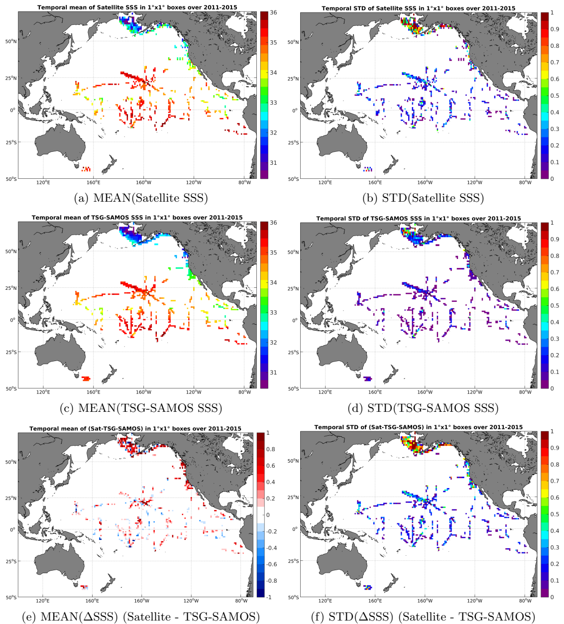
Figure 6: Temporal mean (left) and STD (right) of SSS from AQUARIUS-L2-JPL-V4 (top), TSG-SAMOS (middle), and of \Delta SSS (Satellite - TSG-SAMOS). Only match-up pairs are used to generate these maps.
