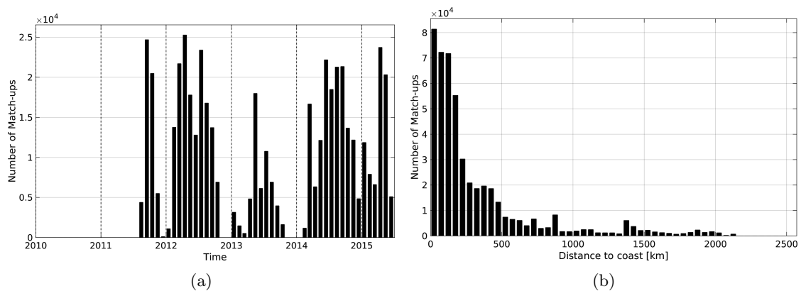
Figure 1: Number of match-ups between TSG-SAMOS and AQUARIUS-L2-JPL-V4 SSS as a function of time (a) and as function of the distance to coast (b) over the Pacific Ocean Pi-MEP region and for the full satellite product period.
