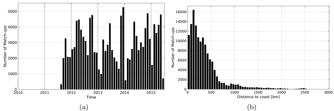
Figure 1: Number of match-ups between TSG-LEGOS-DM and AQUARIUS-L2-JPL-V4 SSS as a function of time (a) and as function of the distance to coast (b) over the Pacific Ocean Pi-MEP region and for the full satellite product period.
