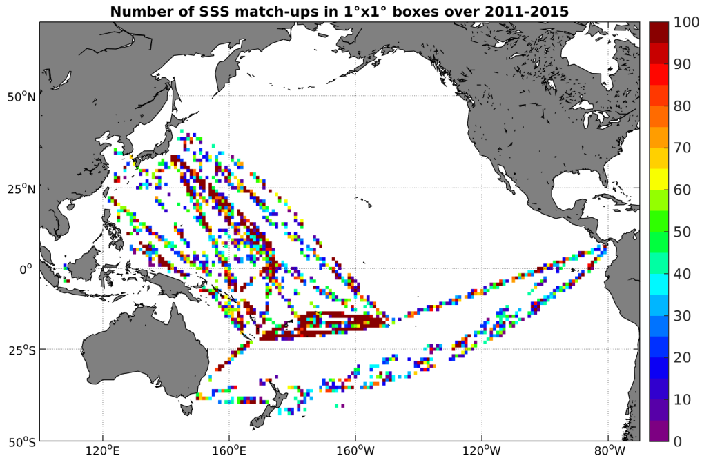
Figure 4: Number of SSS match-ups between TSG-LEGOS-DM SSS and the AQUARIUS-L2-JPL-V4 SSS product for the Pacific Ocean Pi-MEP region over 1^\circ \times 1^\circ boxes and for the full satellite product period.
