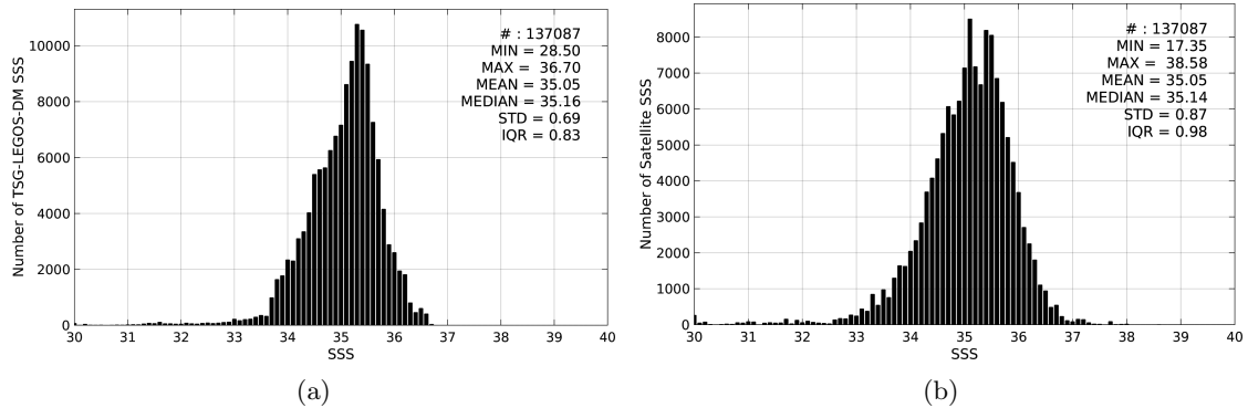
Figure 2: Histograms of SSS from TSG-LEGOS-DM (a) and AQUARIUS-L2-JPL-V4 (b) considering all match-up pairs per bins of 0.1 over the Pacific Ocean Pi-MEP region and for the full satellite product period.
