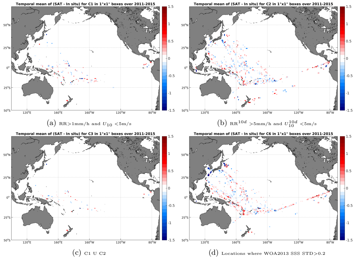
Figure 12: Temporal mean gridded over spatial boxes of size 1^\circ \times 1^\circ of \Delta SSS (AQUARIUS-L2-JPL-V4 - TSG-LEGOS-DM) for 4 different subdatasets corresponding to: RR > 1 mm/h and U_{10} < 5 m/s (a), RR 10d > 5 mm/h and U_{10}^{10d} < 5 m/s (b), C1 U C2 (c), Locations where WOA2013 SSS STD > 0.2 (d).
