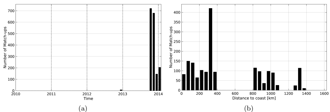
Figure 1: Number of match-ups between TSG-GOSUD-Sailing-ship and AQUARIUS-L2-JPL-V4 SSS as a function of time (a) and as function of the distance to coast (b) over the Pacific Ocean Pi-MEP region and for the full satellite product period.
