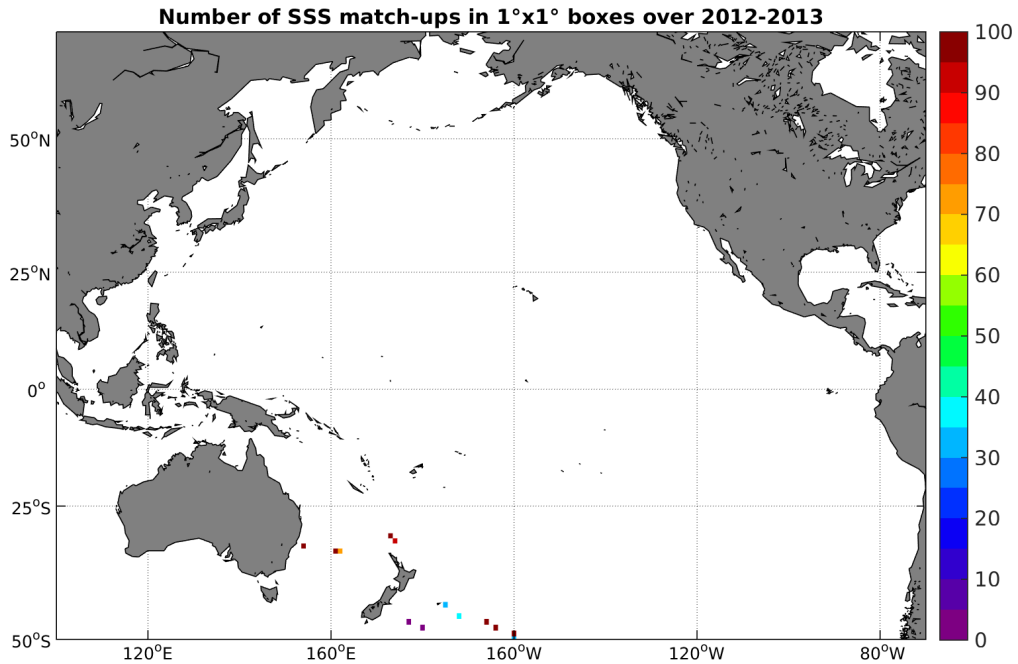
Figure 4: Number of SSS match-ups between TSG-GOSUD-Sailing-ship SSS and the AQUARIUS-L2-JPL-V4 SSS product for the Pacific Ocean Pi-MEP region over 1°x1° boxes and for the full satellite product period.
