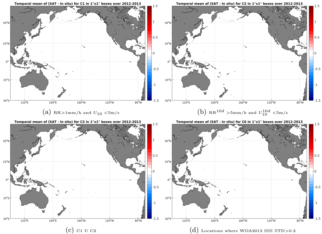
Figure 12: Temporal mean gridded over spatial boxes of size 1^\circ \times 1^\circ of \Delta SSS (AQUARIUS-L2-JPL-V4 - TSG-GOSUD-Sailing-ship) for 4 different subdatasets corresponding to: RR > 1\text{mm/h} and U_{10} < 5\text{m/s} (a), RR^{10d} > 5\text{mm/h} and U_{10}^{10d} < 5\text{m/s} (b), C1 U C2 (c), Locations where WOA2013 SSS STD > 0.2 (d).
