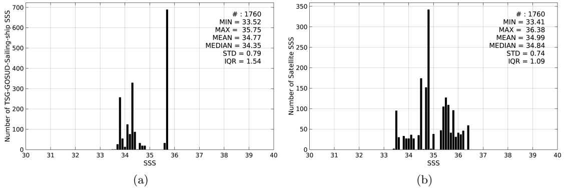
Figure 2: Histograms of SSS from TSG-GOSUD-Sailing-ship (a) and AQUARIUS-L2-JPL-V4 (b) considering all match-up pairs per bins of 0.1 over the Pacific Ocean Pi-MEP region and for the full satellite product period.
