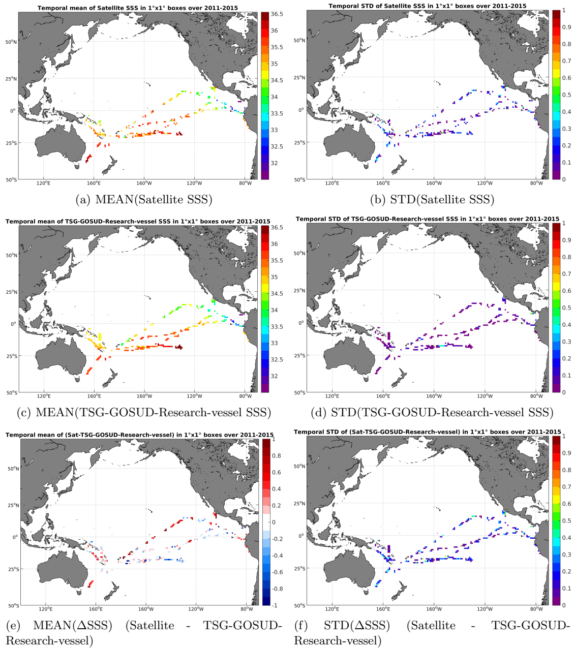
Figure 6: Temporal mean (left) and STD (right) of SSS from AQUARIUS-L2-JPL-V4 (top), TSG-GOSUD-Research-vessel (middle), and of \Delta SSS (Satellite - TSG-GOSUD-Research-vessel). Only match-up pairs are used to generate these maps.
