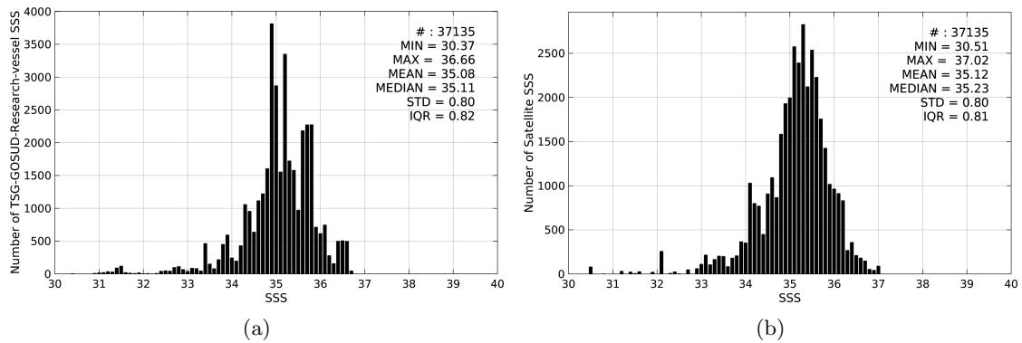
Figure 2: Histograms of SSS from TSG-GOSUD-Research-vessel (a) and AQUARIUS-L2-JPL-V4 (b) considering all match-up pairs per bins of 0.1 over the Pacific Ocean Pi-MEP region and for the full satellite product period.
