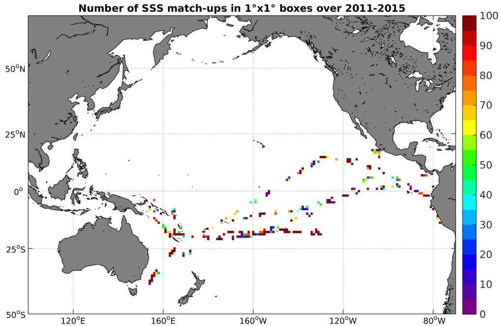
Figure 4: Number of SSS match-ups between TSG-GOSUD-Research-vessel SSS and the AQUARIUS-L2-JPL-V4 SSS product for the Pacific Ocean Pi-MEP region over 1^{\circ} \times 1^{\circ} boxes and for the full satellite product period.
