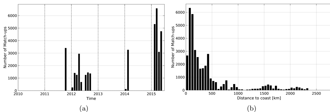
Figure 1: Number of match-ups between TSG-GOSUD-Research-vessel and AQUARIUS-L2-JPL-V4 SSS as a function of time (a) and as function of the distance to coast (b) over the Pacific Ocean Pi-MEP region and for the full satellite product period.
