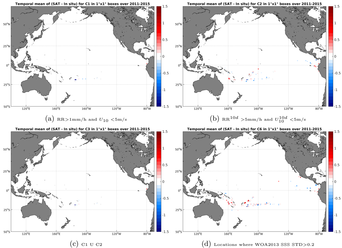
Figure 12: Temporal mean gridded over spatial boxes of size 1^\circ \times 1^\circ of \Delta SSS (AQUARIUS-L2-JPL-V4 - TSG-GOSUD-Research-vessel) for 4 different subdatasets corresponding to:RR > 1 mm/h and U_{10} < 5 m/s (a), RR 10d > 5 mm/h and U_{10}^{10d} < 5 m/s (b), C1 U C2 (c),Locations where WOA2013 SSS STD > 0.2 (d).
