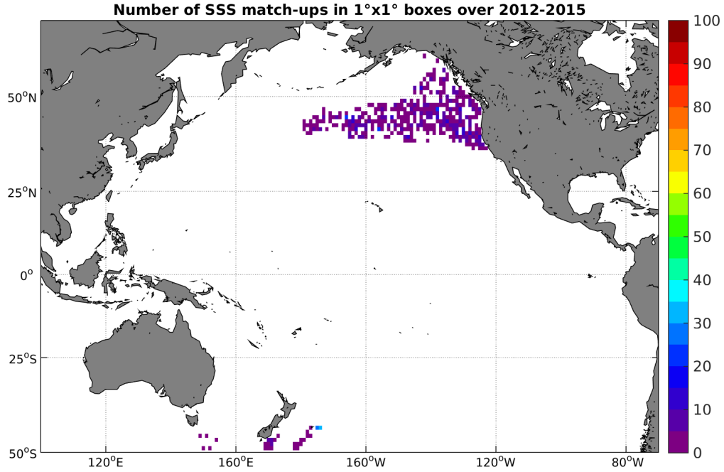
Figure 4: Number of SSS match-ups between Sea mammals SSS and the AQUARIUS-L2-JPL-V4 SSS product for the Pacific Ocean Pi-MEP region over 1^\circ \times 1^\circ boxes and for the full satellite product period.
