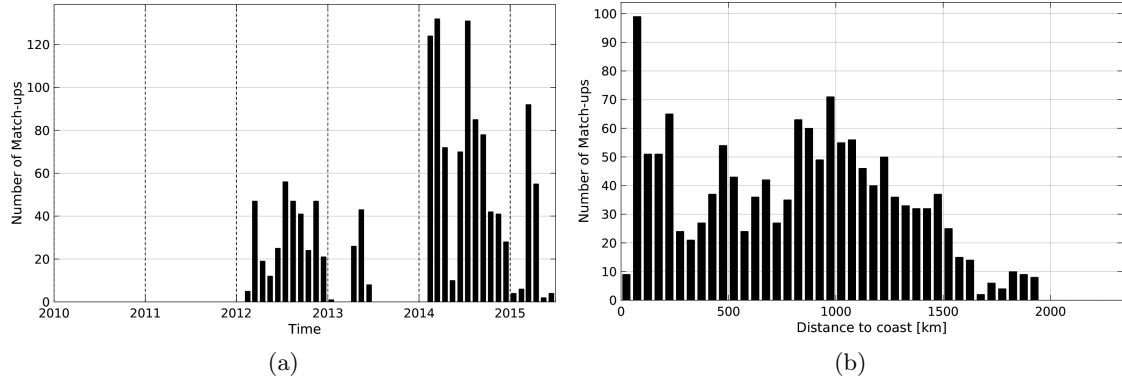
Figure 1: Number of match-ups between Sea mammals and AQUARIUS-L2-JPL-V4 SSS as a function of time (a) and as function of the distance to coast (b) over the Pacific Ocean Pi-MEP region and for the full satellite product period.
