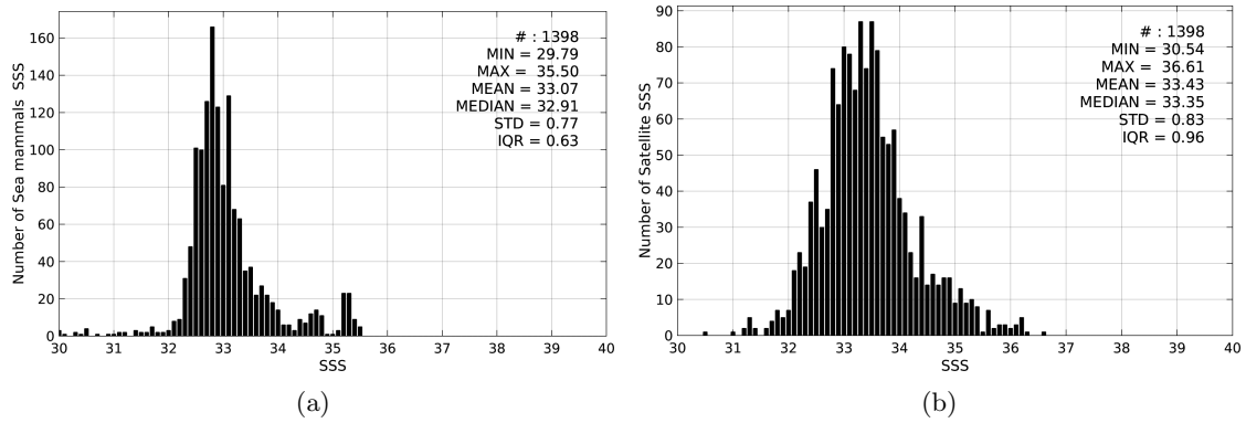
Figure 2: Histograms of SSS from Sea mammals (a) and AQUARIUS-L2-JPL-V4 (b) considering all match-up pairs per bins of 0.1 over the Pacific Ocean Pi-MEP region and for the full satellite product period.
