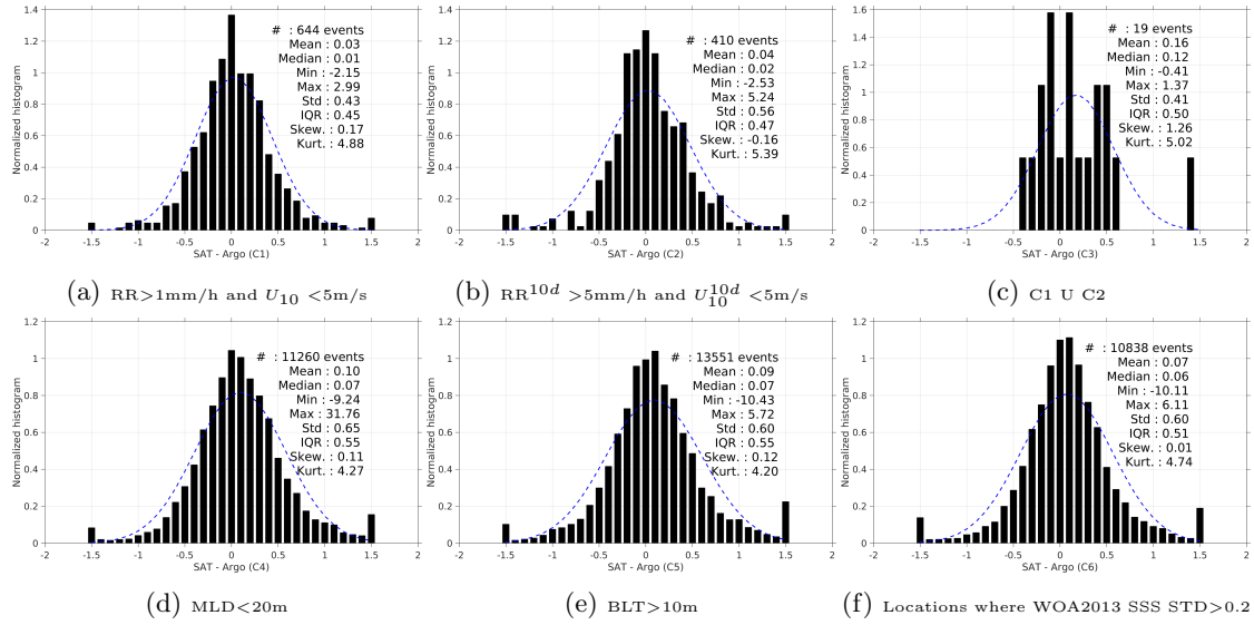
Figure 13: Normalized histogram of \Delta SSS (AQUARIUS-L2-JPL-V4 - Argo) for 6 different sub-datasets corresponding to: RR>1mm/h and U_{10} <5m/s (a), RR 10d >5mm/h and U_{10}^{10d} <5m/s (b), C1 U C2 (c),MLD<20m (d),BLT>10m (e),Locations where WOA2013 SSS STD>0.2 (f).
