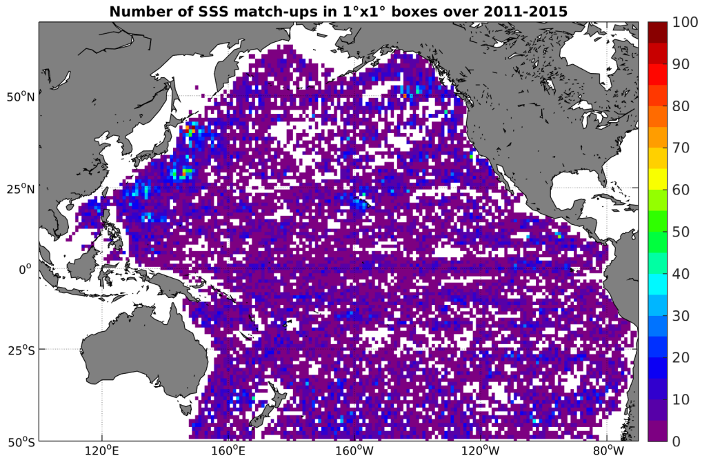
Figure 4: Number of SSS match-ups between Argo SSS and the AQUARIUS-L2-JPL-V4 SSS product for the Pacific Ocean Pi-MEP region over 1°x1° boxes and for the full satellite product period.
