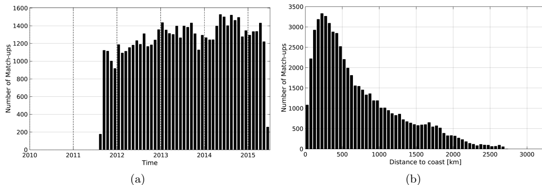
Figure 1: Number of match-ups between Argo and AQUARIUS-L2-JPL-V4 SSS as a function of time (a) and as function of the distance to coast (b) over the Pacific Ocean Pi-MEP region and for the full satellite product period.
