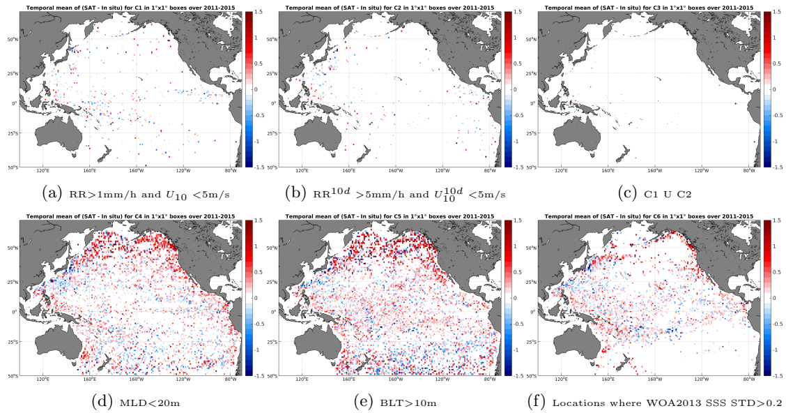
Figure 12: Temporal mean gridded over spatial boxes of size 1^\circ \times 1^\circ of \Delta\text{SSS} (AQUARIUS-L2-JPL-V4 - Argo) for 6 different subdatasets corresponding to: RR > 1\text{mm/h} and U_{10} < 5\text{m/s} (a), RR^{10d} > 5\text{mm/h} and U_{10}^{10d} < 5\text{m/s} (b), C1 U C2 (c), MLD < 20\text{m} (d), BLT > 10\text{m} (e), Locations where WOA2013 SSS STD > 0.2 (f).
