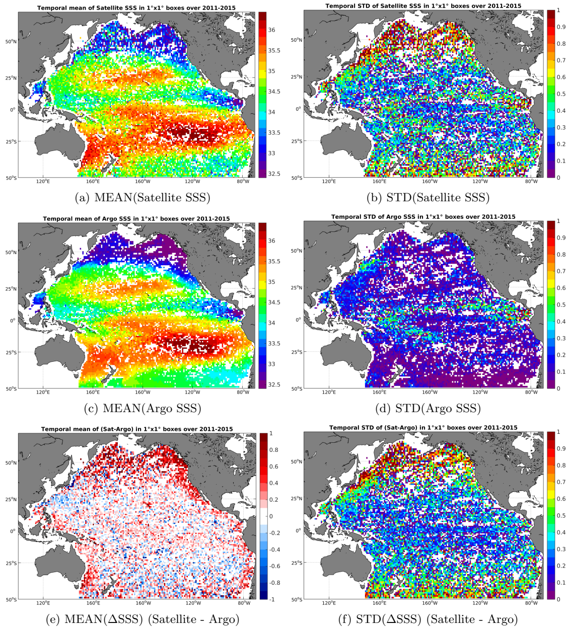
Figure 6: Temporal mean (left) and STD (right) of SSS from AQUARIUS-L2-JPL-V4 (top), Argo (middle), and of \Delta SSS (Satellite - Argo). Only match-up pairs are used to generate these maps.
