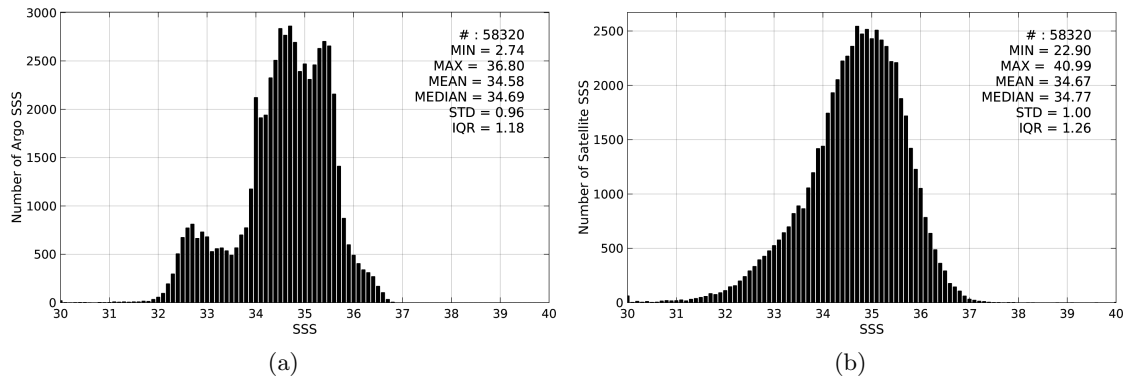
Figure 2: Histograms of SSS from Argo (a) and AQUARIUS-L2-JPL-V4 (b) considering all match-up pairs per bins of 0.1 over the Pacific Ocean Pi-MEP region and for the full satellite product period.
