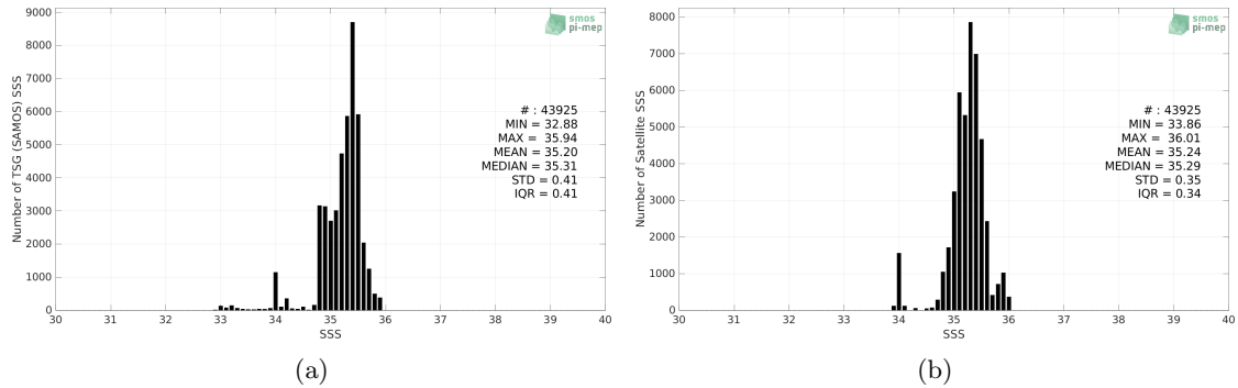
Figure 2: Histograms of SSS from TSG (SAMOS) (a) and SMOS and SMAP SSS L4 OI v1 - 7 Days (LOPS) (b) considering all match-up pairs per bins of 0.1 over the OTT zone Pi-MEP region and for the full satellite product period.
