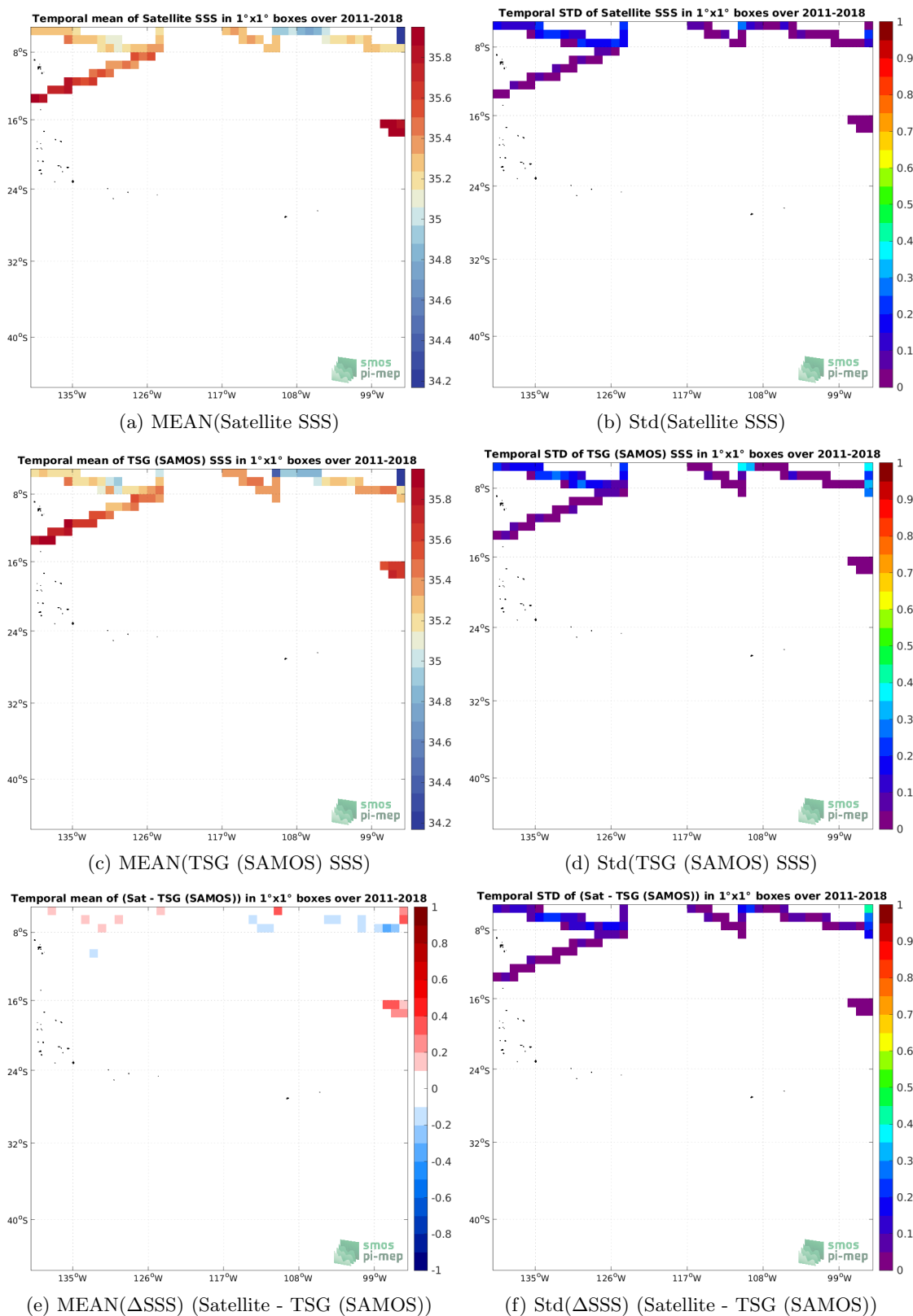
Figure 6: Temporal mean (left) and Std (right) of SSS from SMOS and SMAP SSS L4 OI v1 - 7 Days (LOPS) (top), TSG (SAMOS) (middle), and of \Delta SSS (Satellite - TSG (SAMOS)). Only match-up pairs are used to generate these maps.
