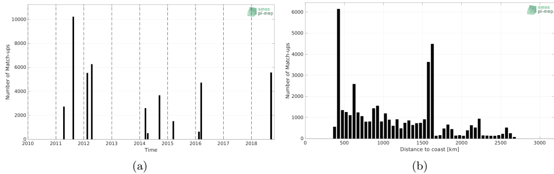
Figure 1: Number of match-ups between TSG (SAMOS) and SMOS and SMAP SSS L4 OI v1 - 7 Days (LOPS) SSS as a function of time (a) and as function of the distance to coast (b) over the OTT zone Pi-MEP region and for the full satellite product period.
