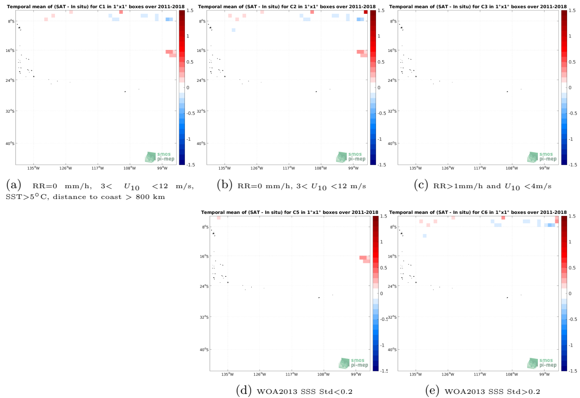
Figure 12: Temporal mean gridded over spatial boxes of size 1^\circ \times 1^\circ of \Delta SSS (SMOS and SMAP SSS L4 OI v1 - 7 Days (LOPS) - TSG (SAMOS)) for 5 different subdatasets corresponding to: RR=0 mm/h, 3 < U_{10} < 12 m/s, SST > 5^\circ C , distance to coast > 800 km (a), RR=0 mm/h, 3 < U_{10} < 12 m/s (b), RR > 1 mm/h and U_{10} < 4 m/s (c), WOA2013 SSS Std < 0.2 (d), WOA2013 SSS Std > 0.2 (e).
