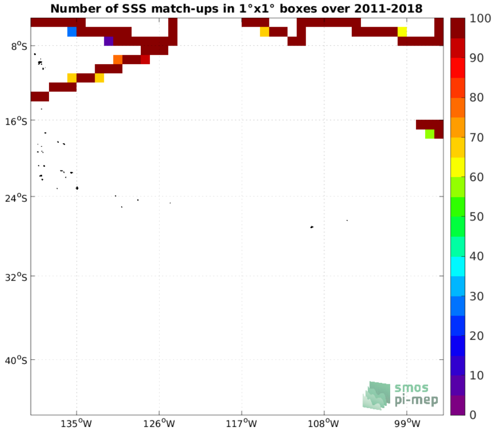
Figure 4: Number of SSS match-ups between TSG (SAMOS) SSS and the SMOS and SMAP SSS L4 OI v1 - 7 Days (LOPS) SSS product for the OTT zone Pi-MEP region over 1^\circ \times 1^\circ boxes and for the full satellite product period.
