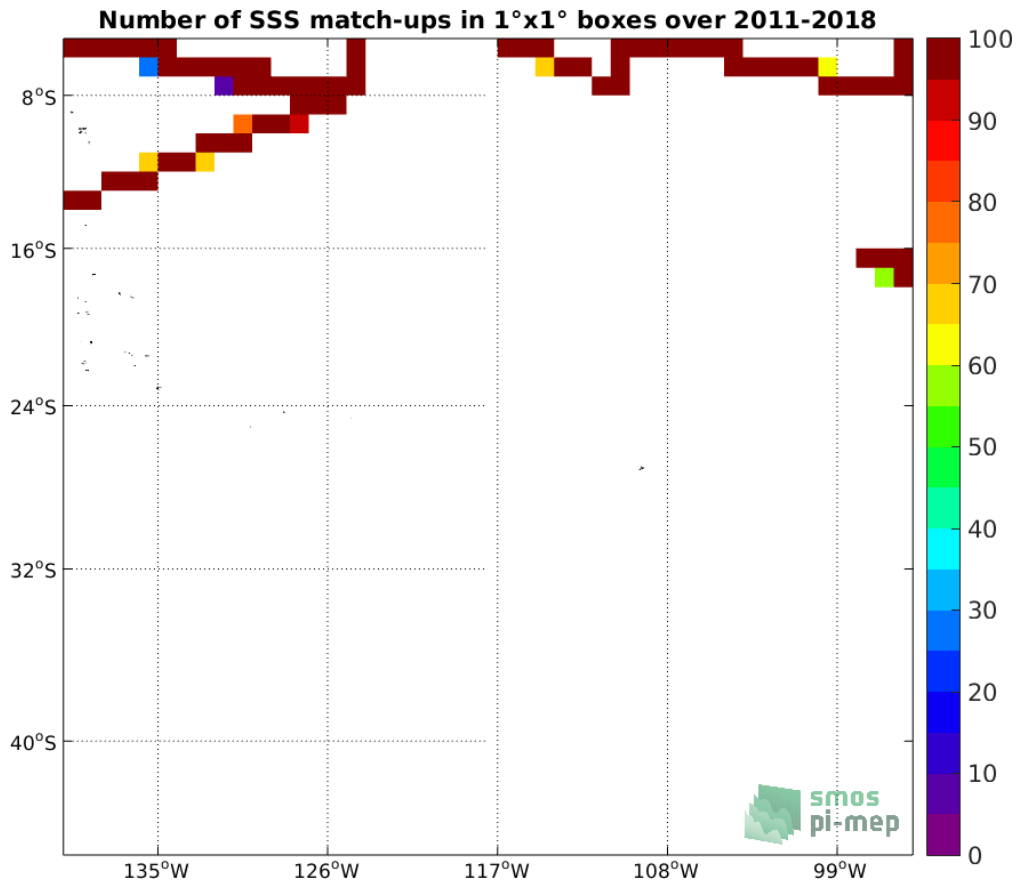
Figure 4: Number of SSS match-ups between TSG (SAMOS) SSS and the SMOS and SMAP SSS L4 OI v1 - 7 Days (LOPS) SSS product for the OTT zone Pi-MEP region over 1°x1° boxes and for the full satellite product period.
