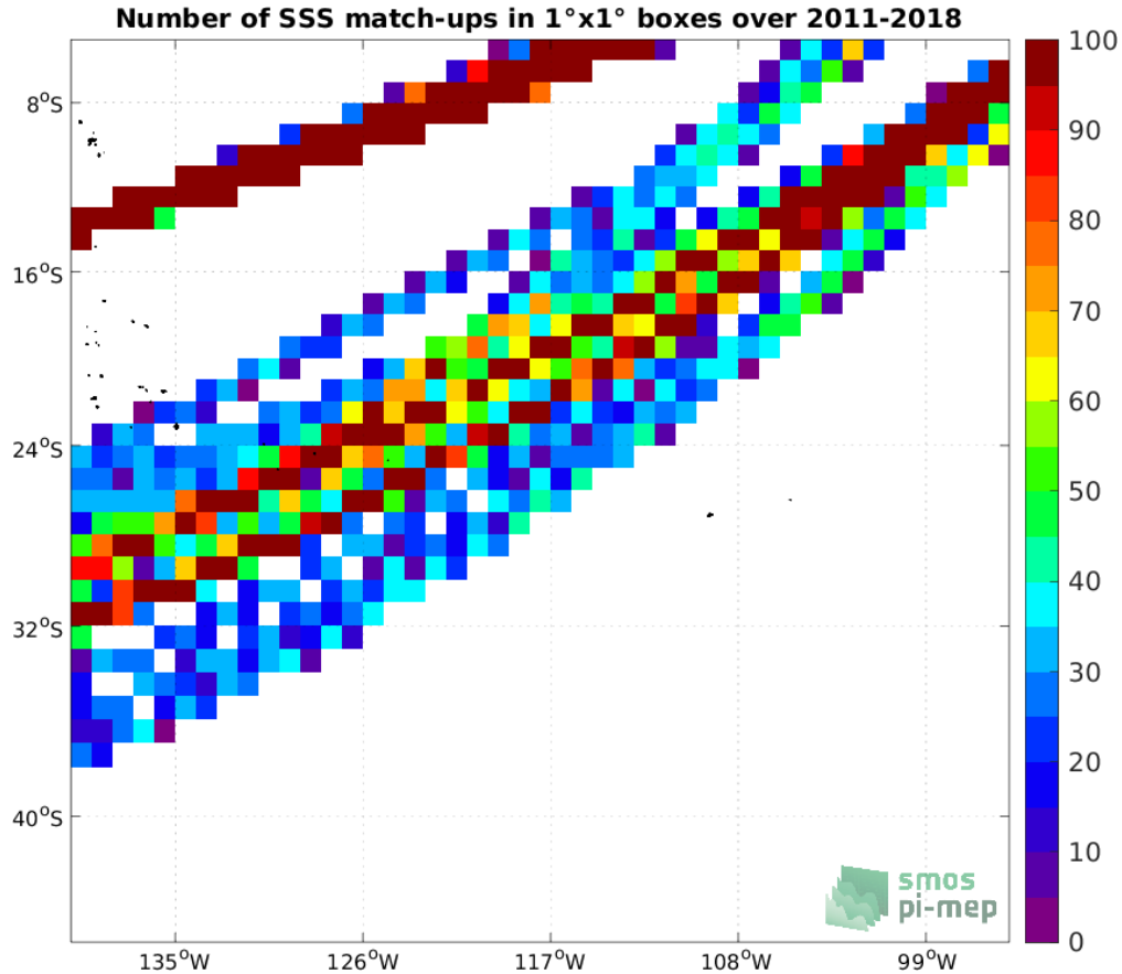
Figure 4: Number of SSS match-ups between TSG (LEGOS-DM) SSS and the SMOS and SMAP SSS L4 OI v1 - 7 Days (LOPS) SSS product for the OTT zone Pi-MEP region over 1^\circ \times 1^\circ boxes and for the full satellite product period.
