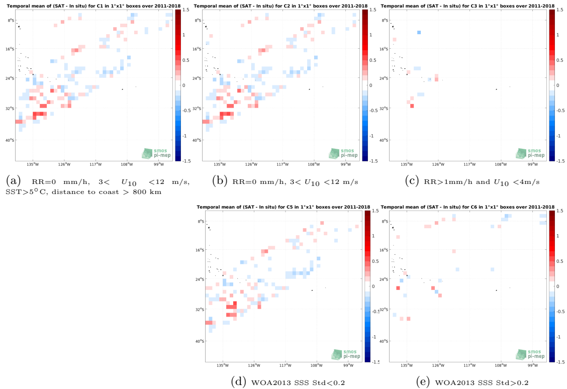
Figure 12: Temporal mean gridded over spatial boxes of size 1^{\circ}\times 1^{\circ} of \Delta\text{SSS} (SMOS and SMAP SSS L4 OI v1 - 7 Days (LOPS) - TSG (LEGOS-DM)) for 5 different subdatasets corresponding to:RR=0 mm/h, 3 < U_{10} < 12 m/s, SST >5^{\circ}\text{C} , distance to coast > 800 km (a), RR=0 mm/h, 3 < U_{10} < 12 m/s (b), RR >1 mm/h and U_{10} < 4 m/s (c), WOA2013 SSS Std <0.2 (d), WOA2013 SSS Std >0.2 (e).
