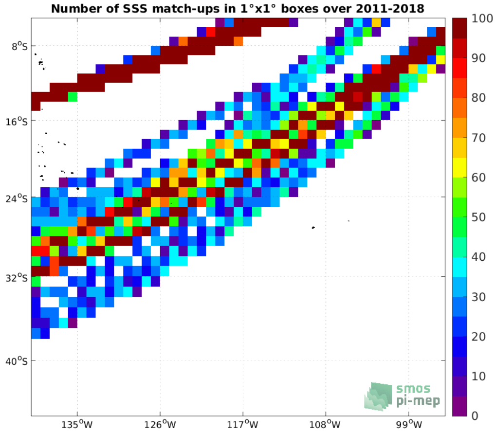
Figure 4: Number of SSS match-ups between TSG (LEGOS-DM) SSS and the SMOS and SMAP SSS L4 OI v1 - 7 Days (LOPS) SSS product for the OTT zone Pi-MEP region over 1°x1° boxes and for the full satellite product period.
