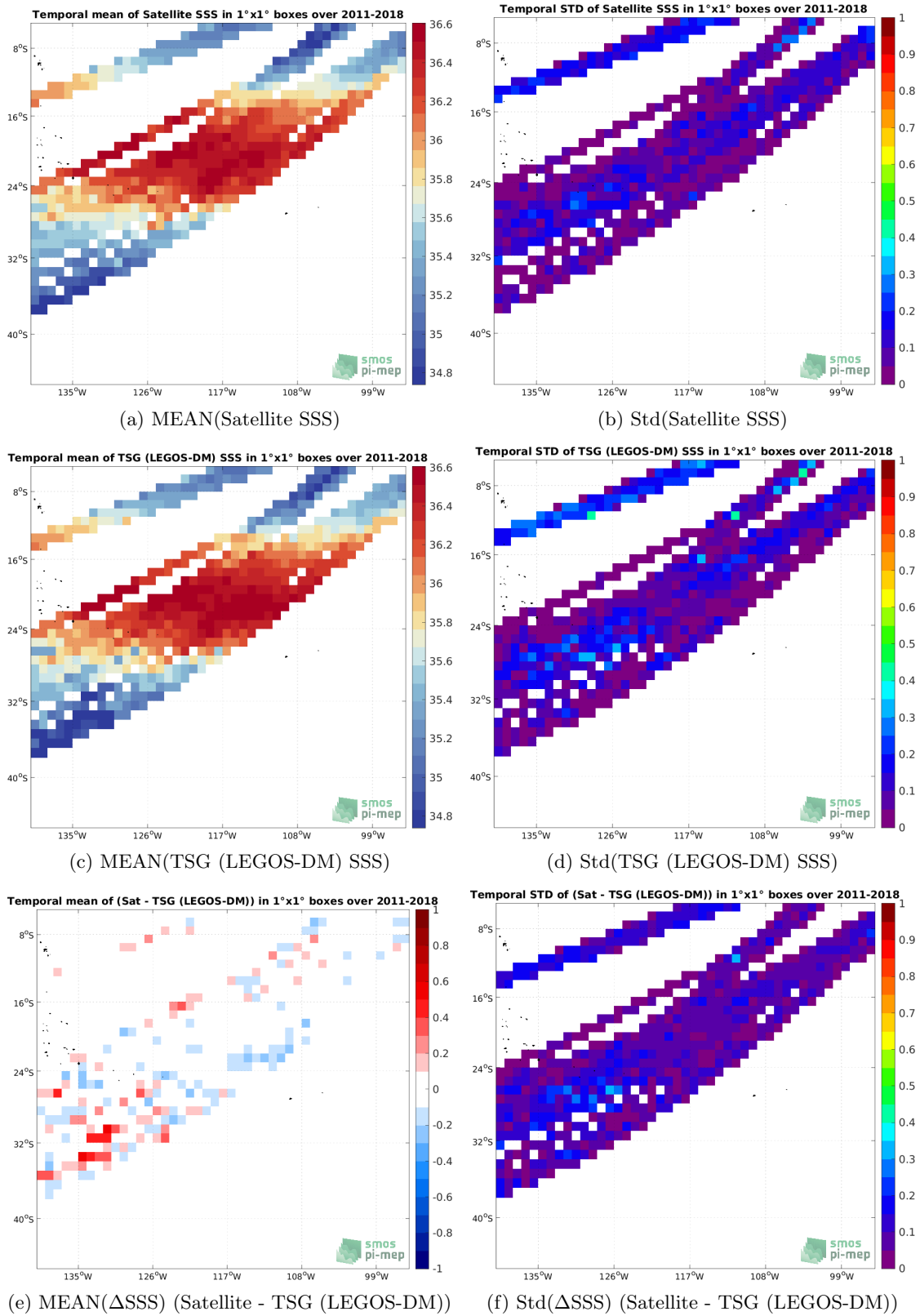
Figure 6: Temporal mean (left) and Std (right) of SSS from SMOS and SMAP SSS L4 OI v1 - 7 Days (LOPS) (top), TSG (LEGOS-DM) (middle), and of \Delta SSS (Satellite - TSG (LEGOS-DM)). Only match-up pairs are used to generate these maps.
