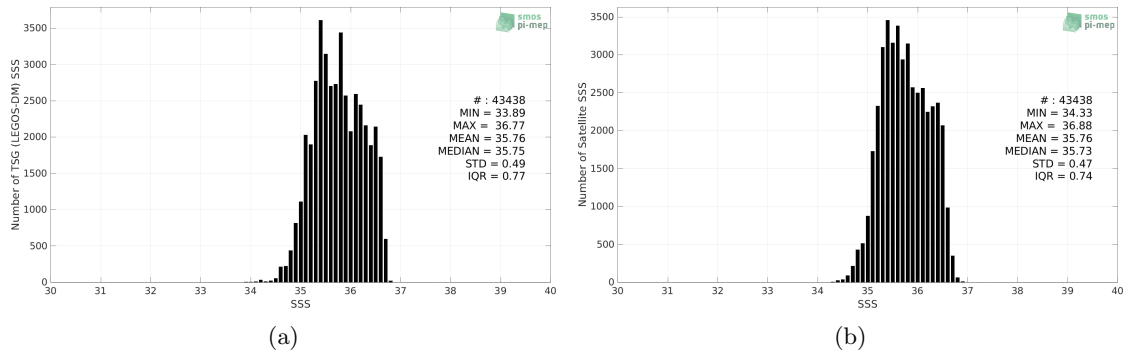
Figure 2: Histograms of SSS from TSG (LEGOS-DM) (a) and SMOS and SMAP SSS L4 OI v1 - 7 Days (LOPS) (b) considering all match-up pairs per bins of 0.1 over the OTT zone Pi-MEP region and for the full satellite product period.
