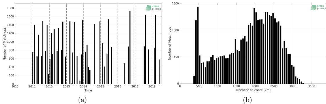
Figure 1: Number of match-ups between TSG (LEGOS-DM) and SMOS and SMAP SSS L4 OI v1 - 7 Days (LOPS) SSS as a function of time (a) and as function of the distance to coast (b) over the OTT zone Pi-MEP region and for the full satellite product period.
