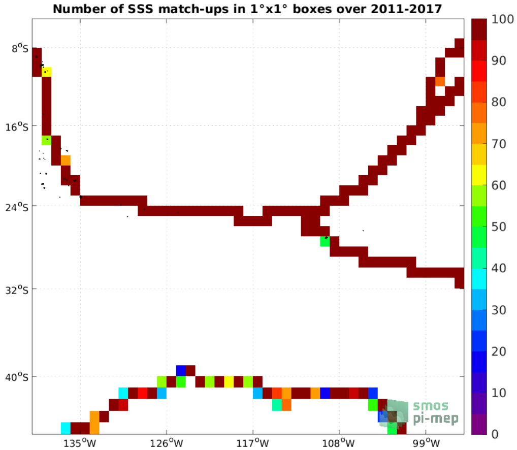
Figure 4: Number of SSS match-ups between TSG (GOSUD-Sailing-ship) SSS and the SMOS and SMAP SSS L4 OI v1 - 7 Days (LOPS) SSS product for the OTT zone Pi-MEP region over 1°x1° boxes and for the full satellite product period.
