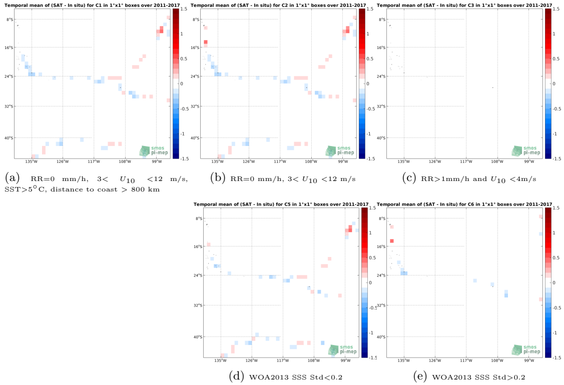
Figure 12: Temporal mean gridded over spatial boxes of size 1^\circ \times 1^\circ of \Delta\text{SSS} (SMOS and SMAP SSS L4 OI v1 - 7 Days (LOPS) - TSG (GOSUD-Sailing-ship)) for 5 different subdatasets corresponding to:RR=0 mm/h, 3 < U_{10} < 12 m/s, SST>5°C, distance to coast > 800 km (a), RR=0 mm/h, 3 < U_{10} < 12 m/s (b), RR>1mm/h and U_{10} < 4 m/s (c), WOA2013 SSS Std<0.2 (d), WOA2013 SSS Std>0.2 (e).
