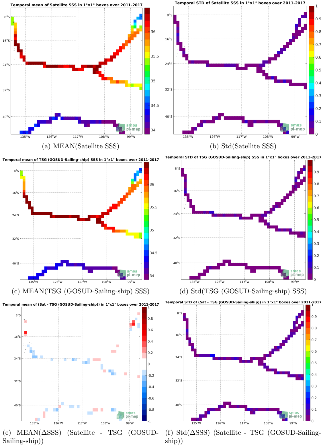
Figure 6: Temporal mean (left) and Std (right) of SSS from SMOS and SMAP SSS L4 OI v1 - 7 Days (LOPS) (top), TSG (GOSUD-Sailing-ship) (middle), and of \Delta SSS (Satellite - TSG (GOSUD-Sailing-ship)). Only match-up pairs are used to generate these maps.
