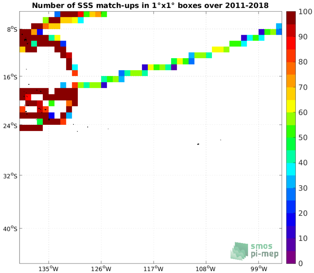
Figure 4: Number of SSS match-ups between TSG (GOSUD-Research-vessel) SSS and the SMOS and SMAP SSS L4 OI v1 - 7 Days (LOPS) SSS product for the OTT zone Pi-MEP region over 1°x1° boxes and for the full satellite product period.
