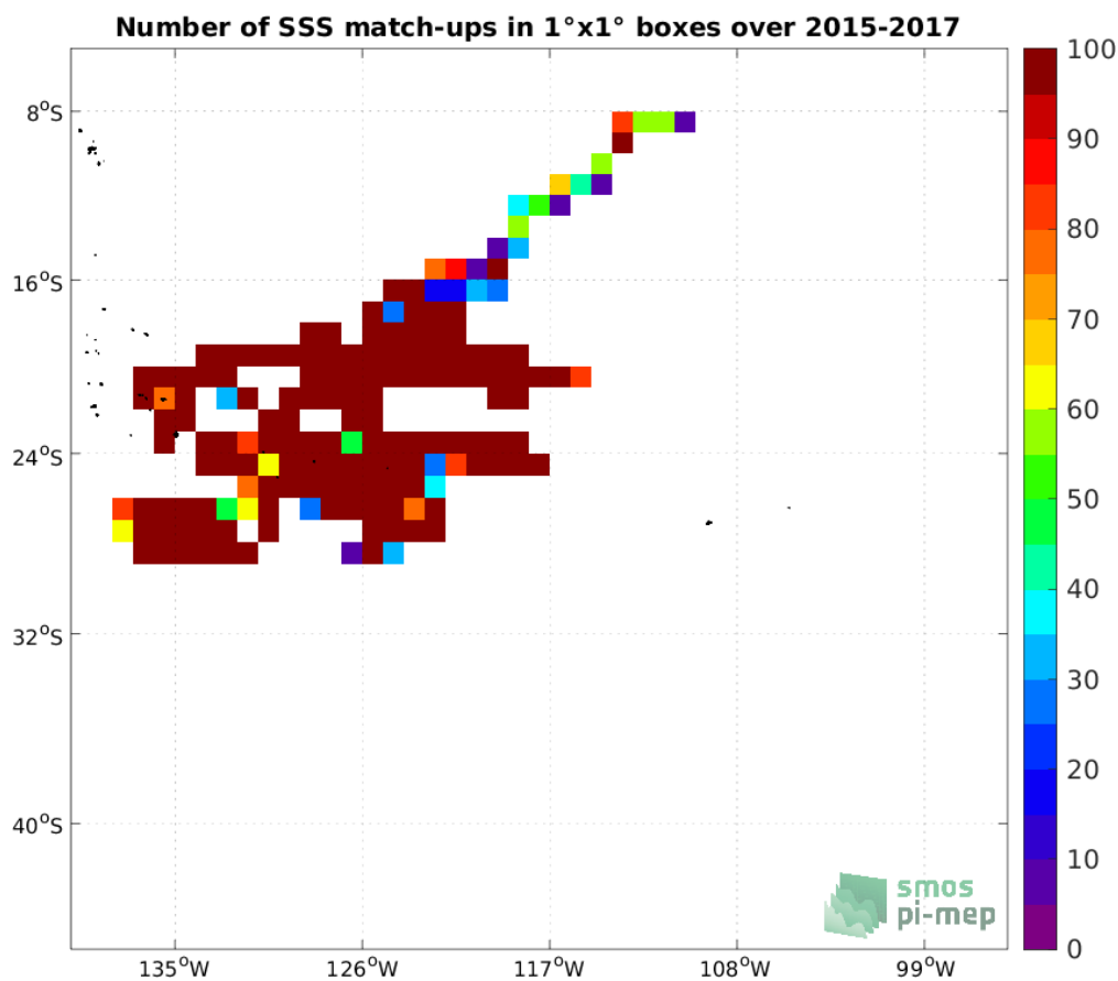
Figure 3: Number of SSS match-ups between Surface drifters SSS and the SMOS and SMAP SSS L4 OI v1 - 7 Days (LOPS) SSS product for the OTT zone Pi-MEP region over 1°x1° boxes and for the full satellite product period.
