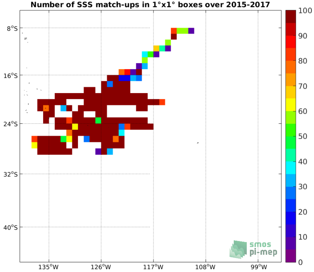
Figure 3: Number of SSS match-ups between Surface drifters SSS and the SMOS and SMAP SSS L4 OI v1 - 7 Days (LOPS) SSS product for the OTT zone Pi-MEP region over 1^\circ \times 1^\circ boxes and for the full satellite product period.
