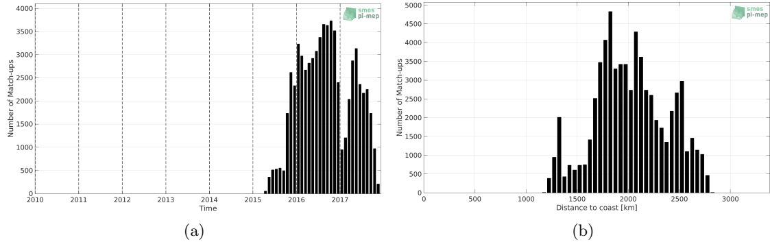
Figure 1: Number of match-ups between Surface drifters and SMOS and SMAP SSS L4 OI v1 - 7 Days (LOPS) SSS as a function of time (a) and as function of the distance to coast (b) over the OTT zone Pi-MEP region and for the full satellite product period.
