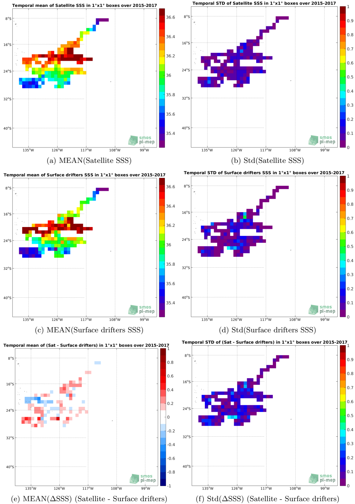
Figure 5: Temporal mean (left) and Std (right) of SSS from SMOS and SMAP SSS L4 OI v1 - 7 Days (LOPS) (top), Surface drifters (middle), and of \Delta SSS (Satellite - Surface drifters). Only match-up pairs are used to generate these maps.
