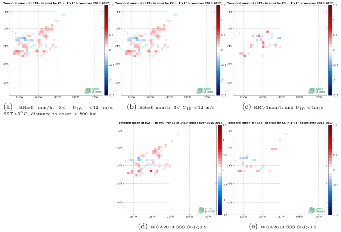
Figure 11: Temporal mean gridded over spatial boxes of size 1^\circ \times 1^\circ of \Delta SSS (SMOS and SMAP SSS L4 OI v1 - 7 Days (LOPS) - Surface drifters) for 5 different subdatasets corresponding to: RR=0 mm/h, 3 < U_{10} < 12 m/s, SST >5^\circ C, distance to coast > 800 km (a), RR=0 mm/h, 3 < U_{10} < 12 m/s (b), RR >1 mm/h and U_{10} < 4 m/s (c), WOA2013 SSS Std <0.2 (d), WOA2013 SSS Std >0.2 (e).
