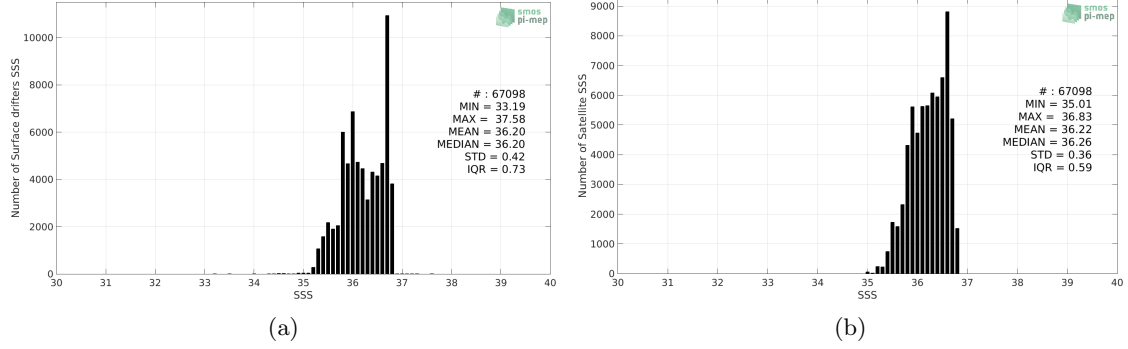
Figure 2: Histograms of SSS from Surface drifters (a) and SMOS and SMAP SSS L4 OI v1 - 7 Days (LOPS) (b) considering all match-up pairs per bins of 0.1 over the OTT zone Pi-MEP region and for the full satellite product period.
