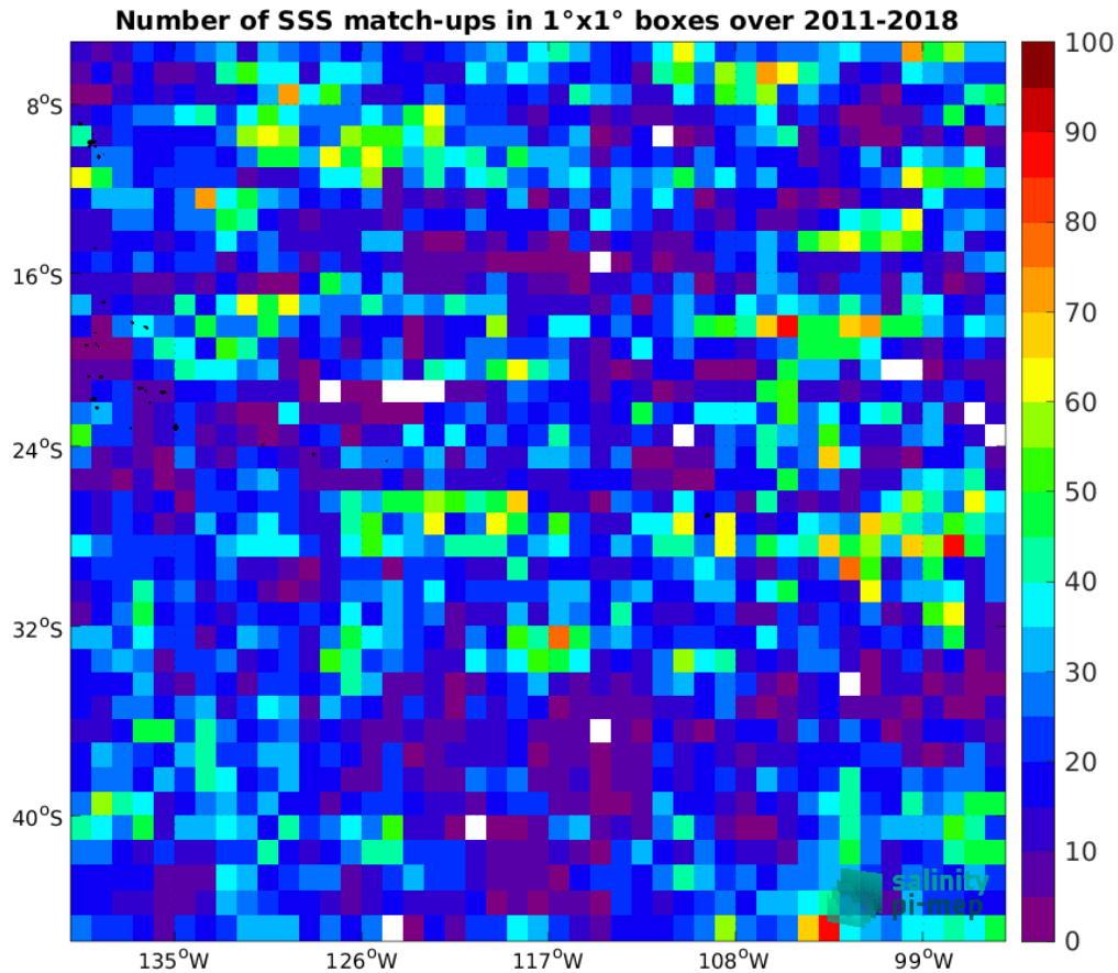
Figure 4: Number of SSS match-ups between Argo SSS and the SMOS and SMAP SSS L4 OI v1 - 7 Days (LOPS) SSS product for the OTT zone Pi-MEP region over 1^\circ \times 1^\circ boxes and for the full satellite product period.
