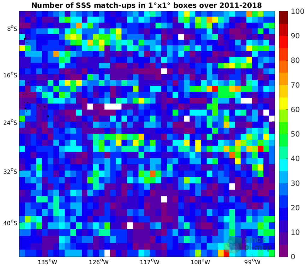
Figure 4: Number of SSS match-ups between Argo SSS and the SMOS and SMAP SSS L4 OI v1 - 7 Days (LOPS) SSS product for the OTT zone Pi-MEP region over 1°x1° boxes and for the full satellite product period.
