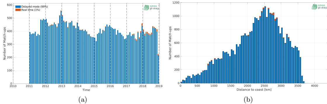
Figure 1: Number of match-ups between Argo and SMOS and SMAP SSS L4 OI v1 - 7 Days (LOPS) SSS as a function of time (a) and as function of the distance to coast (b) over the OTT zone Pi-MEP region and for the full satellite product period.
