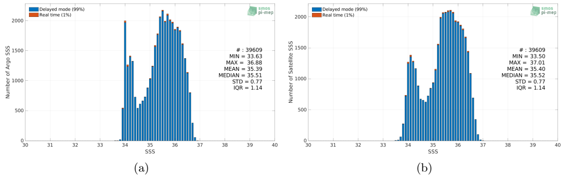
Figure 2: Histograms of SSS from Argo (a) and SMOS and SMAP SSS L4 OI v1 - 7 Days (LOPS) (b) considering all match-up pairs per bins of 0.1 over the OTT zone Pi-MEP region and for the full satellite product period.
