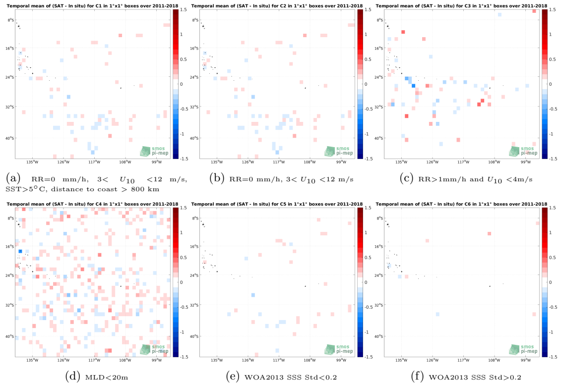
Figure 12: Temporal mean gridded over spatial boxes of size 1^\circ \times 1^\circ of \Delta SSS (SMOS and SMAP SSS L4 OI v1 - 7 Days (LOPS) - Argo) for 6 different subdatasets corresponding to:RR=0 mm/h, 3 < U_{10} < 12 m/s, SST >5^\circ C, distance to coast > 800 km (a), RR=0 mm/h, 3 < U_{10} < 12 m/s (b), RR >1 mm/h and U_{10} < 4 m/s (c),MLD <20 m (d),WOA2013 SSS Std <0.2 (e),WOA2013 SSS Std >0.2 (f).
