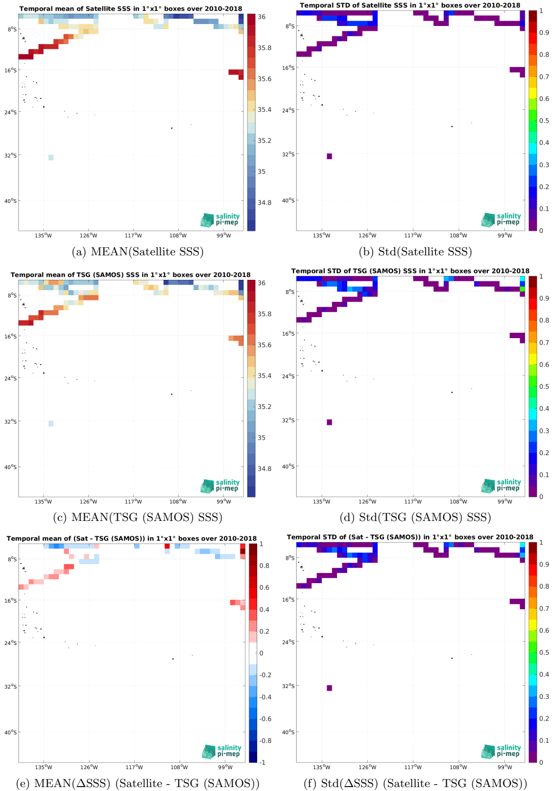
Figure 6: Temporal mean (left) and Std (right) of SSS from SMOS SSS L4 v1 - Weekly (CMEMS-CNR) (top), TSG (SAMOS) (middle), and of \Delta SSS (Satellite - TSG (SAMOS)). Only match-up pairs are used to generate these maps.
