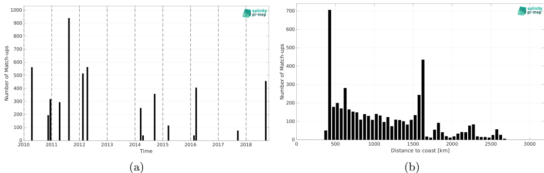
Figure 1: Number of match-ups between TSG (SAMOS) and SMOS SSS L4 v1 - Weekly (CMEMS-CNR) SSS as a function of time (a) and as function of the distance to coast (b) over the OTT zone Pi-MEP region and for the full satellite product period.
