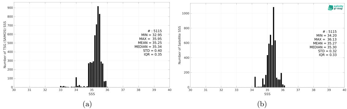
Figure 2: Histograms of SSS from TSG (SAMOS) (a) and SMOS SSS L4 v1 - Weekly (CMEMS-CNR) (b) considering all match-up pairs per bins of 0.1 over the OTT zone Pi-MEP region and for the full satellite product period.
