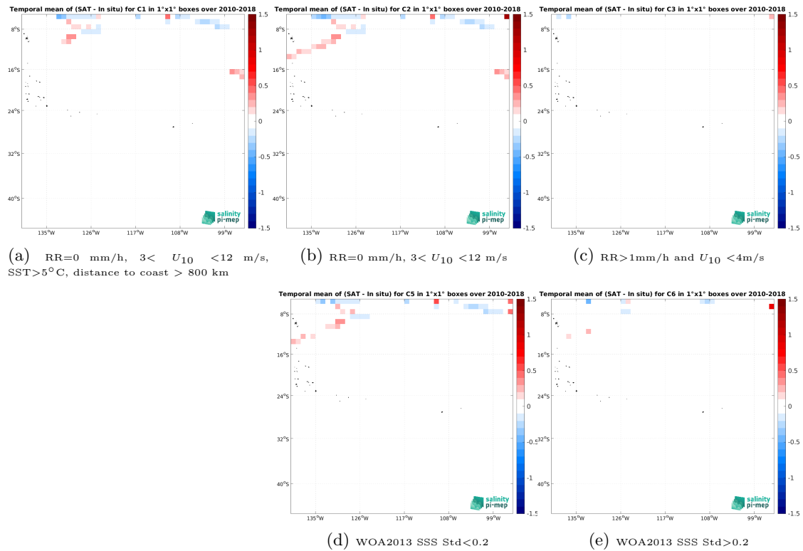
Figure 12: Temporal mean gridded over spatial boxes of size 1^\circ \times 1^\circ of \Delta SSS (SMOS SSS L4 v1 - Weekly (CMEMS-CNR) - TSG (SAMOS)) for 5 different subdatasets corresponding to:RR=0 mm/h, 3 < U_{10} < 12 m/s, SST >5^\circ C, distance to coast > 800 km (a), RR=0 mm/h, 3 < U_{10} < 12 m/s (b), RR >1 mm/h and U_{10} < 4 m/s (c), WOA2013 SSS Std <0.2 (d), WOA2013 SSS Std >0.2 (e).
