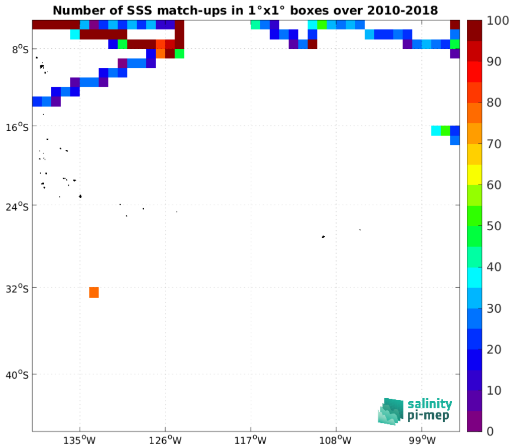
Figure 4: Number of SSS match-ups between TSG (SAMOS) SSS and the SMOS SSS L4 v1 - Weekly (CMEMS-CNR) SSS product for the OTT zone Pi-MEP region over 1^{\circ} \times 1^{\circ} boxes and for the full satellite product period.
