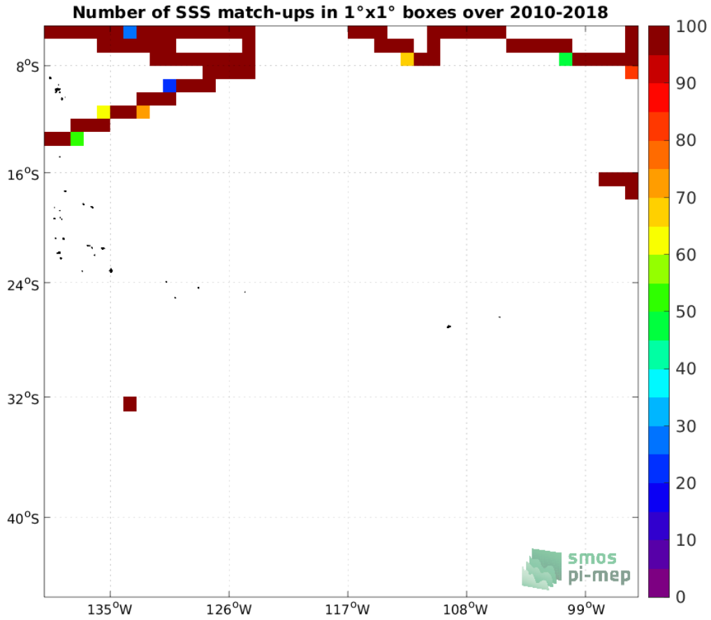
Figure 4: Number of SSS match-ups between TSG (SAMOS) SSS and the SMOS SSS L4 v1 - Weekly (CMEMS-CNR) SSS product for the OTT zone Pi-MEP region over 1^\circ \times 1^\circ boxes and for the full satellite product period.
