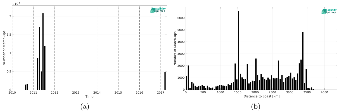
Figure 1: Number of match-ups between TSG (GOSUD-Sailing-ship) and SMOS SSS L4 v1 - Weekly (CMEMS-CNR) SSS as a function of time (a) and as function of the distance to coast (b) over the OTT zone Pi-MEP region and for the full satellite product period.
