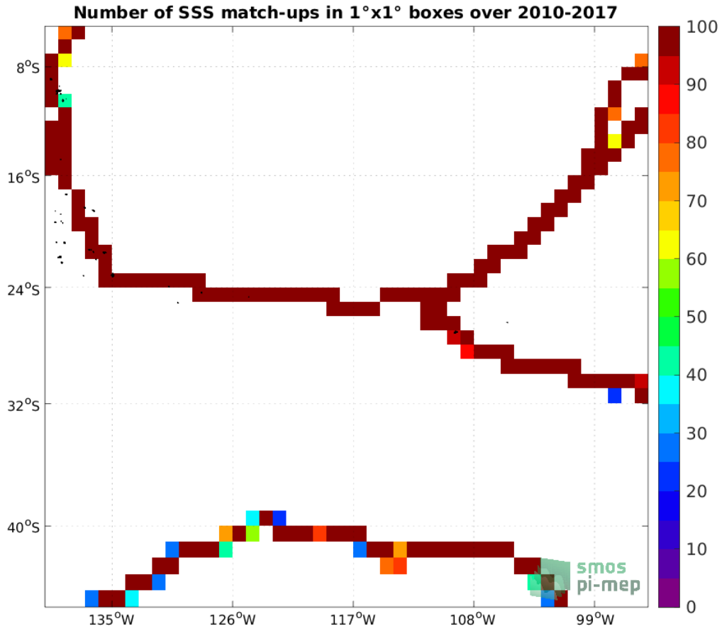
Figure 4: Number of SSS match-ups between TSG (GOSUD-Sailing-ship) SSS and the SMOS SSS L4 v1 - Weekly (CMEMS-CNR) SSS product for the OTT zone Pi-MEP region over 1^\circ \times 1^\circ boxes and for the full satellite product period.
