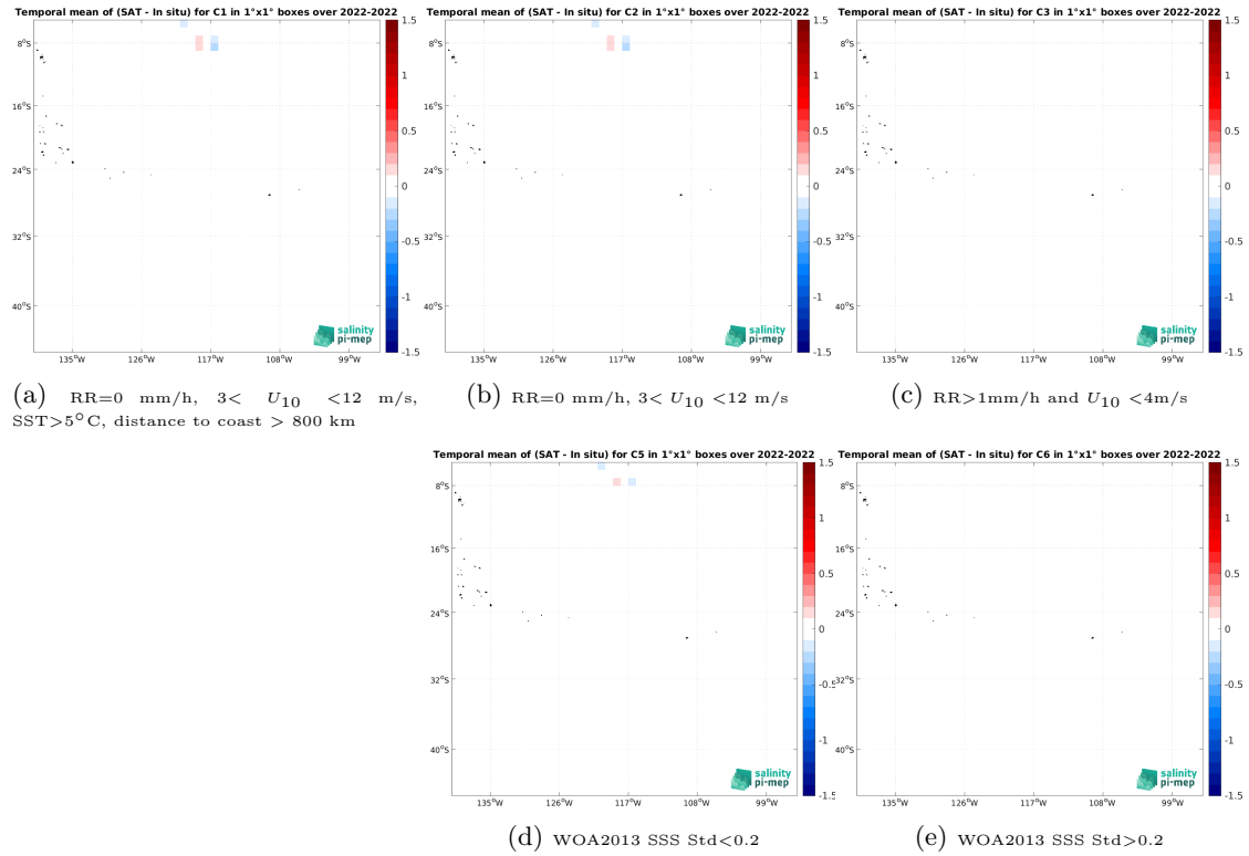
Figure 12: Temporal mean gridded over spatial boxes of size 1^\circ \times 1^\circ of \Delta SSS (SMOS SSS L4 v1 - Weekly (CMEMS-CNR) - Sailability) for 5 different subdatasets corresponding to:RR=0 mm/h, 3 < U_{10} < 12 m/s, SST >5^\circ C, distance to coast > 800 km (a), RR=0 mm/h, 3 < U_{10} < 12 m/s (b), RR >1 mm/h and U_{10} < 4 m/s (c), WOA2013 SSS Std <0.2 (d), WOA2013 SSS Std >0.2 (e).
