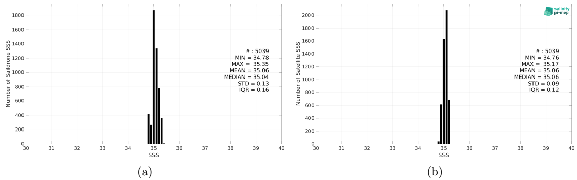
Figure 2: Histograms of SSS from Saildrone (a) and SMOS SSS L4 v1 - Weekly (CMEMS-CNR) (b) considering all match-up pairs per bins of 0.1 over the OTT zone Pi-MEP region and for the full satellite product period.
