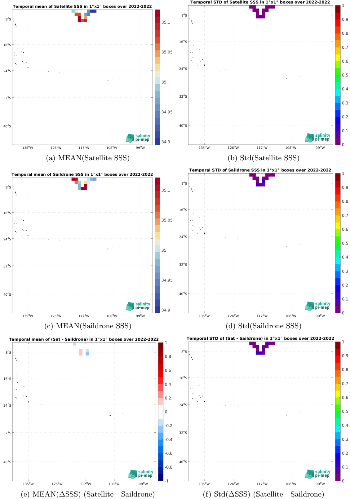
Figure 6: Temporal mean (left) and Std (right) of SSS from SMOS SSS L4 v1 - Weekly (CMEMS-CNR) (top), Saildrone (middle), and of \Delta SSS (Satellite - Saildrone). Only match-up pairs are used to generate these maps.
