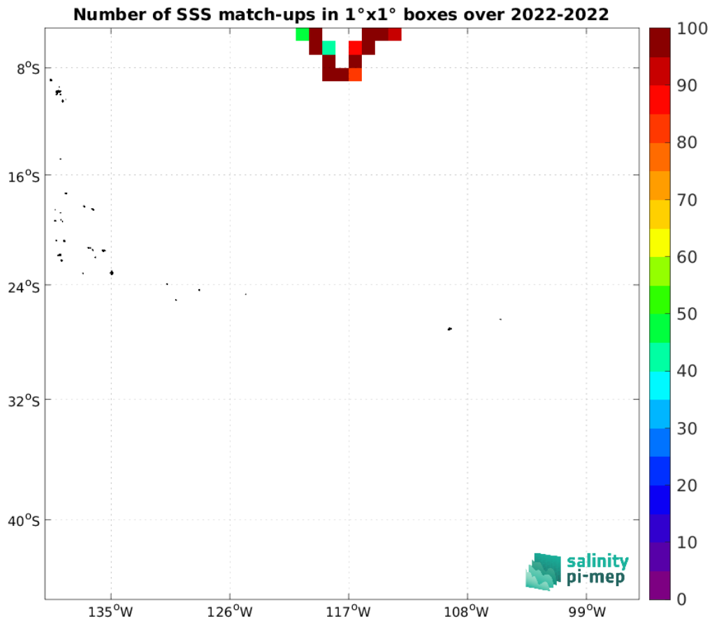
Figure 4: Number of SSS match-ups between Saildrone SSS and the SMOS SSS L4 v1 - Weekly (CMEMS-CNR) SSS product for the OTT zone Pi-MEP region over 1°x1° boxes and for the full satellite product period.
