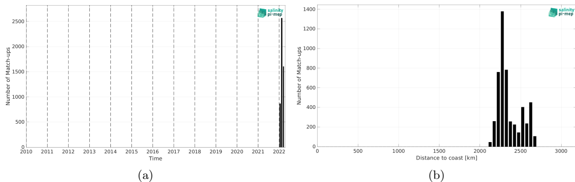
Figure 1: Number of match-ups between Saildrone and SMOS SSS L4 v1 - Weekly (CMEMS-CNR) SSS as a function of time (a) and as function of the distance to coast (b) over the OTT zone Pi-MEP region and for the full satellite product period.
