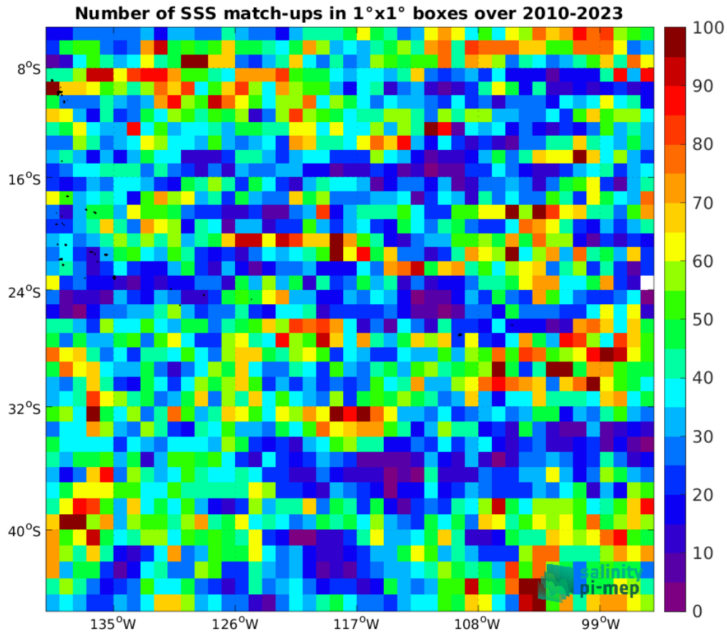
Figure 4: Number of SSS match-ups between Argo SSS and the SMOS SSS L4 v1 - Weekly (CMEMS-CNR) SSS product for the OTT zone Pi-MEP region over 1^\circ \times 1^\circ boxes and for the full satellite product period.
