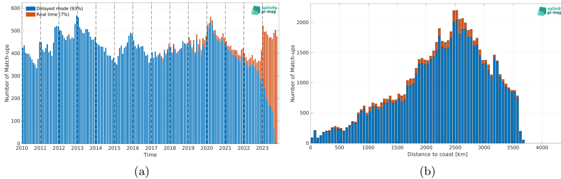
Figure 1: Number of match-ups between Argo and SMOS SSS L4 v1 - Weekly (CMEMS-CNR) SSS as a function of time (a) and as function of the distance to coast (b) over the OTT zone Pi-MEP region and for the full satellite product period.
