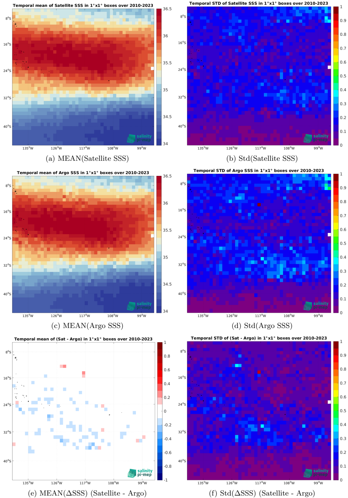
Figure 6: Temporal mean (left) and Std (right) of SSS from SMOS SSS L4 v1 - Weekly (CMEMS-CNR) (top), Argo (middle), and of \Delta\text{SSS} (Satellite - Argo). Only match-up pairs are used to generate these maps.
