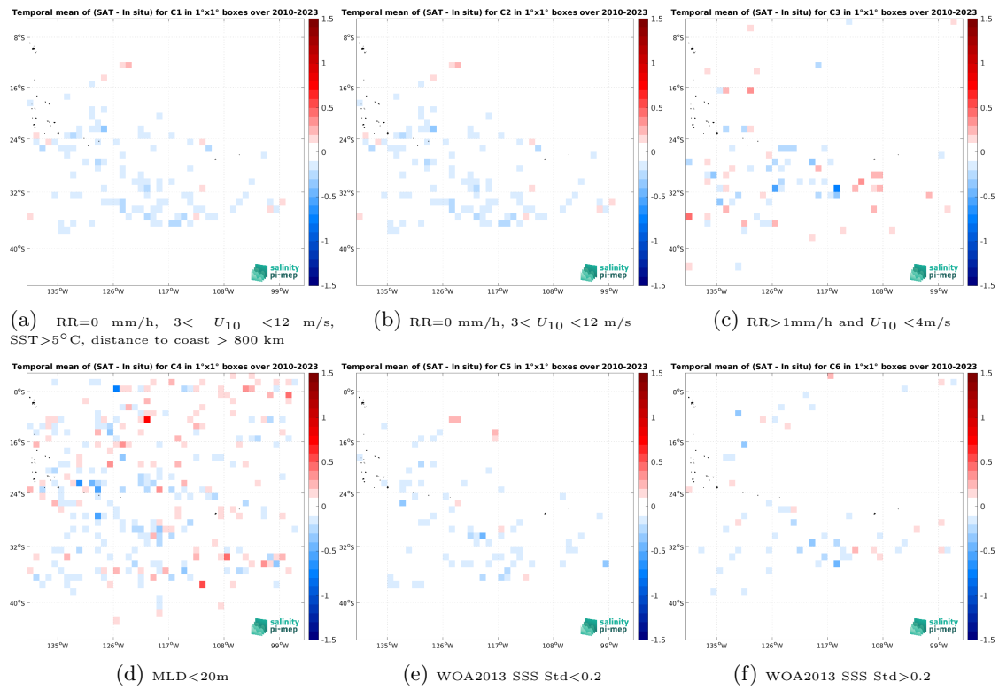
Figure 12: Temporal mean gridded over spatial boxes of size 1^\circ \times 1^\circ of \Delta SSS (SMOS SSS L4 v1 - Weekly (CMEMS-CNR) - Argo) for 6 different subdatasets corresponding to:RR=0 mm/h, 3 < U_{10} < 12 m/s, SST > 5^\circ C , distance to coast > 800 km (a), RR=0 mm/h, 3 < U_{10} < 12 m/s (b), RR > 1 mm/h and U_{10} < 4 m/s (c),MLD < 20 m (d),WOA2013 SSS Std < 0.2 (e),WOA2013 SSS Std > 0.2 (f).
