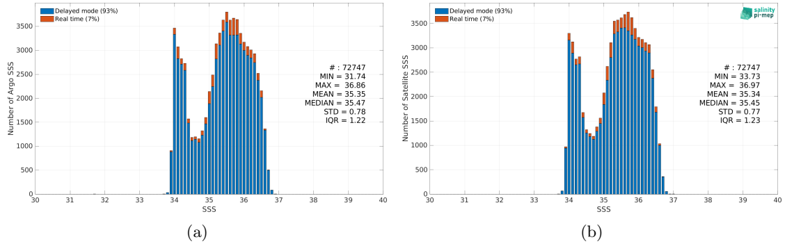
Figure 2: Histograms of SSS from Argo (a) and SMOS SSS L4 v1 - Weekly (CMEMS-CNR) (b) considering all match-up pairs per bins of 0.1 over the OTT zone Pi-MEP region and for the full satellite product period.
