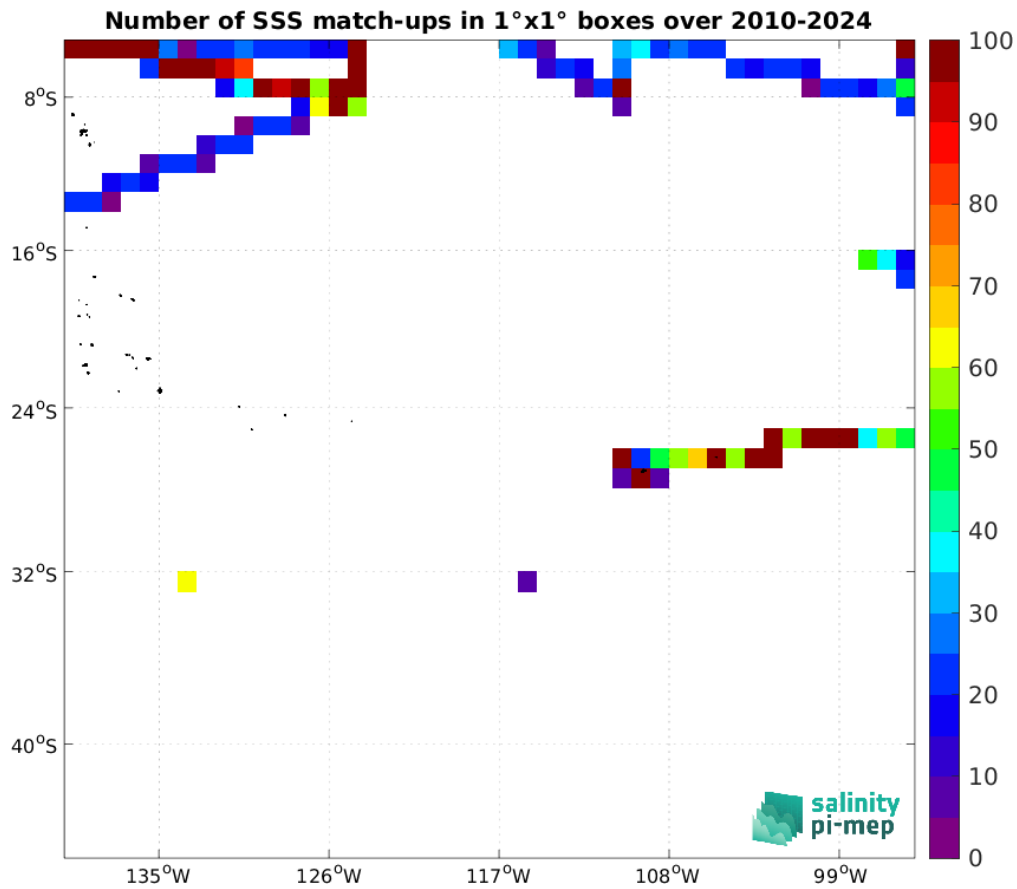
Figure 5: Number of SSS match-ups between TSG (SAMOS) SSS and the SMOS SSS L4 v1 - Monthly (CMEMS-CNR) SSS product for the OTT zone Pi-MEP region over 1^\circ \times 1^\circ boxes and for the full satellite product period.
