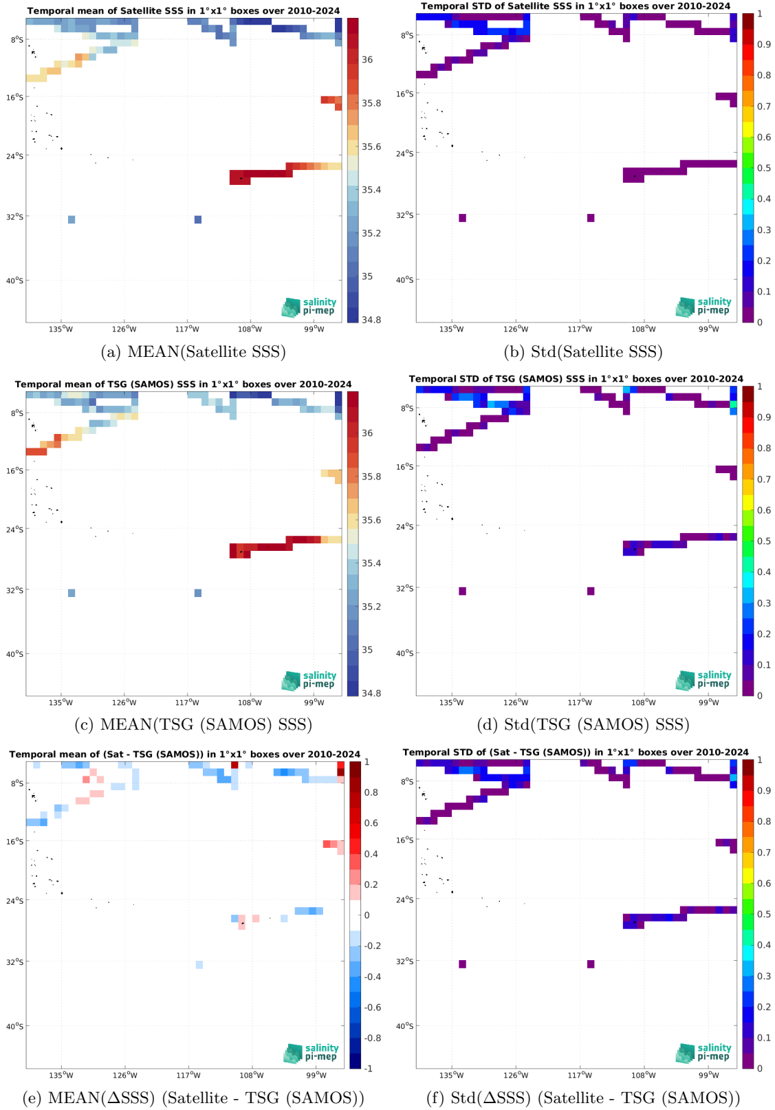
Figure 7: Temporal mean (left) and Std (right) of SSS from SMOS SSS L4 v1 - Monthly (CMEMS-CNR) (top), TSG (SAMOS) (middle), and of \Delta SSS (Satellite - TSG (SAMOS)). Only match-up pairs are used to generate these maps.
