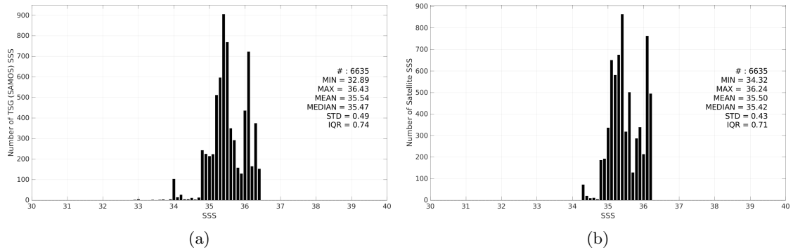
Figure 3: Histograms of SSS from TSG (SAMOS) (a) and SMOS SSS L4 v1 - Monthly (CMEMS-CNR) (b) considering all match-up pairs per bins of 0.1 over the OTT zone Pi-MEP region and for the full satellite product period.
