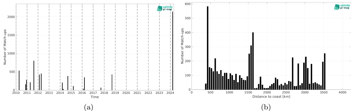
Figure 2: Number of match-ups between TSG (SAMOS) and SMOS SSS L4 v1 - Monthly (CMEMS-CNR) SSS as a function of time (a) and as function of the distance to coast (b) over the OTT zone Pi-MEP region and for the full satellite product period.
