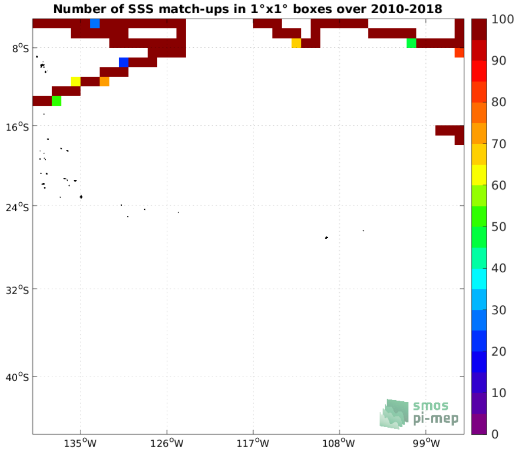
Figure 4: Number of SSS match-ups between TSG (SAMOS) SSS and the SMOS SSS L4 v1 - Monthly (CMEMS-CNR) SSS product for the OTT zone Pi-MEP region over 1^\circ \times 1^\circ boxes and for the full satellite product period.
