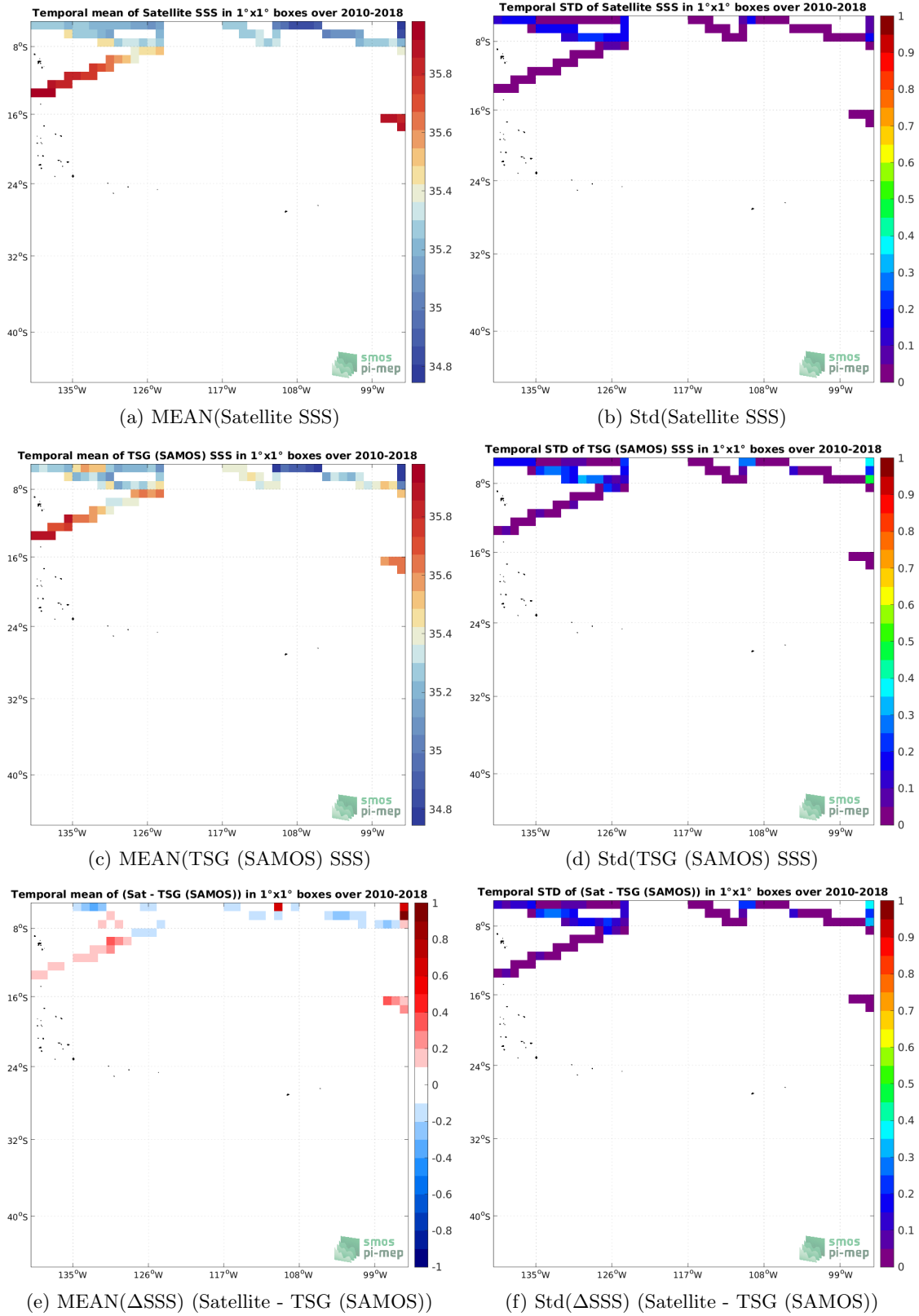
Figure 6: Temporal mean (left) and Std (right) of SSS from SMOS SSS L4 v1 - Monthly (CMEMS-CNR) (top), TSG (SAMOS) (middle), and of \Delta SSS (Satellite - TSG (SAMOS)). Only match-up pairs are used to generate these maps.
