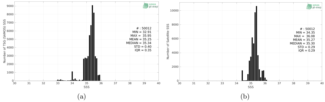
Figure 2: Histograms of SSS from TSG (SAMOS) (a) and SMOS SSS L4 v1 - Monthly (CMEMS-CNR) (b) considering all match-up pairs per bins of 0.1 over the OTT zone Pi-MEP region and for the full satellite product period.
