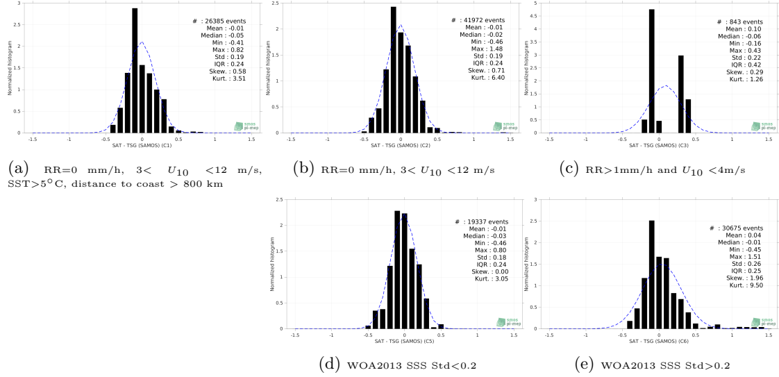
Figure 13: Normalized histogram of \Delta\text{SSS} (SMOS SSS L4 v1 - Monthly (CMEMS-CNR) - TSG (SAMOS)) for 5 different subdatasets corresponding to: RR=0 mm/h, 3 < U_{10} < 12 m/s, SST>5°C, distance to coast > 800 km (a), RR=0 mm/h, 3 < U_{10} < 12 m/s (b), RR>1mm/h and U_{10} < 4 m/s (c), WOA2013 SSS Std<0.2 (d), WOA2013 SSS Std>0.2 (e).
