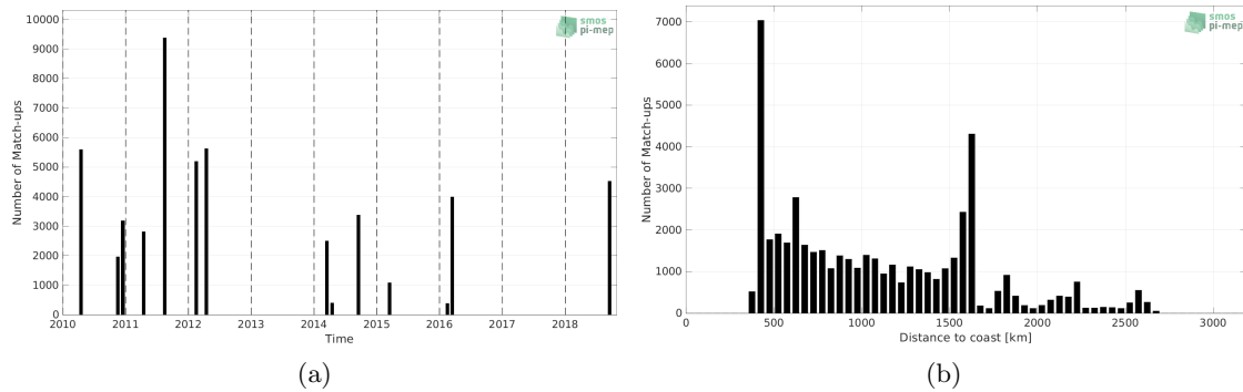
Figure 1: Number of match-ups between TSG (SAMOS) and SMOS SSS L4 v1 - Monthly (CMEMS-CNR) SSS as a function of time (a) and as function of the distance to coast (b) over the OTT zone Pi-MEP region and for the full satellite product period.
