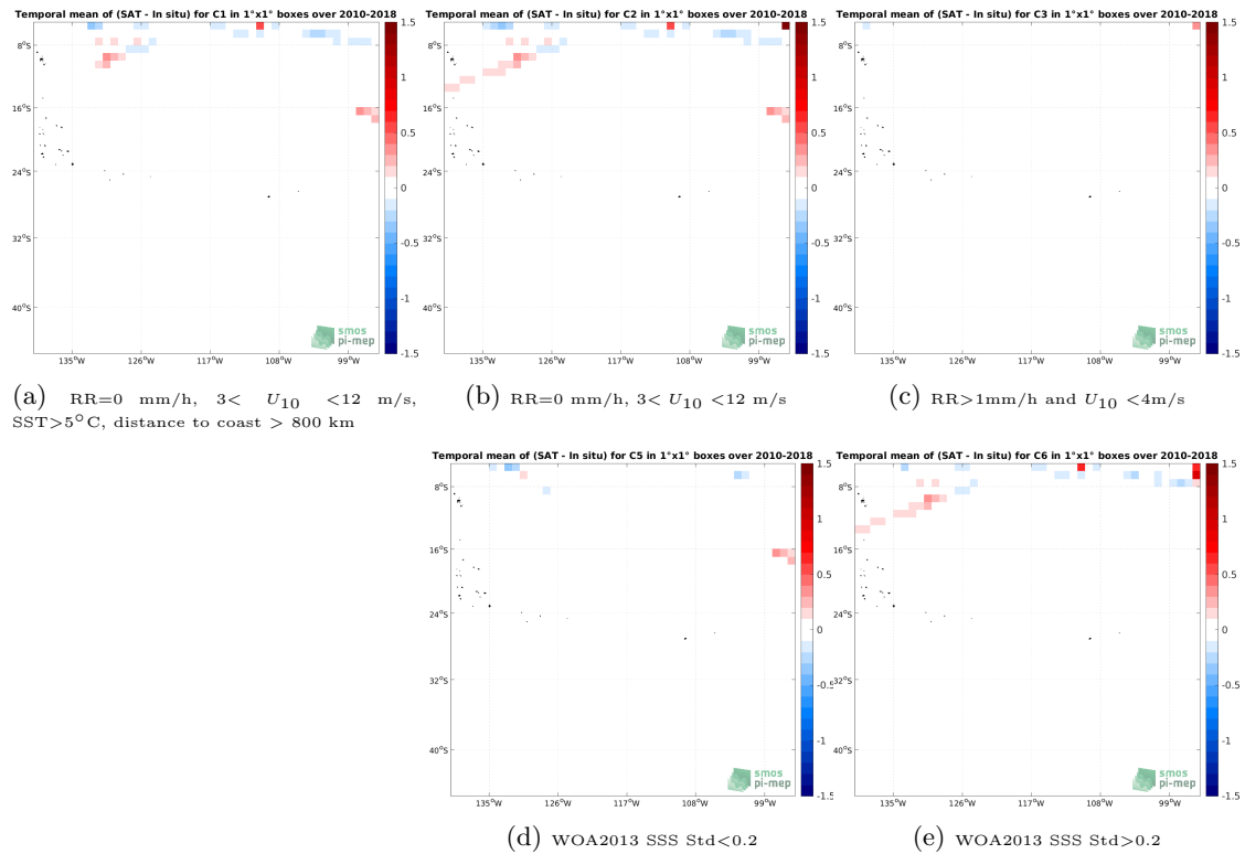
Figure 12: Temporal mean gridded over spatial boxes of size 1^\circ \times 1^\circ of \Delta SSS (SMOS SSS L4 v1 - Monthly (CMEMS-CNR) - TSG (SAMOS)) for 5 different subdatasets corresponding to:RR=0 mm/h, 3 < U_{10} < 12 m/s, SST >5^\circ C, distance to coast > 800 km (a), RR=0 mm/h, 3 < U_{10} < 12 m/s (b), RR >1 mm/h and U_{10} < 4 m/s (c), WOA2013 SSS Std <0.2 (d), WOA2013 SSS Std >0.2 (e).
