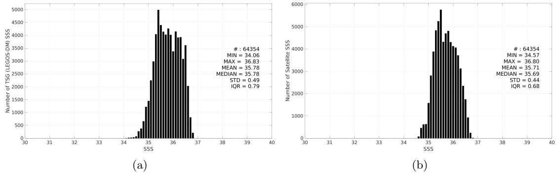
Figure 3: Histograms of SSS from TSG (LEGOS-DM) (a) and SMOS SSS L4 v1 - Monthly (CMEMS-CNR) (b) considering all match-up pairs per bins of 0.1 over the OTT zone Pi-MEP region and for the full satellite product period.
