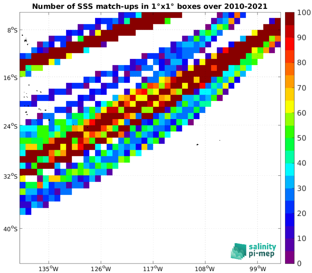
Figure 5: Number of SSS match-ups between TSG (LEGOS-DM) SSS and the SMOS SSS L4 v1 - Monthly (CMEMS-CNR) SSS product for the OTT zone Pi-MEP region over 1°x1° boxes and for the full satellite product period.
