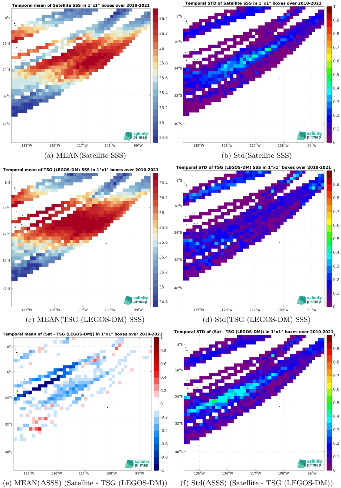
Figure 7: Temporal mean (left) and Std (right) of SSS from SMOS SSS L4 v1 - Monthly (CMEMS-CNR) (top), TSG (LEGOS-DM) (middle), and of \Delta SSS (Satellite - TSG (LEGOS-DM)). Only match-up pairs are used to generate these maps.
