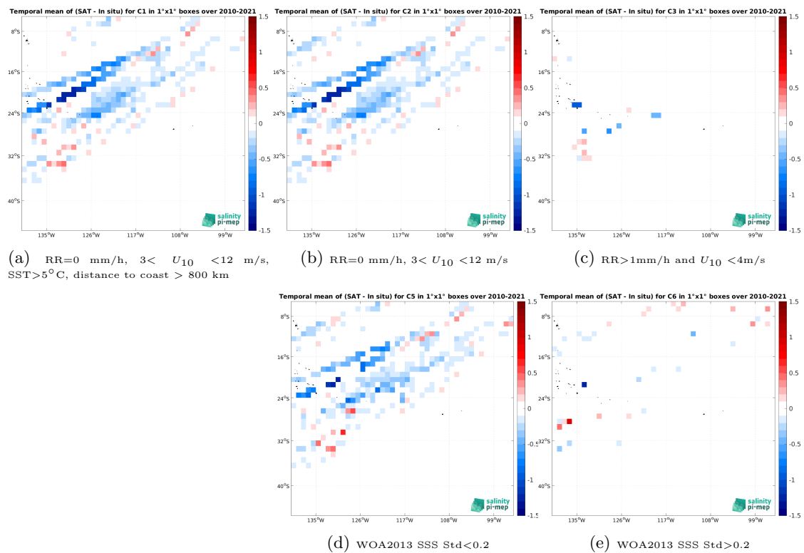
Figure 14: Temporal mean gridded over spatial boxes of size 1^\circ \times 1^\circ of \Delta SSS (SMOS SSS L4 v1 - Monthly (CMEMS-CNR) - TSG (LEGOS-DM)) for 5 different subdatasets corresponding to:RR=0 mm/h, 3 < U_{10} < 12 m/s, SST >5^\circ\text{C} , distance to coast > 800 km (a), RR=0 mm/h, 3 < U_{10} < 12 m/s (b), RR >1 mm/h and U_{10} < 4 m/s (c), WOA2013 SSS Std <0.2 (d), WOA2013 SSS Std >0.2 (e).
