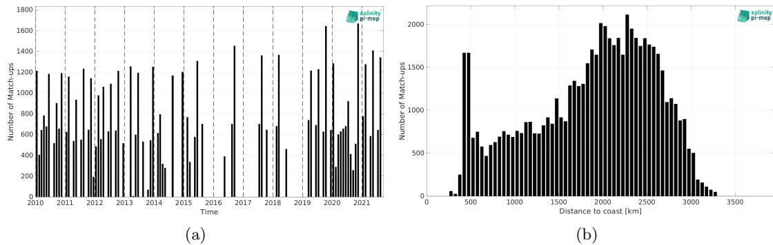
Figure 2: Number of match-ups between TSG (LEGOS-DM) and SMOS SSS L4 v1 - Monthly (CMEMS-CNR) SSS as a function of time (a) and as function of the distance to coast (b) over the OTT zone Pi-MEP region and for the full satellite product period.
