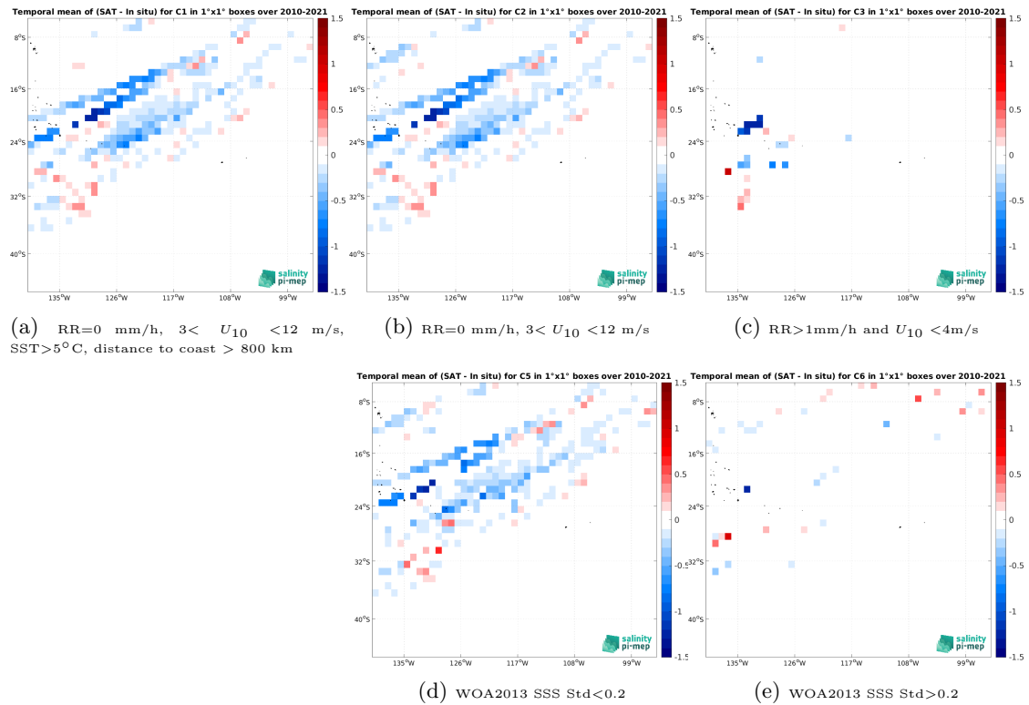
Figure 12: Temporal mean gridded over spatial boxes of size 1^\circ \times 1^\circ of \Delta SSS (SMOS SSS L4 v1 - Monthly (CMEMS-CNR) - TSG (LEGOS-DM)) for 5 different subdatasets corresponding to: RR=0 mm/h, 3 < U_{10} < 12 m/s, SST > 5^\circ\text{C} , distance to coast > 800 km (a), RR=0 mm/h, 3 < U_{10} < 12 m/s (b), RR > 1 mm/h and U_{10} < 4 m/s (c), WOA2013 SSS Std < 0.2 (d), WOA2013 SSS Std > 0.2 (e).
