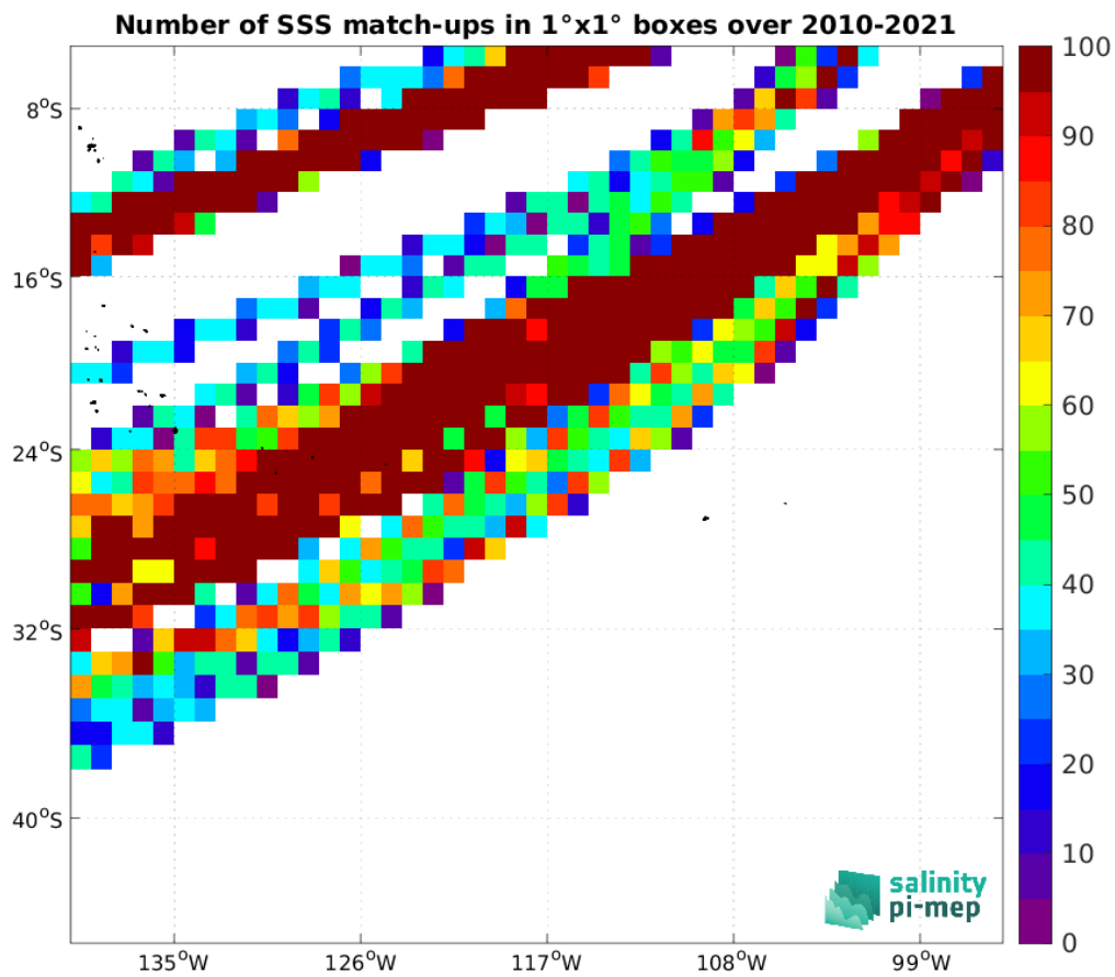
Figure 4: Number of SSS match-ups between TSG (LEGOS-DM) SSS and the SMOS SSS L4 v1 - Monthly (CMEMS-CNR) SSS product for the OTT zone Pi-MEP region over 1^\circ \times 1^\circ boxes and for the full satellite product period.
