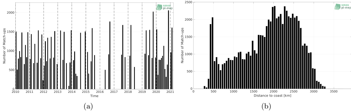
Figure 1: Number of match-ups between TSG (LEGOS-DM) and SMOS SSS L4 v1 - Monthly (CMEMS-CNR) SSS as a function of time (a) and as function of the distance to coast (b) over the OTT zone Pi-MEP region and for the full satellite product period.
