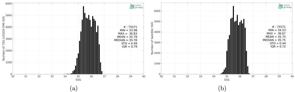
Figure 2: Histograms of SSS from TSG (LEGOS-DM) (a) and SMOS SSS L4 v1 - Monthly (CMEMS-CNR) (b) considering all match-up pairs per bins of 0.1 over the OTT zone Pi-MEP region and for the full satellite product period.
