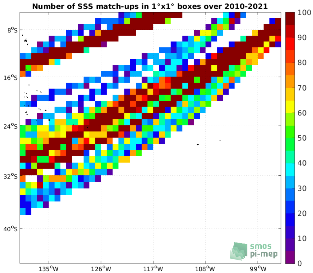
Figure 4: Number of SSS match-ups between TSG (LEGOS-DM) SSS and the SMOS SSS L4 v1 - Monthly (CMEMS-CNR) SSS product for the OTT zone Pi-MEP region over 1°x1° boxes and for the full satellite product period.
