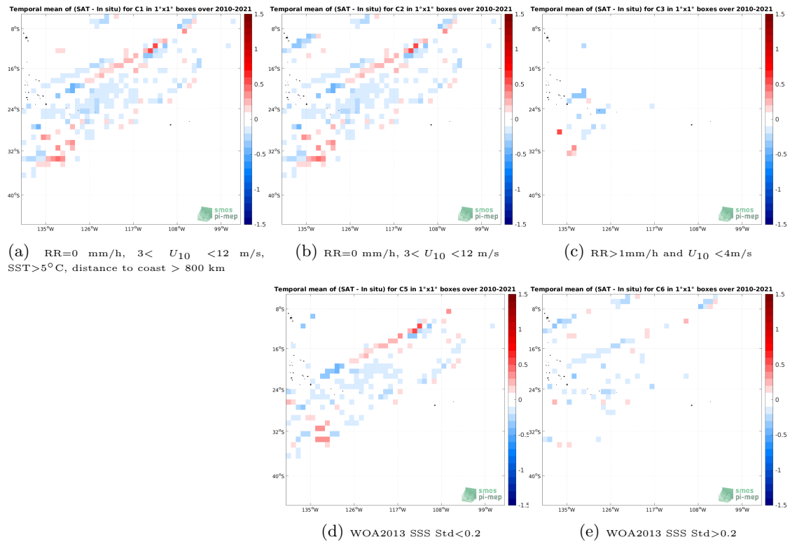
Figure 12: Temporal mean gridded over spatial boxes of size 1^\circ \times 1^\circ of \Delta SSS (SMOS SSS L4 v1 - Monthly (CMEMS-CNR) - TSG (LEGOS-DM)) for 5 different subdatasets corresponding to:RR=0 mm/h, 3 < U_{10} < 12 m/s, SST >5^\circ C, distance to coast > 800 km (a), RR=0 mm/h, 3 < U_{10} < 12 m/s (b), RR >1 mm/h and U_{10} < 4 m/s (c), WOA2013 SSS Std <0.2 (d), WOA2013 SSS Std >0.2 (e).
