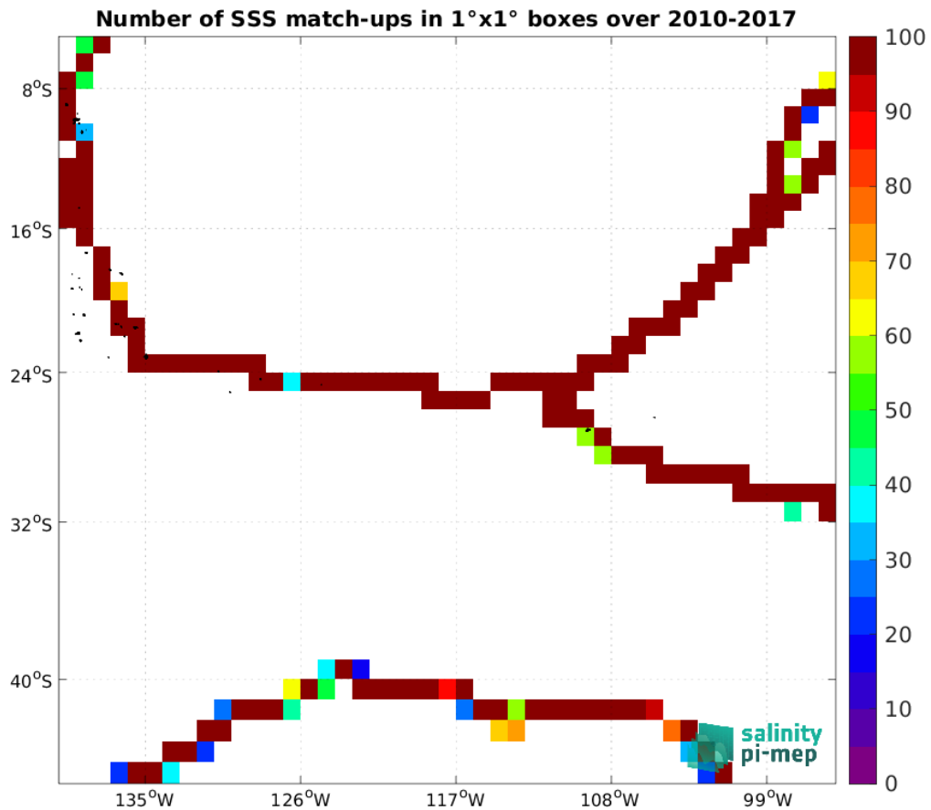
Figure 5: Number of SSS match-ups between TSG (GOSUD-Sailing-ship) SSS and the SMOS SSS L4 v1 - Monthly (CMEMS-CNR) SSS product for the OTT zone Pi-MEP region over 1^\circ \times 1^\circ boxes and for the full satellite product period.
