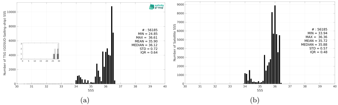
Figure 3: Histograms of SSS from TSG (GOSUD-Sailing-ship) (a) and SMOS SSS L4 v1 - Monthly (CMEMS-CNR) (b) considering all match-up pairs per bins of 0.1 over the OTT zone Pi-MEP region and for the full satellite product period.
