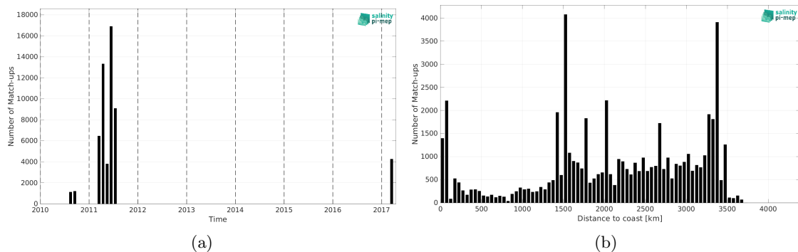
Figure 2: Number of match-ups between TSG (GOSUD-Sailing-ship) and SMOS SSS L4 v1 - Monthly (CMEMS-CNR) SSS as a function of time (a) and as function of the distance to coast (b) over the OTT zone Pi-MEP region and for the full satellite product period.
