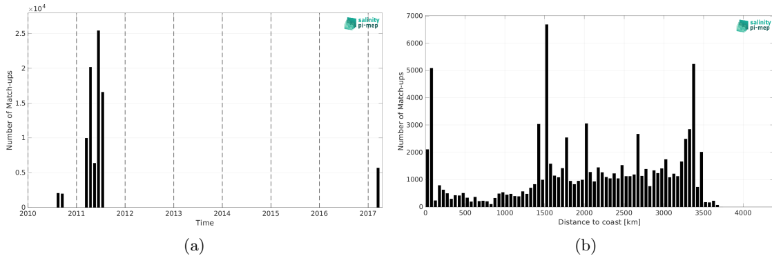
Figure 1: Number of match-ups between TSG (GOSUD-Sailing-ship) and SMOS SSS L4 v1 - Monthly (CMEMS-CNR) SSS as a function of time (a) and as function of the distance to coast (b) over the OTT zone Pi-MEP region and for the full satellite product period.
