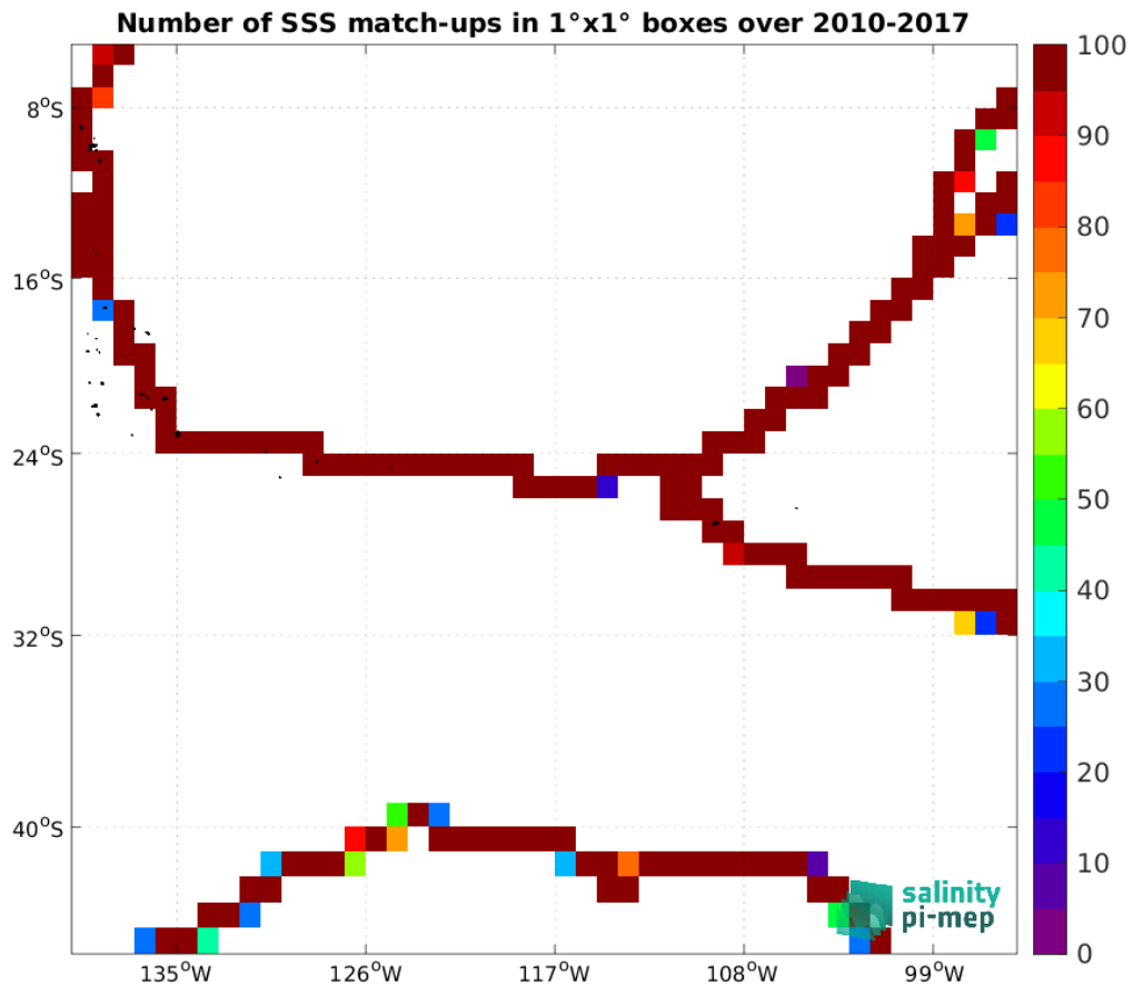
Figure 4: Number of SSS match-ups between TSG (GOSUD-Sailing-ship) SSS and the SMOS SSS L4 v1 - Monthly (CMEMS-CNR) SSS product for the OTT zone Pi-MEP region over 1^\circ \times 1^\circ boxes and for the full satellite product period.
