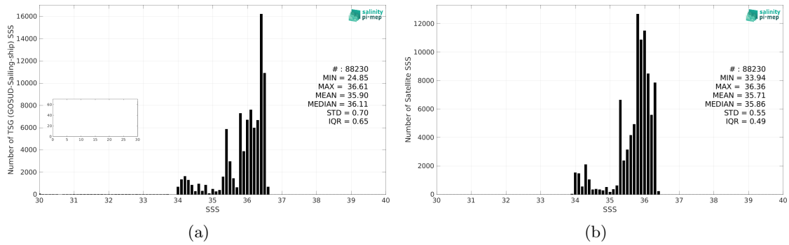
Figure 2: Histograms of SSS from TSG (GOSUD-Sailing-ship) (a) and SMOS SSS L4 v1 - Monthly (CMEMS-CNR) (b) considering all match-up pairs per bins of 0.1 over the OTT zone Pi-MEP region and for the full satellite product period.
