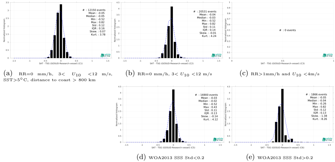
Figure 15: Normalized histogram of \Delta SSS (SMOS SSS L4 v1 - Monthly (CMEMS-CNR) - TSG (GOSUD-Research-vessel)) for 5 different subdatasets corresponding to: RR=0 mm/h, 3 < U_{10} < 12 m/s, SST > 5°C, distance to coast > 800 km (a), RR=0 mm/h, 3 < U_{10} < 12 m/s (b), RR > 1mm/h and U_{10} < 4 m/s (c), WOA2013 SSS Std < 0.2 (d), WOA2013 SSS Std > 0.2 (e).
