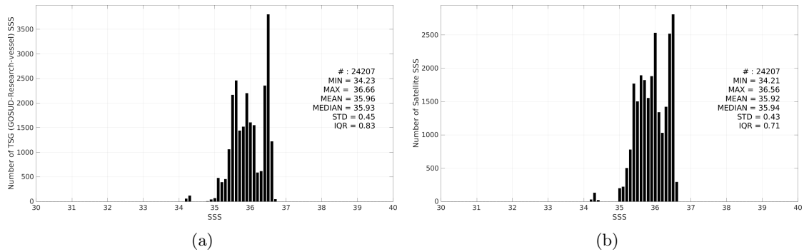
Figure 3: Histograms of SSS from TSG (GOSUD-Research-vessel) (a) and SMOS SSS L4 v1 - Monthly (CMEMS-CNR) (b) considering all match-up pairs per bins of 0.1 over the OTT zone Pi-MEP region and for the full satellite product period.
