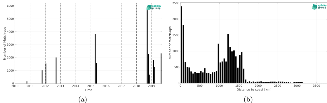
Figure 2: Number of match-ups between TSG (GOSUD-Research-vessel) and SMOS SSS L4 v1 - Monthly (CMEMS-CNR) SSS as a function of time (a) and as function of the distance to coast (b) over the OTT zone Pi-MEP region and for the full satellite product period.
