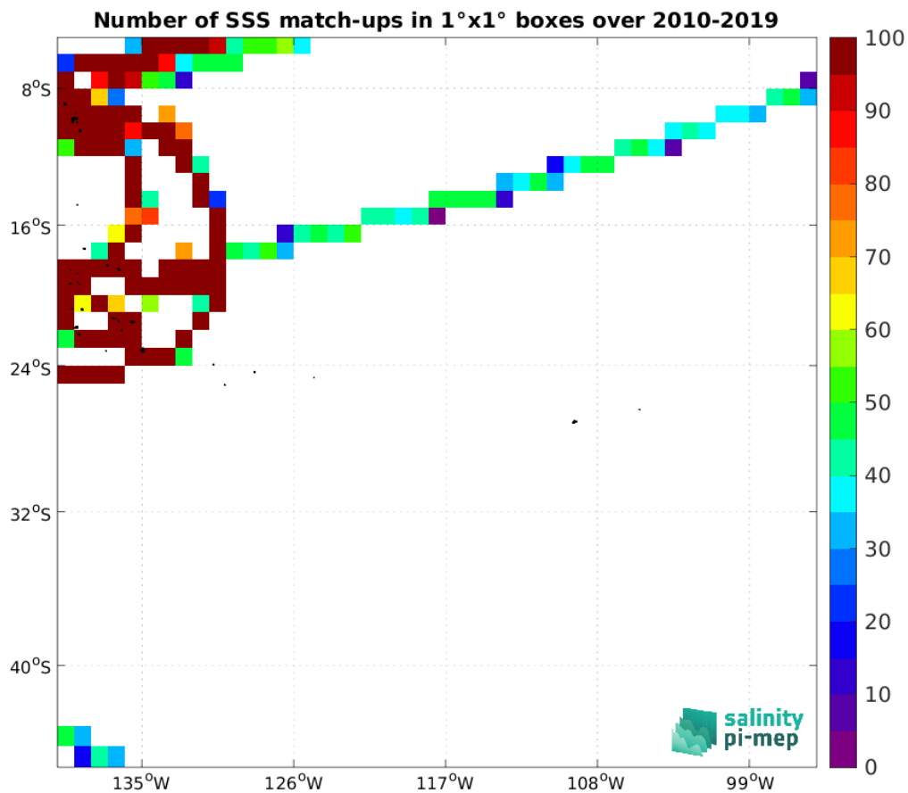
Figure 5: Number of SSS match-ups between TSG (GOSUD-Research-vessel) SSS and the SMOS SSS L4 v1 - Monthly (CMEMS-CNR) SSS product for the OTT zone Pi-MEP region over 1^\circ \times 1^\circ boxes and for the full satellite product period.
