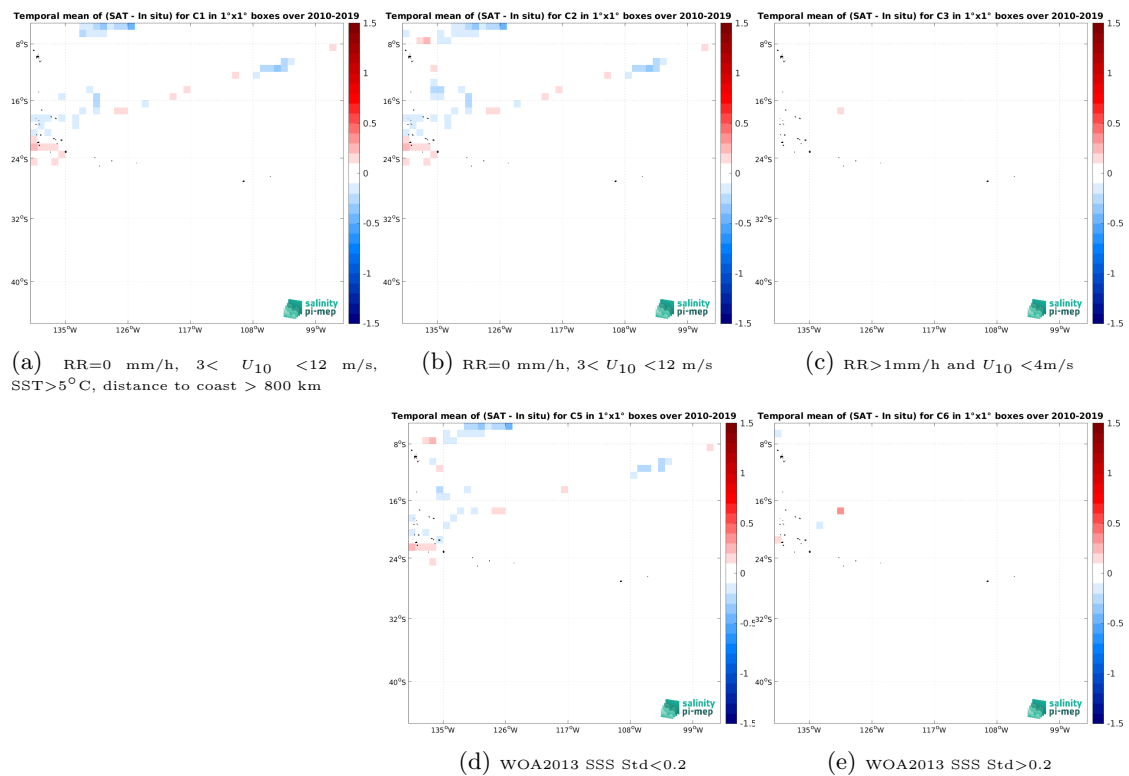
Figure 14: Temporal mean gridded over spatial boxes of size 1^\circ \times 1^\circ of \Delta SSS (SMOS SSS L4 v1 - Monthly (CMEMS-CNR) - TSG (GOSUD-Research-vessel)) for 5 different subdatasets corresponding to:RR=0 mm/h, 3 < U_{10} < 12 m/s, SST >5^\circ C, distance to coast > 800 km (a), RR=0 mm/h, 3 < U_{10} < 12 m/s (b), RR >1 mm/h and U_{10} < 4 m/s (c), WOA2013 SSS Std <0.2 (d), WOA2013 SSS Std >0.2 (e).
