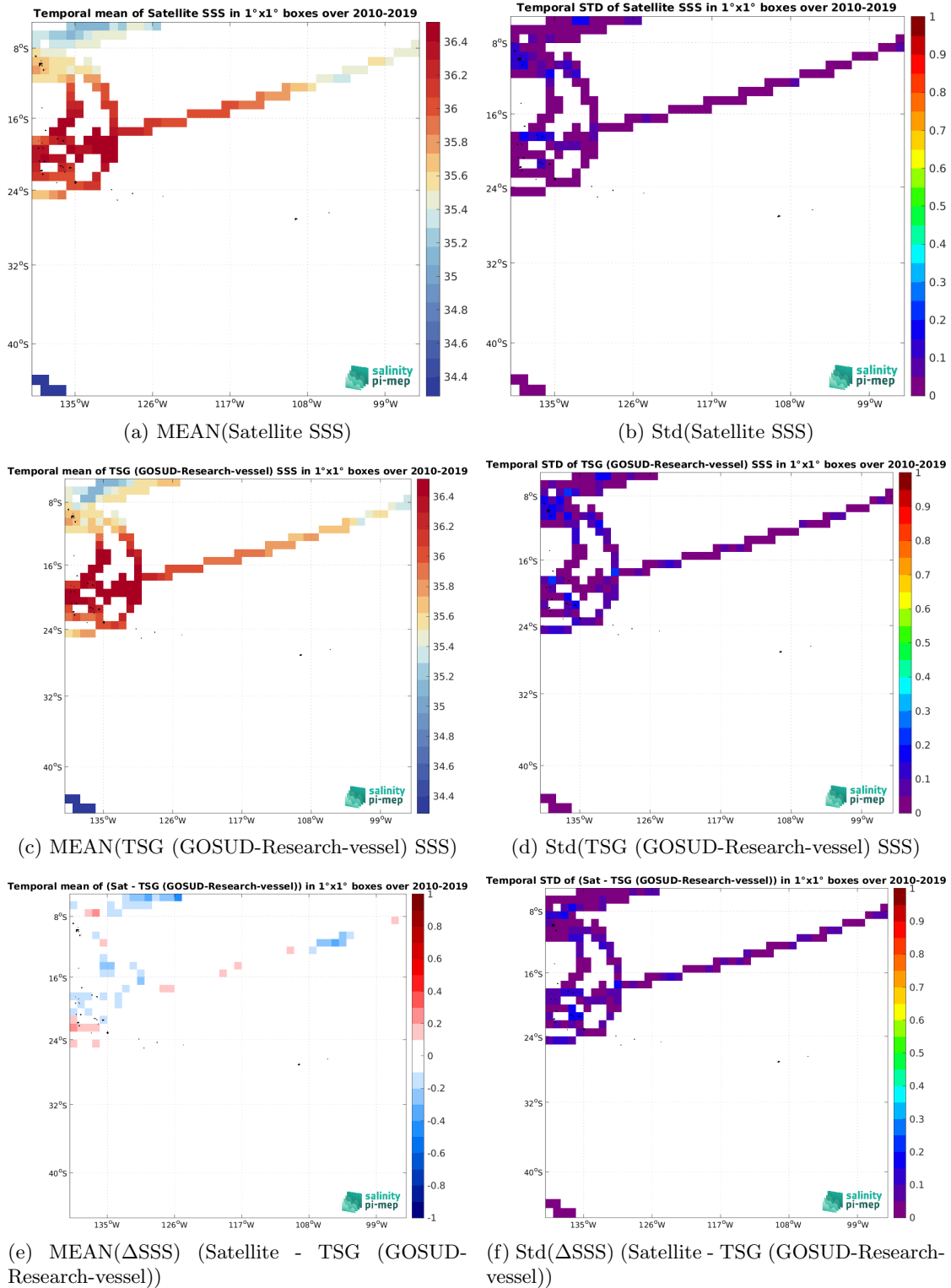
Figure 7: Temporal mean (left) and Std (right) of SSS from SMOS SSS L4 v1 - Monthly (CMEMS-CNR) (top), TSG (GOSUD-Research-vessel) (middle), and of \Delta SSS (Satellite - TSG (GOSUD-Research-vessel)). Only match-up pairs are used to generate these maps.
