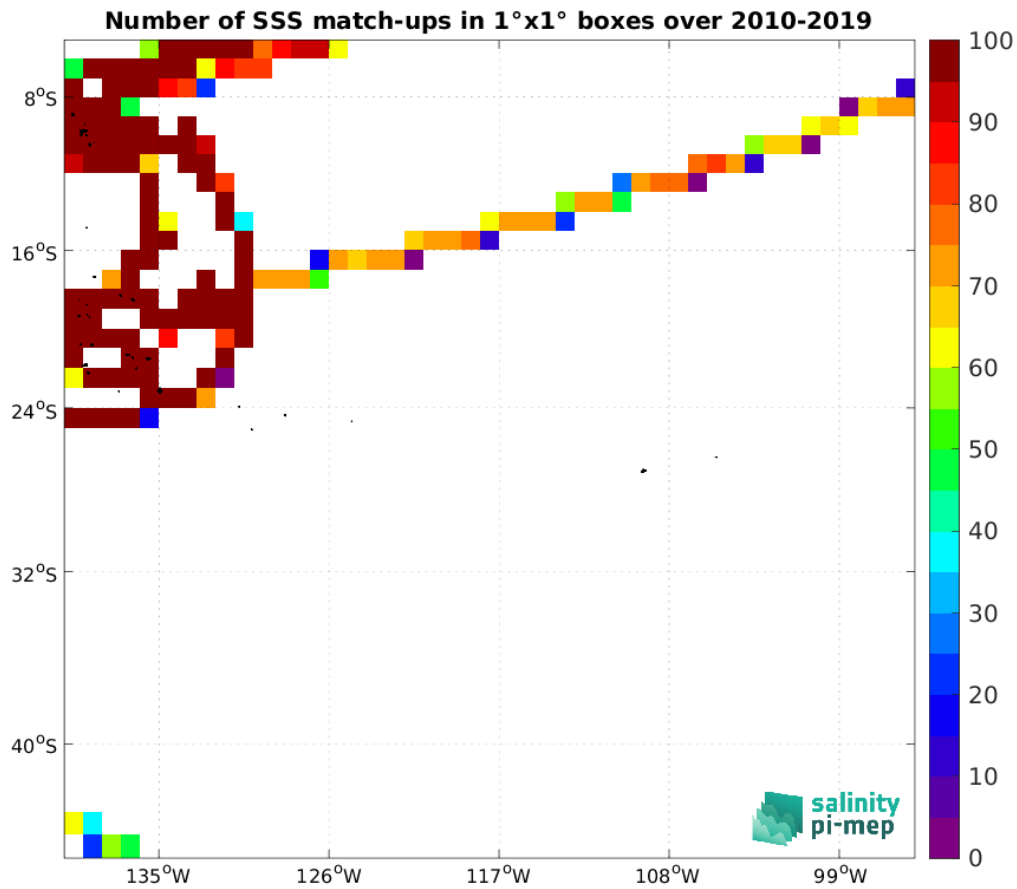
Figure 4: Number of SSS match-ups between TSG (GOSUD-Research-vessel) SSS and the SMOS SSS L4 v1 - Monthly (CMEMS-CNR) SSS product for the OTT zone Pi-MEP region over 1^\circ \times 1^\circ boxes and for the full satellite product period.
