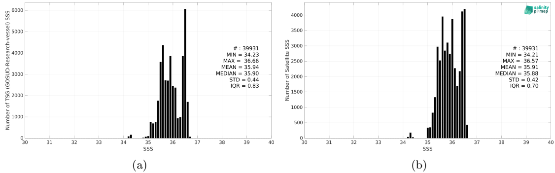
Figure 2: Histograms of SSS from TSG (GOSUD-Research-vessel) (a) and SMOS SSS L4 v1 - Monthly (CMEMS-CNR) (b) considering all match-up pairs per bins of 0.1 over the OTT zone Pi-MEP region and for the full satellite product period.
