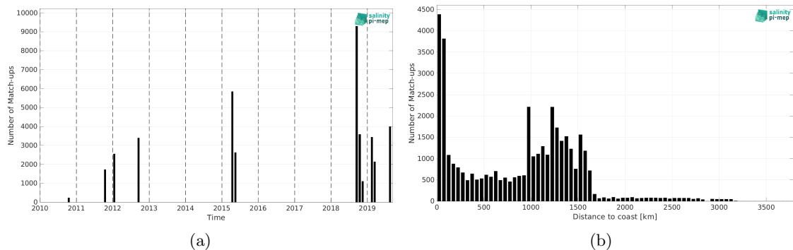
Figure 1: Number of match-ups between TSG (GOSUD-Research-vessel) and SMOS SSS L4 v1 - Monthly (CMEMS-CNR) SSS as a function of time (a) and as function of the distance to coast (b) over the OTT zone Pi-MEP region and for the full satellite product period.
