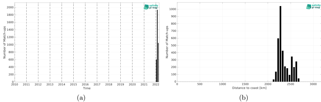
Figure 2: Number of match-ups between Saildrone and SMOS SSS L4 v1 - Monthly (CMEMS-CNR) SSS as a function of time (a) and as function of the distance to coast (b) over the OTT zone Pi-MEP region and for the full satellite product period.
