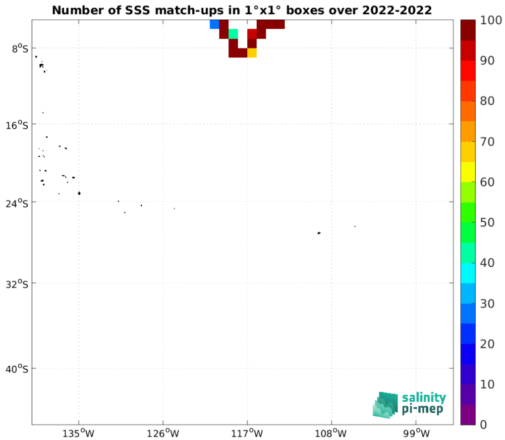
Figure 5: Number of SSS match-ups between Saildrone SSS and the SMOS SSS L4 v1 - Monthly (CMEMS-CNR) SSS product for the OTT zone Pi-MEP region over 1°x1° boxes and for the full satellite product period.
