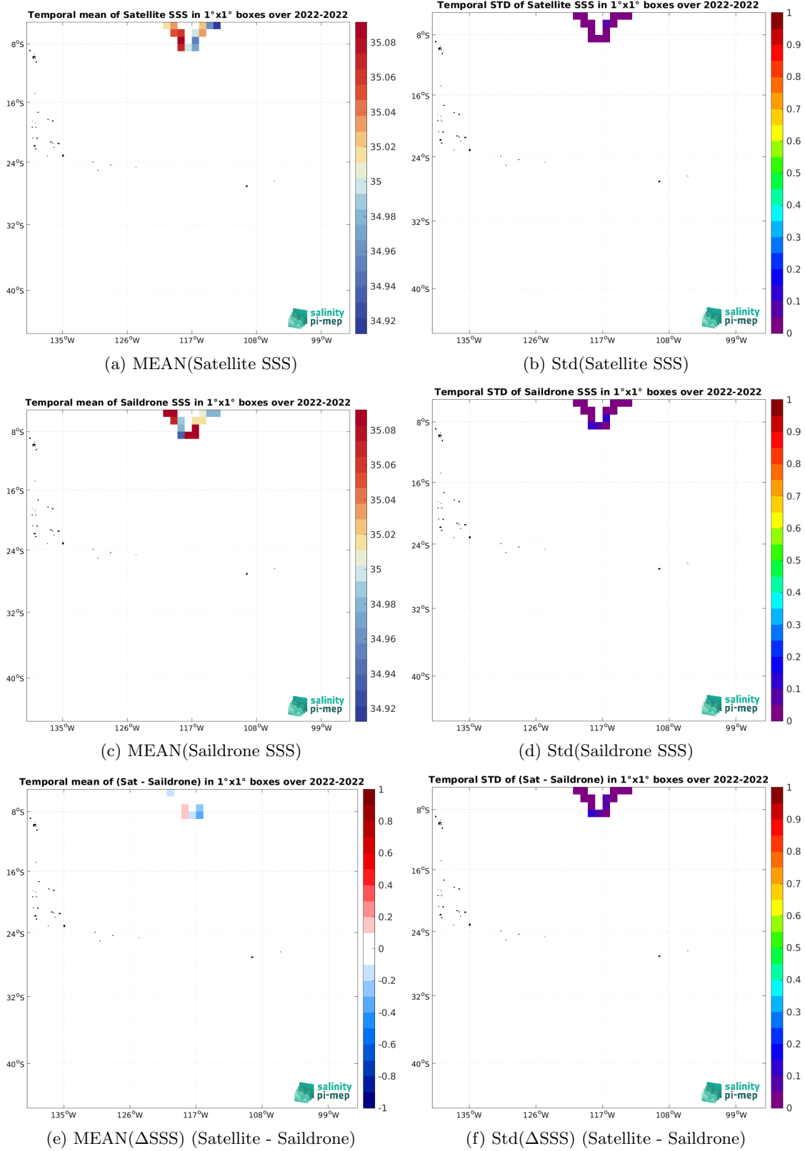
Figure 7: Temporal mean (left) and Std (right) of SSS from SMOS SSS L4 v1 - Monthly (CMEMS-CNR) (top), Saildrone (middle), and of \Delta SSS (Satellite - Saildrone). Only match-up pairs are used to generate these maps.
