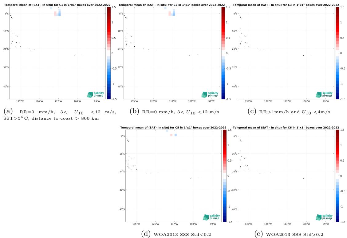
Figure 14: Temporal mean gridded over spatial boxes of size 1^\circ \times 1^\circ of \Delta SSS (SMOS SSS L4 v1 - Monthly (CMEMS-CNR) - Saildrone) for 5 different subdatasets corresponding to: RR=0 mm/h, 3 < U_{10} < 12 m/s, SST > 5^\circ C , distance to coast > 800 km (a), RR=0 mm/h, 3 < U_{10} < 12 m/s (b), RR > 1 mm/h and U_{10} < 4 m/s (c), WOA2013 SSS Std < 0.2 (d), WOA2013 SSS Std > 0.2 (e).
