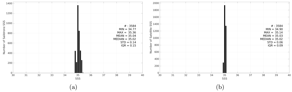
Figure 3: Histograms of SSS from Saildrone (a) and SMOS SSS L4 v1 - Monthly (CMEMS-CNR) (b) considering all match-up pairs per bins of 0.1 over the OTT zone Pi-MEP region and for the full satellite product period.
