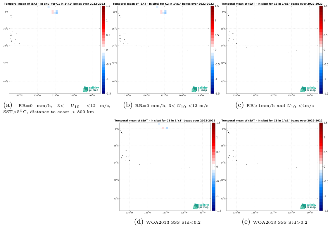
Figure 12: Temporal mean gridded over spatial boxes of size 1^\circ \times 1^\circ of \Delta SSS (SMOS SSS L4 v1 - Monthly (CMEMS-CNR) - Saildrone) for 5 different subdatasets corresponding to:RR=0 mm/h, 3 < U_{10} < 12 m/s, SST >5^\circ C, distance to coast > 800 km (a), RR=0 mm/h, 3 < U_{10} < 12 m/s (b), RR >1 mm/h and U_{10} < 4 m/s (c), WOA2013 SSS Std <0.2 (d), WOA2013 SSS Std >0.2 (e).
