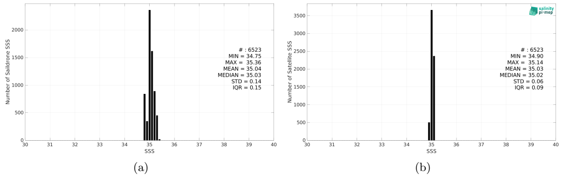
Figure 2: Histograms of SSS from Saildrone (a) and SMOS SSS L4 v1 - Monthly (CMEMS-CNR) (b) considering all match-up pairs per bins of 0.1 over the OTT zone Pi-MEP region and for the full satellite product period.
