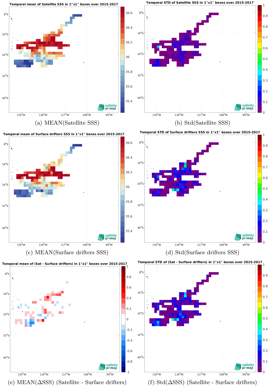
Figure 5: Temporal mean (left) and Std (right) of SSS from SMOS SSS L4 v1 - Monthly (CMEMS-CNR) (top), Surface drifters (middle), and of \Delta SSS (Satellite - Surface drifters). Only match-up pairs are used to generate these maps.
