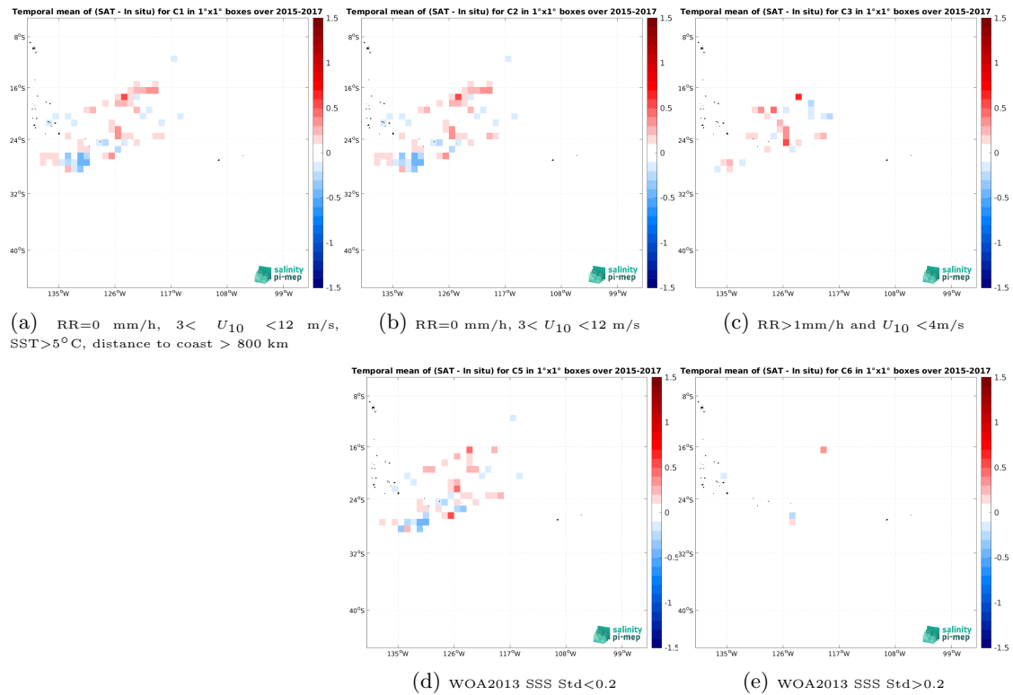
Figure 11: Temporal mean gridded over spatial boxes of size 1^\circ \times 1^\circ of \Delta SSS (SMOS SSS L4 v1 - Monthly (CMEMS-CNR) - Surface drifters) for 5 different subdatasets corresponding to:RR=0 mm/h, 3 < U_{10} < 12 m/s, SST >5^\circ C, distance to coast > 800 km (a), RR=0 mm/h, 3 < U_{10} < 12 m/s (b), RR >1 mm/h and U_{10} < 4 m/s (c), WOA2013 SSS Std <0.2 (d), WOA2013 SSS Std >0.2 (e).
