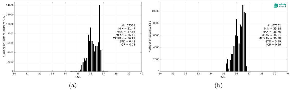
Figure 2: Histograms of SSS from Surface drifters (a) and SMOS SSS L4 v1 - Monthly (CMEMS-CNR) (b) considering all match-up pairs per bins of 0.1 over the OTT zone Pi-MEP region and for the full satellite product period.
