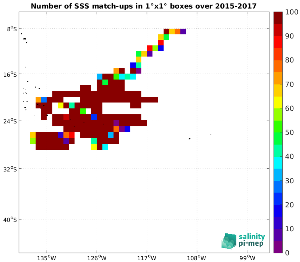
Figure 3: Number of SSS match-ups between Surface drifters SSS and the SMOS SSS L4 v1 - Monthly (CMEMS-CNR) SSS product for the OTT zone Pi-MEP region over 1°x1° boxes and for the full satellite product period.
