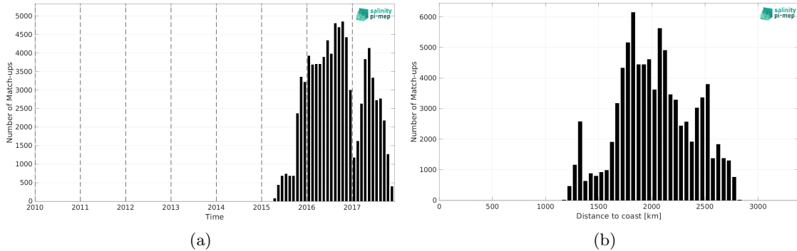
Figure 1: Number of match-ups between Surface drifters and SMOS SSS L4 v1 - Monthly (CMEMS-CNR) SSS as a function of time (a) and as function of the distance to coast (b) over the OTT zone Pi-MEP region and for the full satellite product period.
