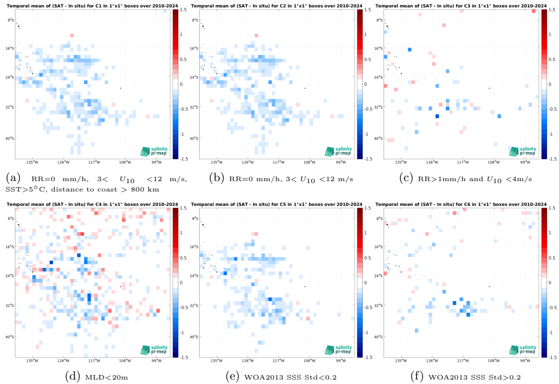
Figure 14: Temporal mean gridded over spatial boxes of size 1^\circ \times 1^\circ of \Delta SSS (SMOS SSS L4 v1 - Monthly (CMEMS-CNR) - Argo) for 6 different subdatasets corresponding to:RR=0 mm/h, 3 < U_{10} < 12 m/s, SST >5^\circ\text{C} , distance to coast > 800 km (a), RR=0 mm/h, 3 < U_{10} < 12 m/s (b), RR >1 mm/h and U_{10} < 4 m/s (c),MLD <20 m (d),WOA2013 SSS Std <0.2 (e),WOA2013 SSS Std >0.2 (f).
