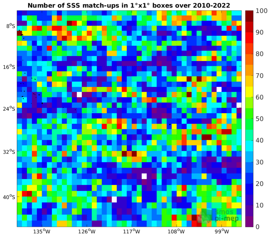
Figure 4: Number of SSS match-ups between Argo SSS and the SMOS SSS L4 v1 - Monthly (CMEMS-CNR) SSS product for the OTT zone Pi-MEP region over 1°x1° boxes and for the full satellite product period.
