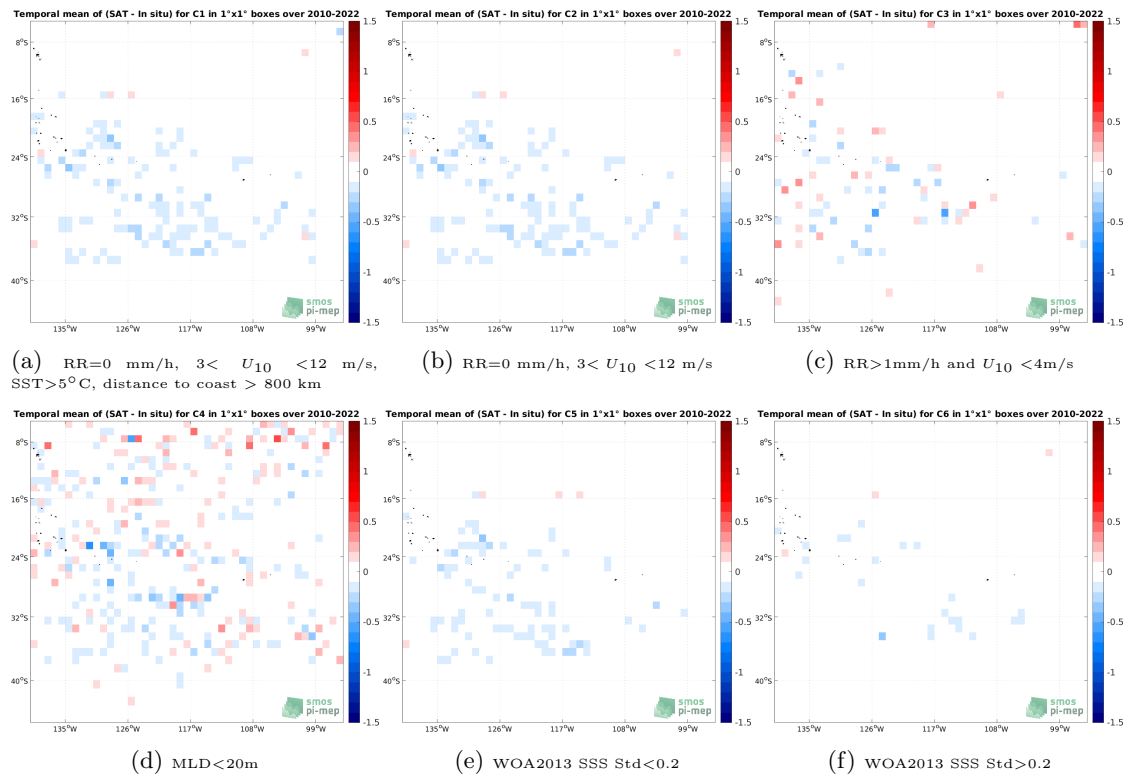
Figure 12: Temporal mean gridded over spatial boxes of size 1^\circ \times 1^\circ of \Delta SSS (SMOS SSS L4 v1 - Monthly (CMEMS-CNR) - Argo) for 6 different subdatasets corresponding to:RR=0 mm/h, 3 < U_{10} < 12 m/s, SST >5^\circ C, distance to coast > 800 km (a), RR=0 mm/h, 3 < U_{10} < 12 m/s (b), RR >1 mm/h and U_{10} < 4 m/s (c),MLD <20 m (d),WOA2013 SSS Std <0.2 (e),WOA2013 SSS Std >0.2 (f).
