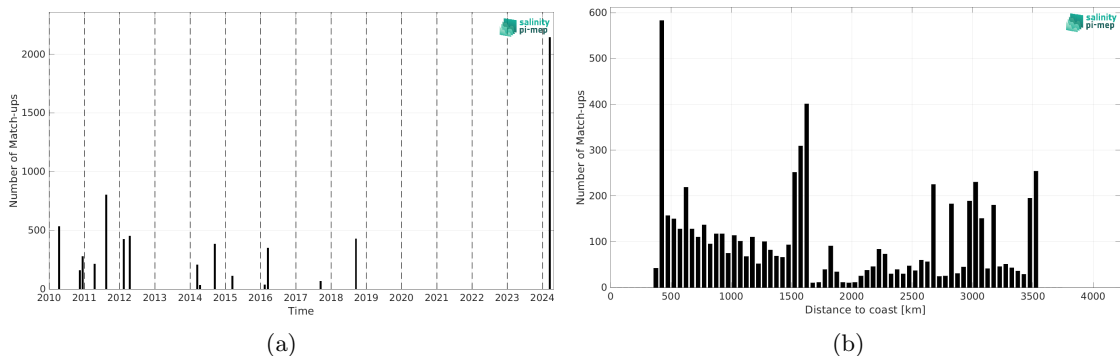
Figure 2: Number of match-ups between TSG (SAMOS) and SMOS SSS L4 v1 - Daily (CMEMS-CNR) SSS as a function of time (a) and as function of the distance to coast (b) over the OTT zone Pi-MEP region and for the full satellite product period.
