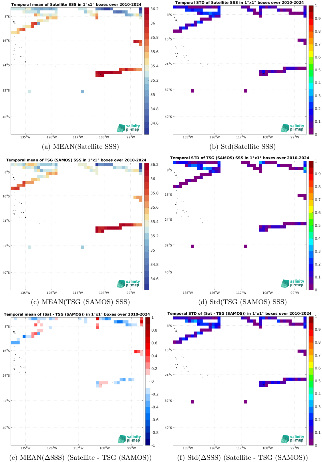
Figure 7: Temporal mean (left) and Std (right) of SSS from SMOS SSS L4 v1 - Daily (CMEMS-CNR) (top), TSG (SAMOS) (middle), and of \Delta SSS (Satellite - TSG (SAMOS)). Only match-up pairs are used to generate these maps.
