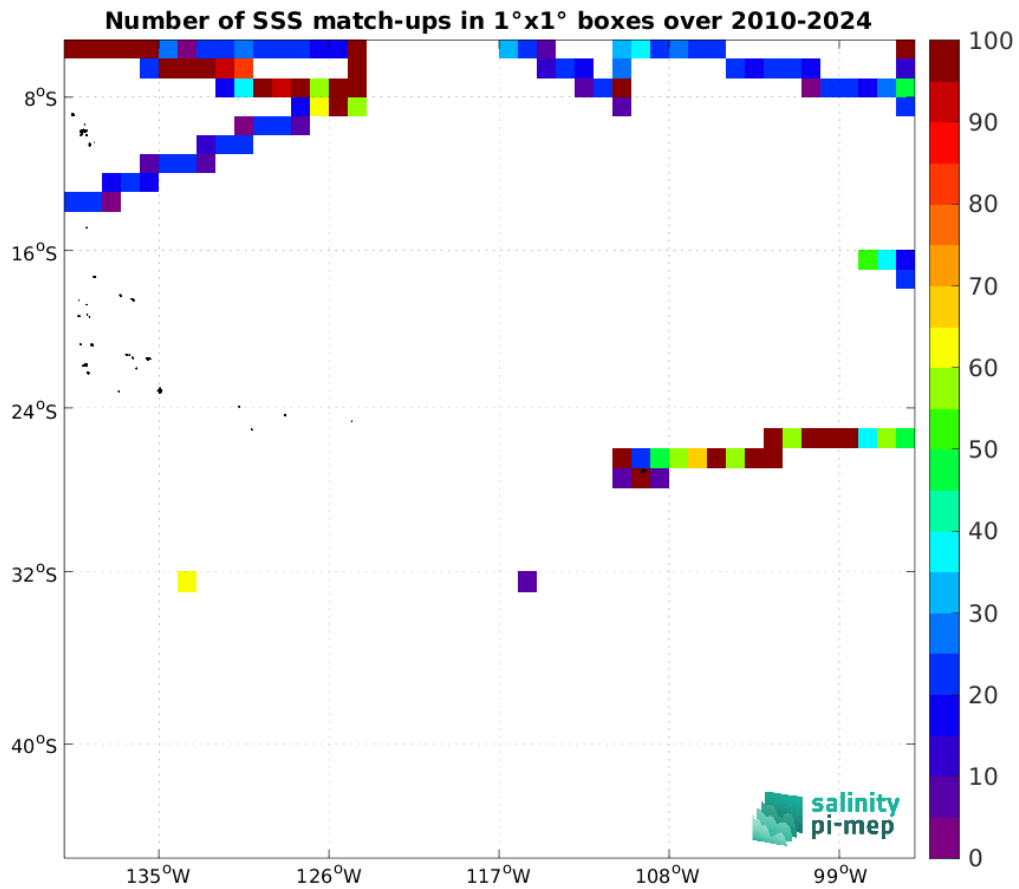
Figure 5: Number of SSS match-ups between TSG (SAMOS) SSS and the SMOS SSS L4 v1 - Daily (CMEMS-CNR) SSS product for the OTT zone Pi-MEP region over 1^\circ \times 1^\circ boxes and for the full satellite product period.
