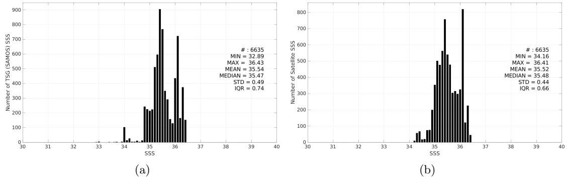
Figure 3: Histograms of SSS from TSG (SAMOS) (a) and SMOS SSS L4 v1 - Daily (CMEMS-CNR) (b) considering all match-up pairs per bins of 0.1 over the OTT zone Pi-MEP region and for the full satellite product period.
